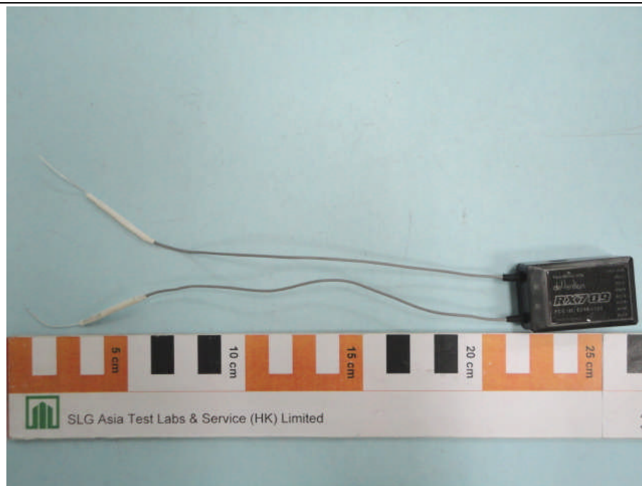
Picture 11: RX709 (2.4GHz DSSS Transceiver module)
