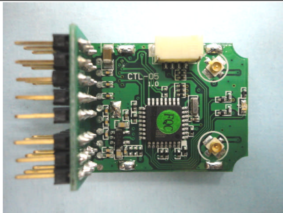
Picture 12: RX709 (2.4GHz DSSS Transceiver module)
