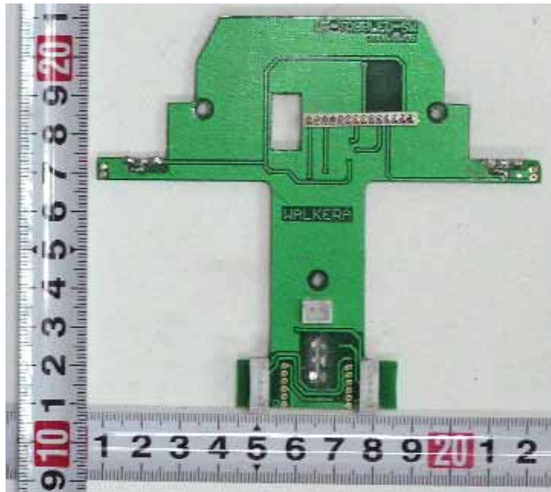
EUT –PCB 2 View (One Side)
