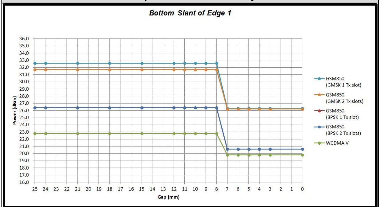
Proximity Sensor for Bottom Slant of Edge 1
