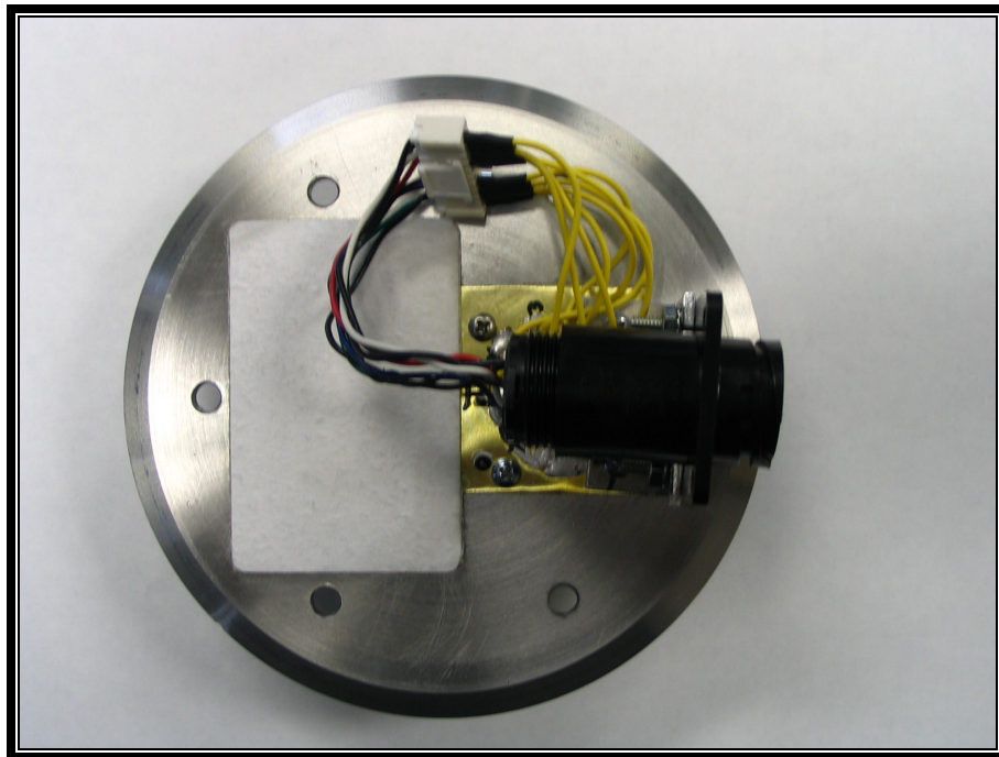
PHOTOGRAPH 17: RX TOP VIEW
