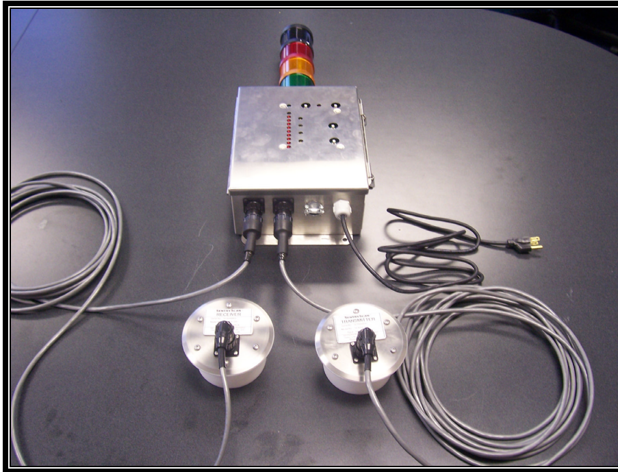
PHOTOGRAPH 8: EUT COMPONENTS - CONTROL BOX WITH TRANSMITTER AND RECEIVER
