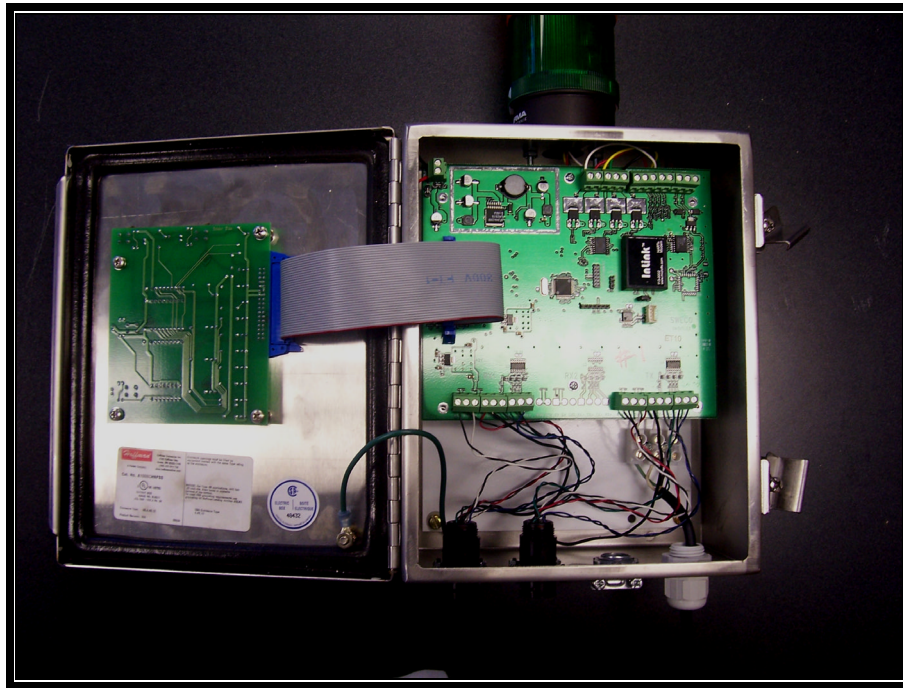
PHOTOGRAPH 22: CONTROL BOX INSIDE VIEW - PCB
