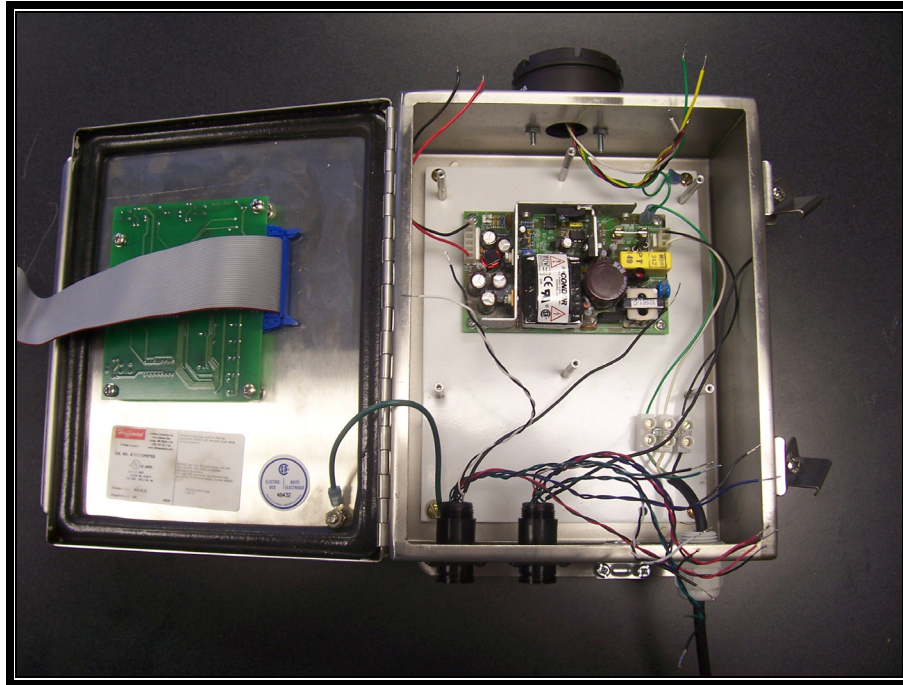
PHOTOGRAPH 20: CONTROL BOX INSIDE VIEW - BOTH SIDES
