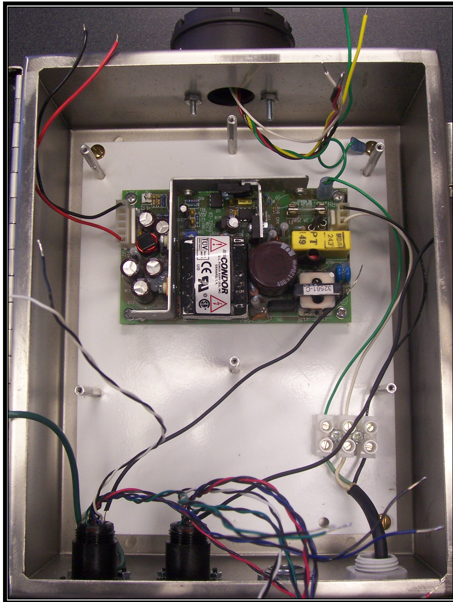
PHOTOGRAPH 21: CONTROL BOX INSIDE VIEW – RIGHT SIDE
