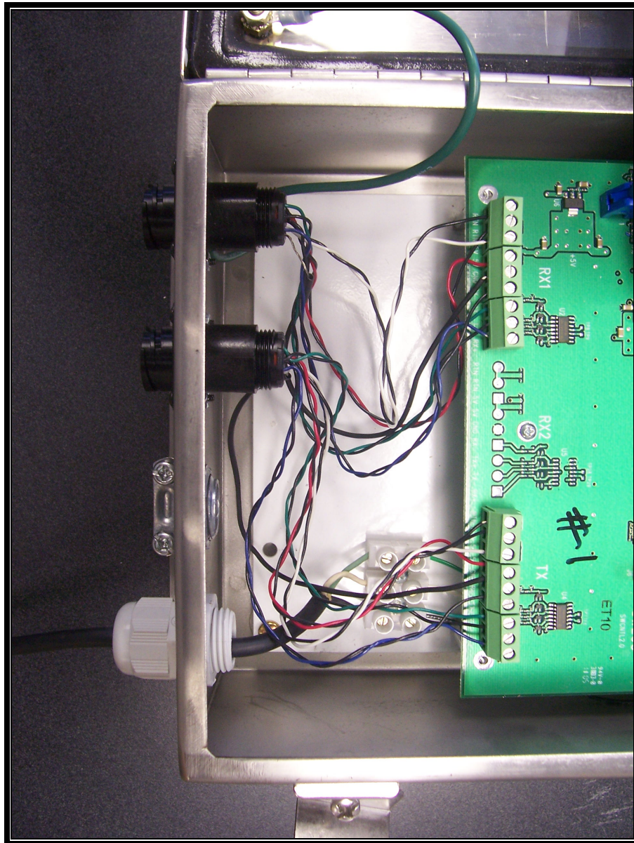
PHOTOGRAPH 24: CONTROL BOX INSIDE VIEW
