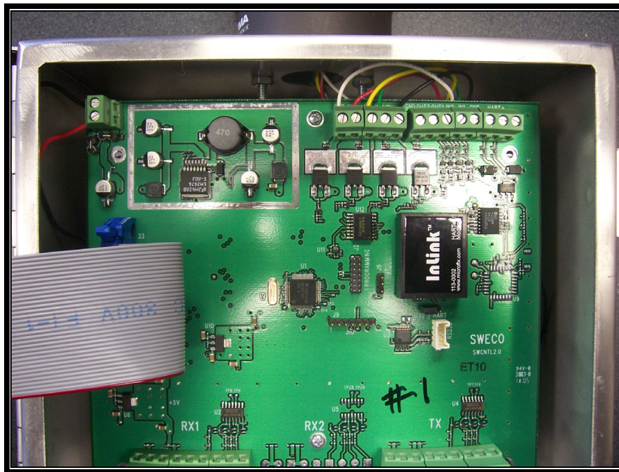
PHOTOGRAPH 23: CONTROL BOX INSIDE VIEW – PCB CLOSER VIEW
