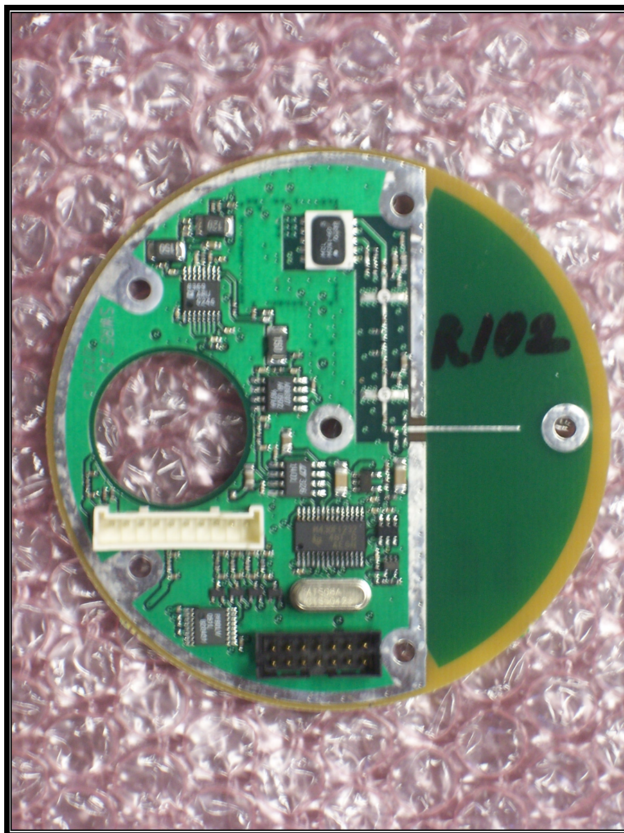
PHOTOGRAPH 30: RX BOARD FRONT VIEW
