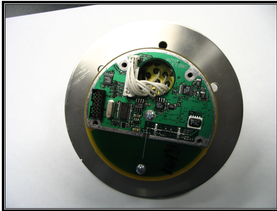
PHOTOGRAPH 29: RX BOARD IN PLACE
