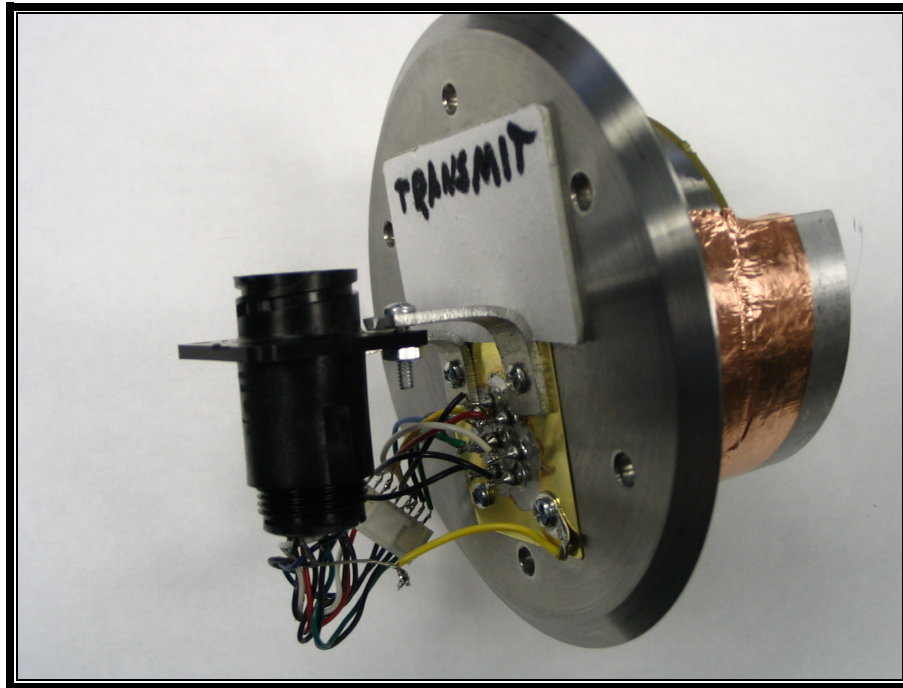
PHOTOGRAPH 32: TX TOP AND SIDE VIEW
