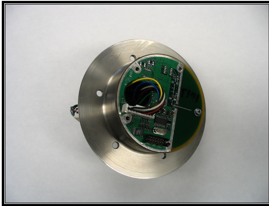
PHOTOGRAPH 36: TX BOARD IN PLACE
