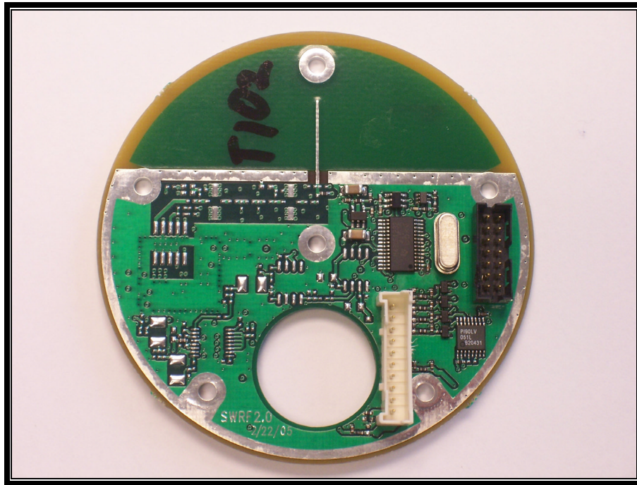
PHOTOGRAPH 37: TX BOARD FRONT VIEW
