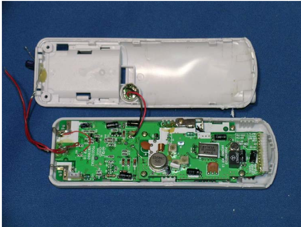
Handset assembly
