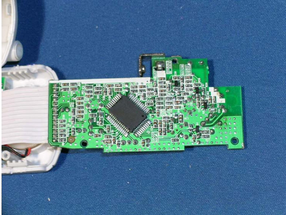
Handset Main PCB display comp side
