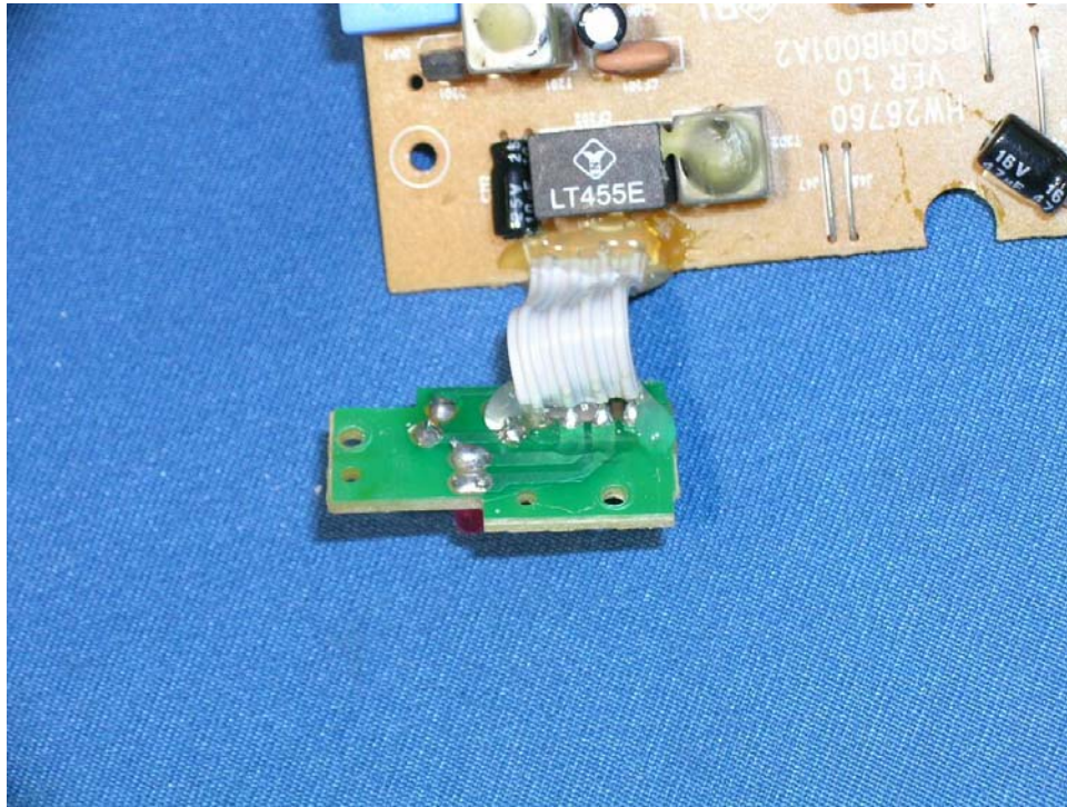
Base LED rear side
