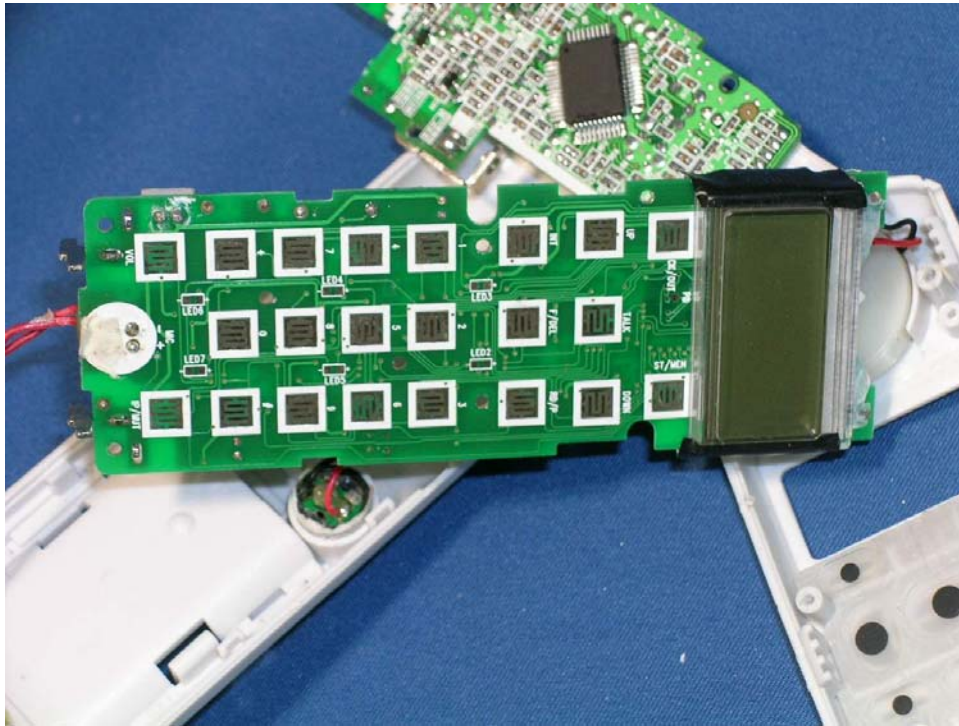
Handset Main PCB display solder side
