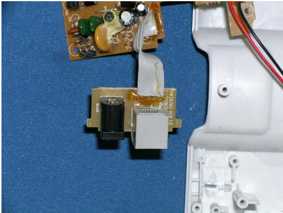
Base Telephone Line Jack front side
