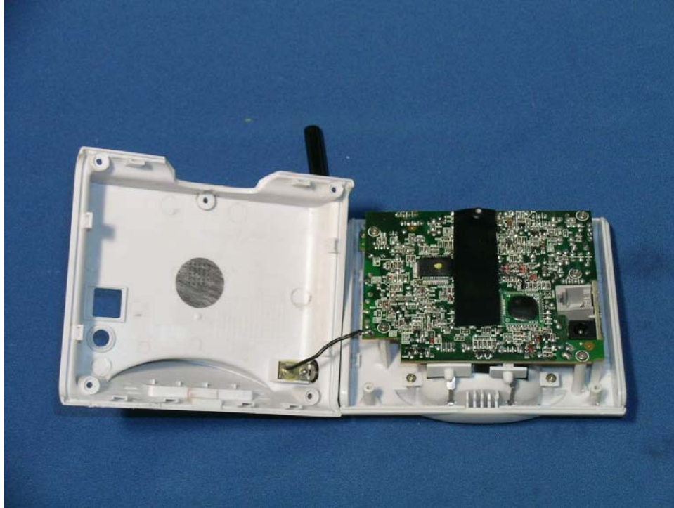
Base assembly
