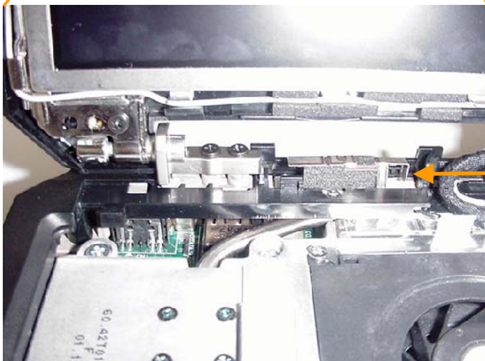
Auxiliary antenna Inverted-F type P/N: 46L6324
