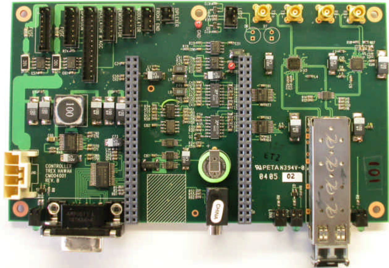
Photo of Control board – Top view with Netburner board removed
