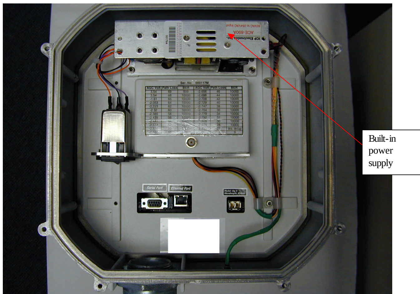
Photo of EUT showing service compartment with rear cover removed
