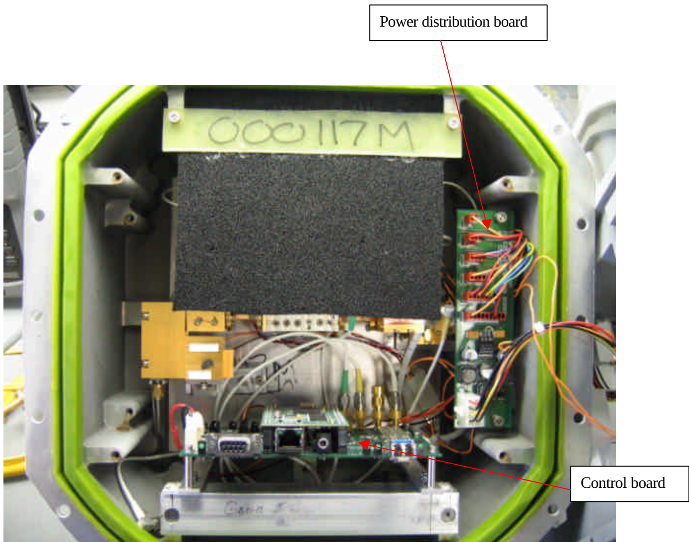
Internal photo of EUT with service compartment removed from main housing
