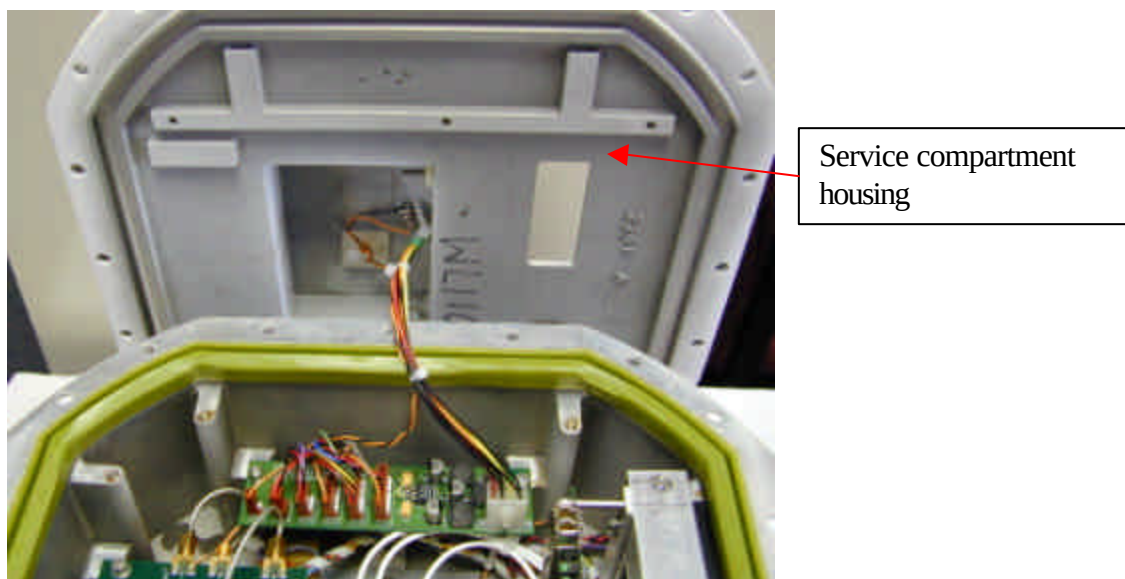
Photo of EUT showing backside of service compartment housing
