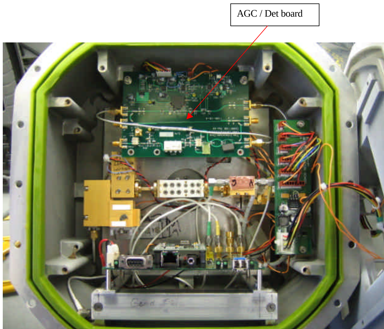
Internal photo of EUT with absorber material removed
