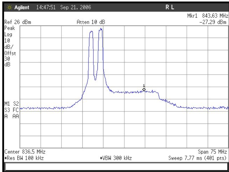
Uplink Low End Intermod (CDMA)
