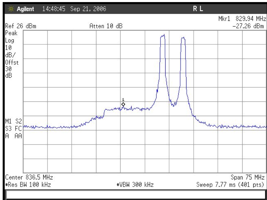
Uplink High End Intermod (CDMA)
