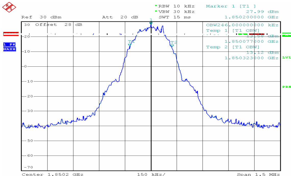
Figure 7-1: PCS Channel Low
