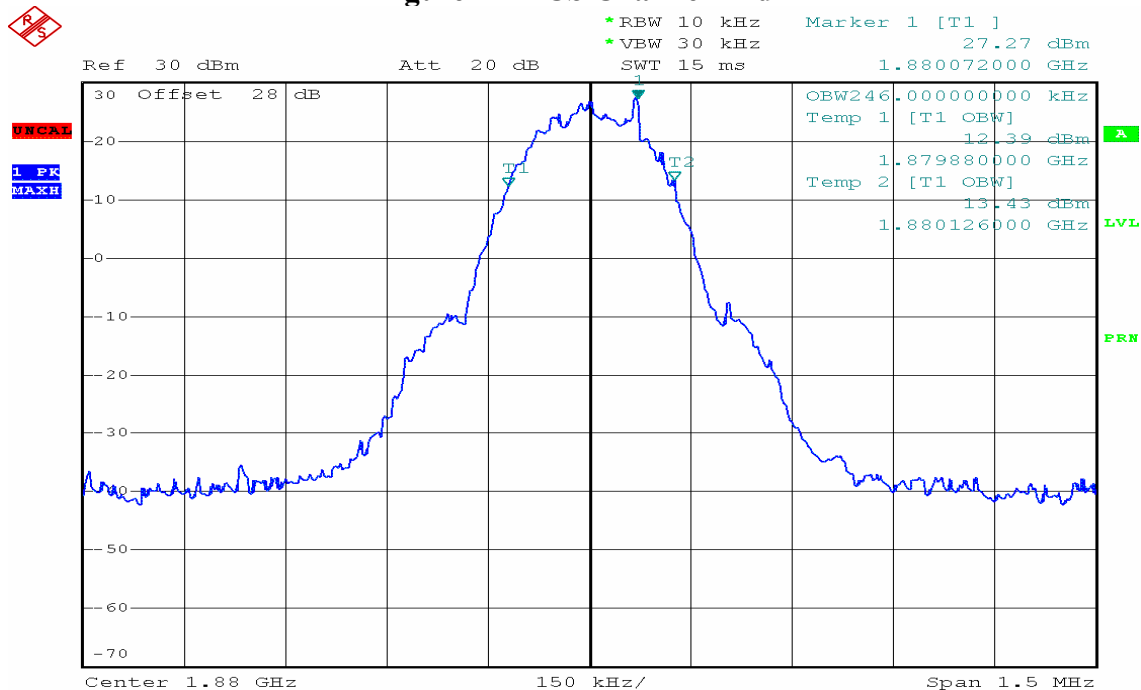
Figure 7-2 PCS Channel Mid
