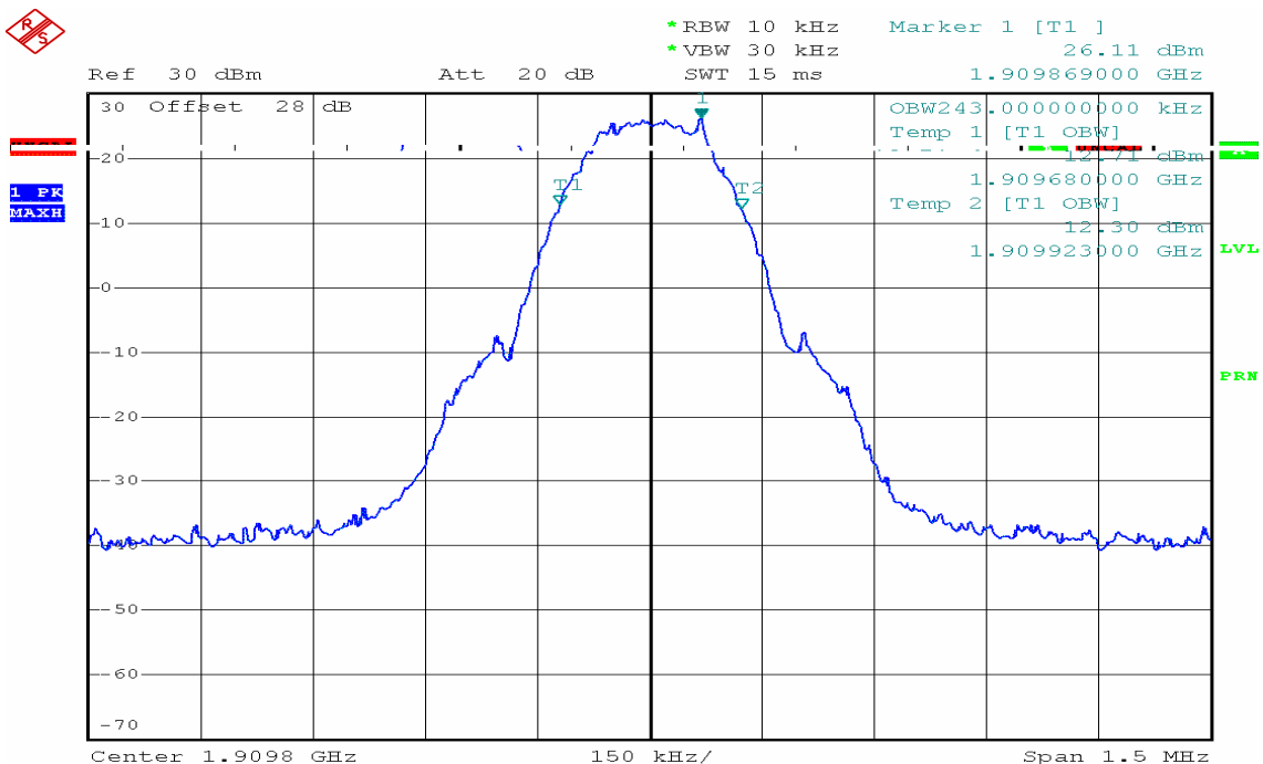
Figure 7-3: PCS Channel High
