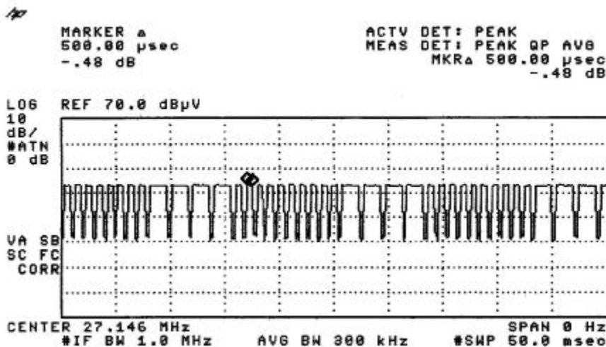
Figure C [Short Pulse]
