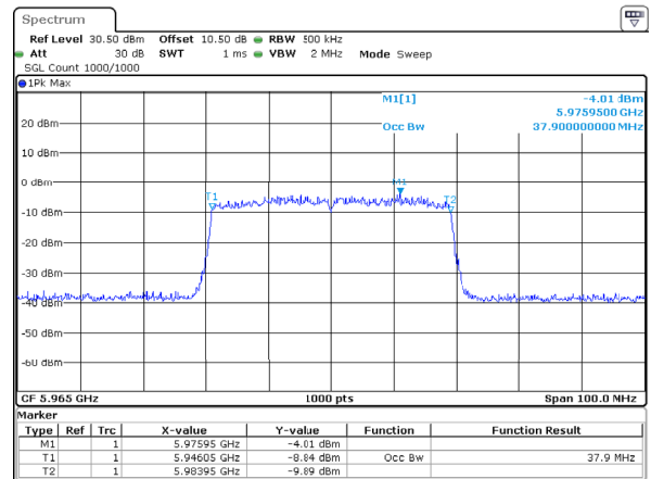
802.11ax40_5965MHz_RU_Full_ANT2 37.900MHz
