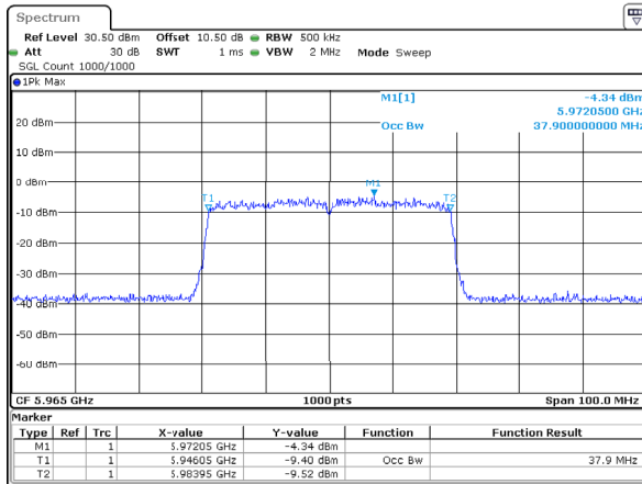
802.11ax40_5965MHz_RU_Full_ANT1 37.900MHz
