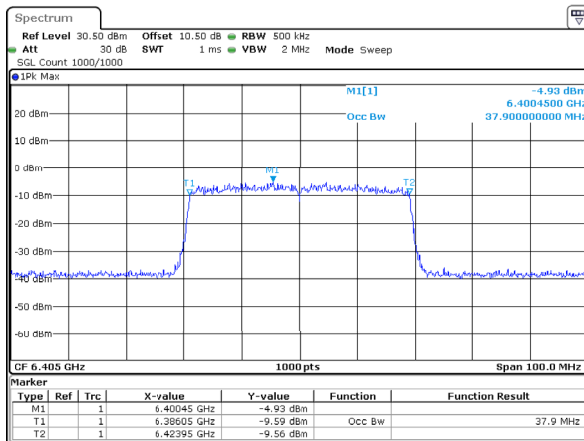
802.11ax40_6405MHz_RU_Full_ANT1 37.900MHz
