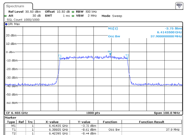
802.11ax40_6405MHz_RU_Full_ANT2 37.900MHz
