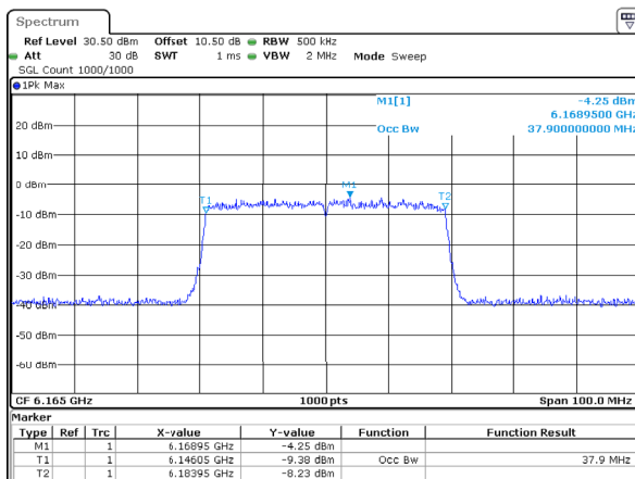
802.11ax40_6165MHz_RU_Full_ANT2 37.900MHz
