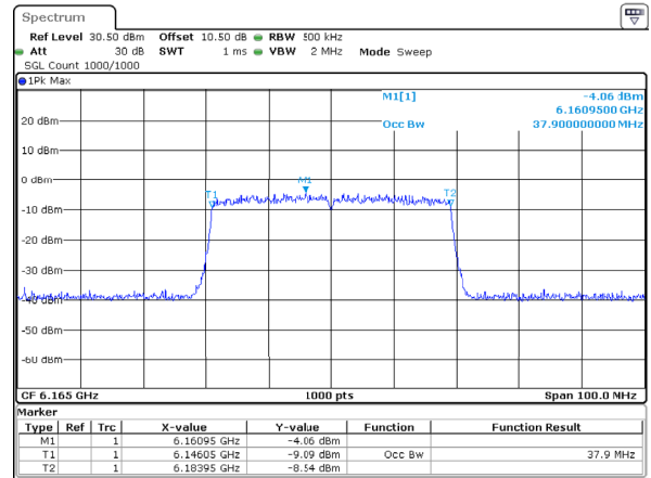
802.11ax40_6165MHz_RU_Full_ANT1 37.900MHz
