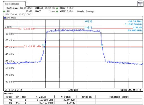
802.11ax80_6145MHz_RU_Full_ANT1 83.483MHz
