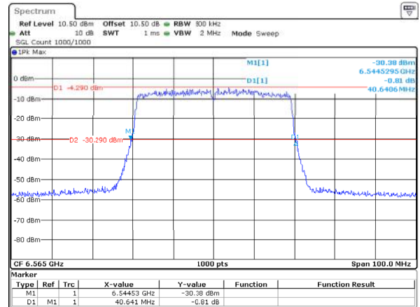
802.11ax40_6565MHz_RU_Full_ANT2 40.641MHz
