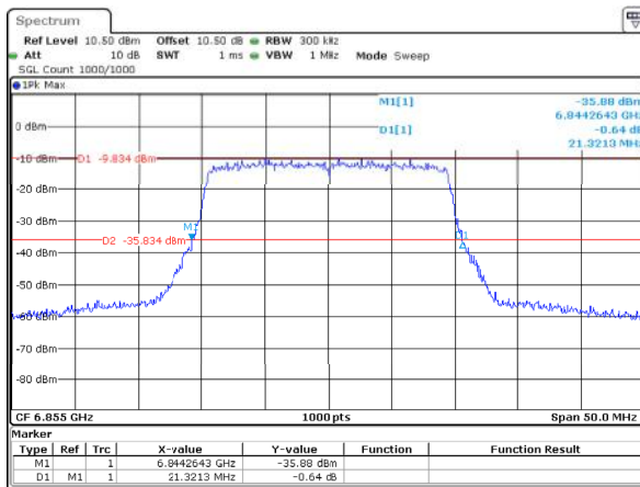
802.11ax20_6855MHz_RU_Full_ANT1 21.321MHz
