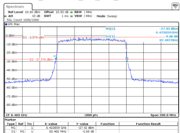
802.11ax80_6465MHz_RU_Full_ANT2 82.482MHz
