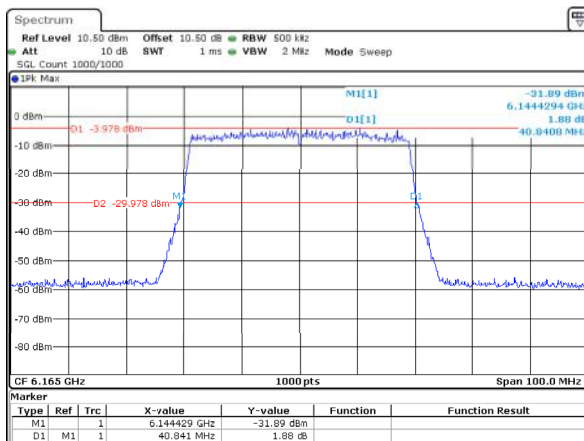
802.11ax40_6165MHz_RU_Full_ANT2 40.841MHz
