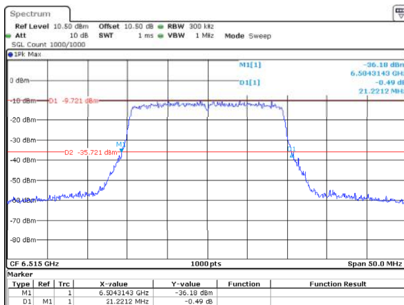
802.11ax20_6515MHz_RU_Full_ANT1 21.221MHz
