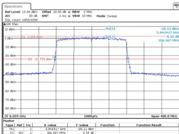
802.11ax160_6025MHz_RU_Full_ANT1 166.567MHz
