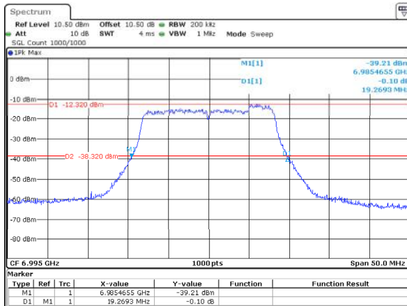
802.11a_6995MHz_ANT1 19.269MHz
