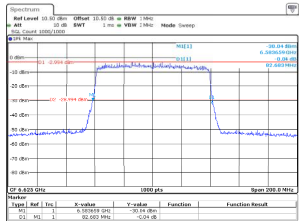
802.11ax80_6625MHz_RU_Full_ANT2 82.683MHz
