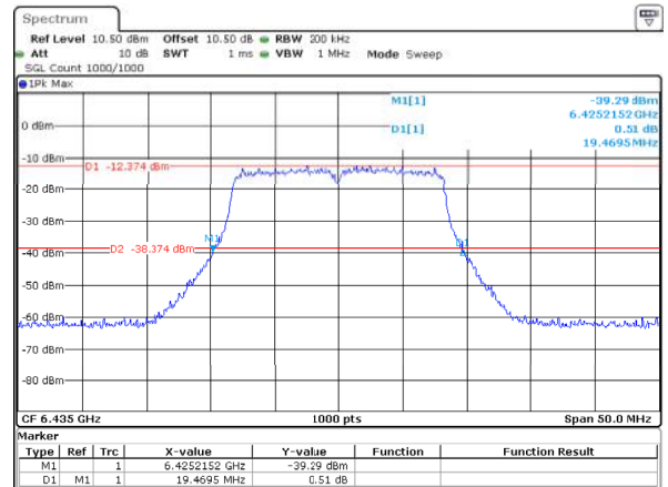
802.11a_6435MHz_ANT2 19.469MHz
