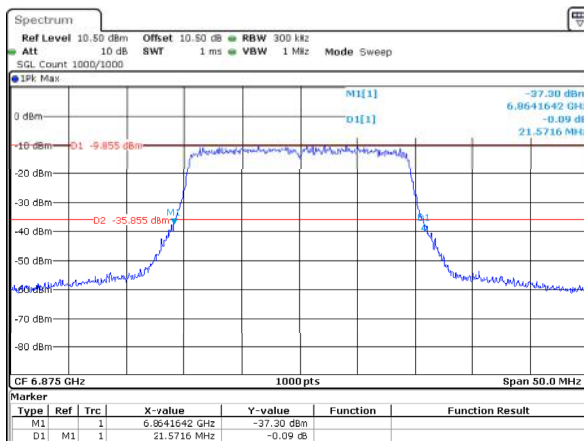
802.11ax20_6875MHz_RU_Full_ANT1 21.572MHz
