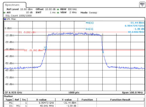
802.11ax40_6925MHz_RU_Full_ANT2 40.641MHz
