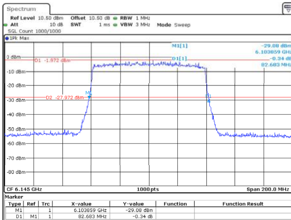
802.11ax80_6145MHz_RU_Full_ANT2 82.683MHz
