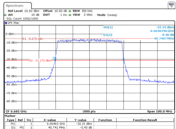
802.11ax40_6685MHz_RU_Full_ANT1 40.741MHz
