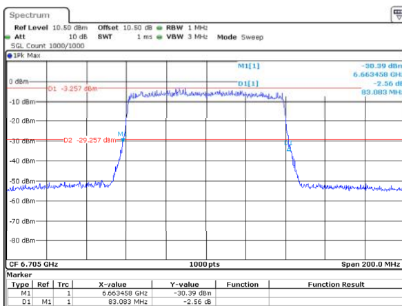
802.11ax80_6705MHz_RU_Full_ANT2 83.083MHz
