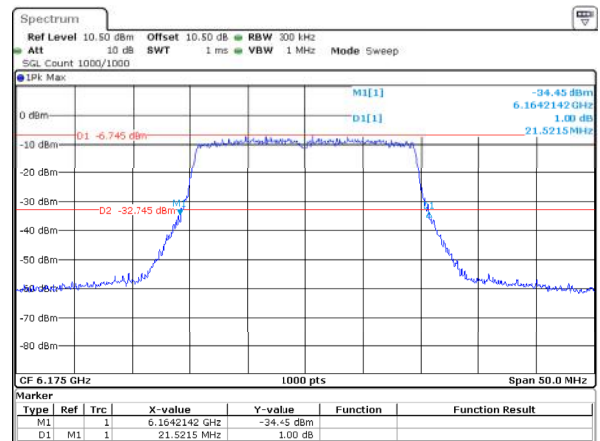
802.11ax20_6175MHz_RU_Full_ANT1 21.522MHz
