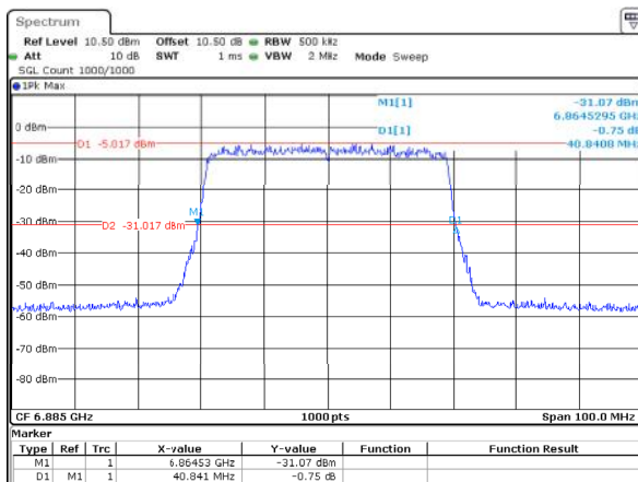
802.11ax40_6885MHz_RU_Full_ANT2 40.841MHz
