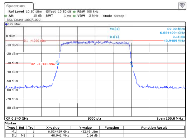
802.11ax40_6845MHz_RU_Full_ANT2 40.941MHz
