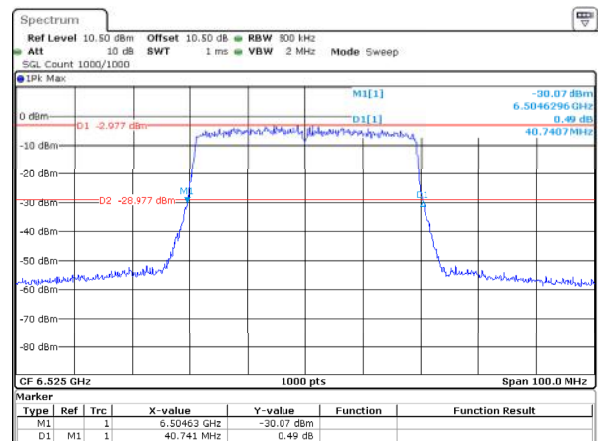
802.11ax40_6525MHz_RU_Full_ANT2 40.741MHz
