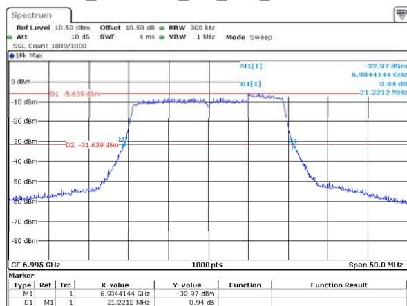
802.11ax20_6995MHz_RU_Full_ANT2 21.221MHz
