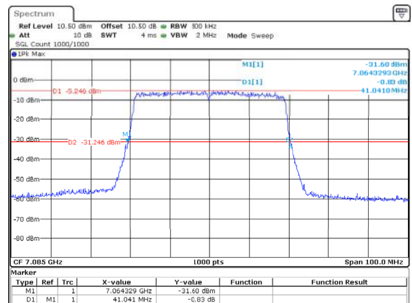
802.11ax40_7085MHz_RU_Full_ANT1 41.041MHz
