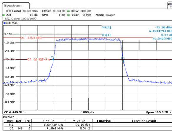
802.11ax40_6445MHz_RU_Full_ANT2 41.041MHz
