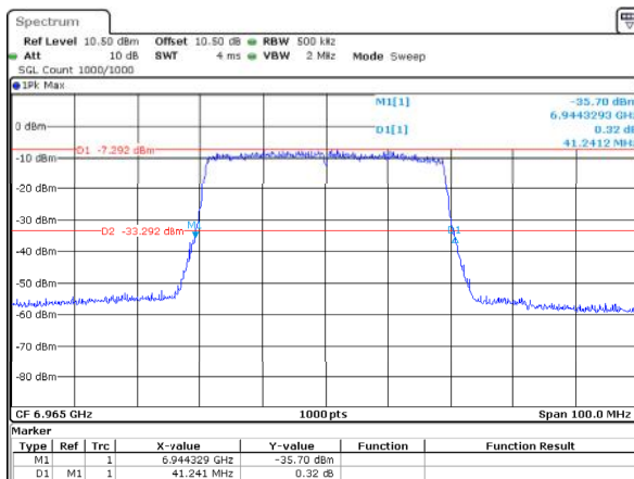
802.11ax40_6965MHz_RU_Full_ANT1 41.241MHz
