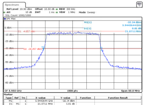
802.11ax20_5955MHz_RU_Full_ANT2 21.071MHz
