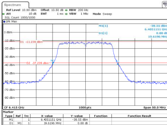
802.11a_6415MHz_ANT1 19.620MHz
