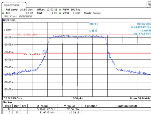
802.11ax20_5955MHz_RU_Full_ANT1 21.471MHz
