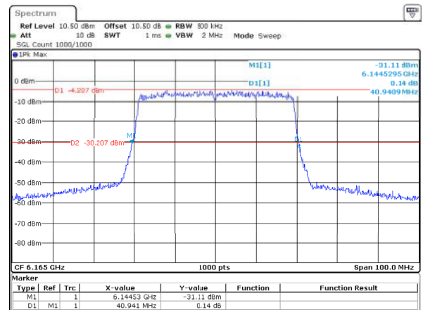
802.11ax40_6165MHz_RU_Full_ANT1 40.941MHz
