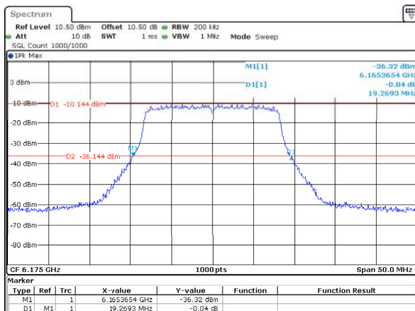
802.11a_6175MHz_ANT2 19.269MHz
