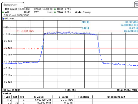
802.11ax80_6945MHz_RU_Full_ANT1 82.683MHz
