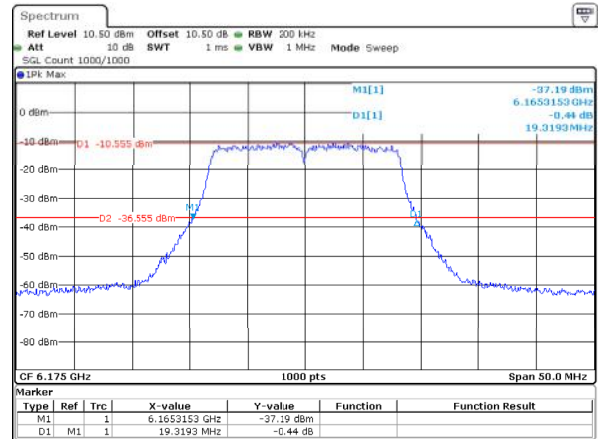
802.11a_6175MHz_ANT1 19.319MHz
