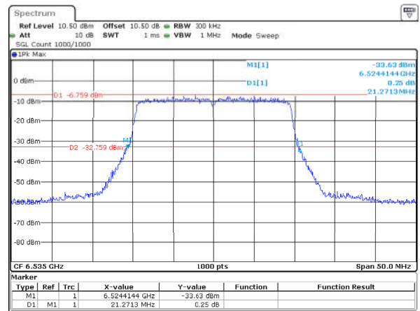
802.11ax20_6535MHz_RU_Full_ANT2 21.271MHz
