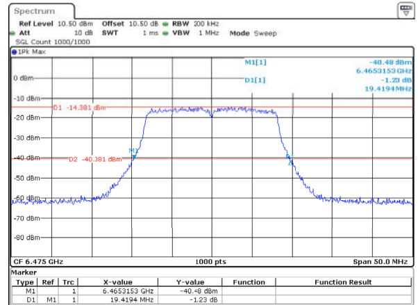
802.11a_6475MHz_ANT1 19.419MHz
