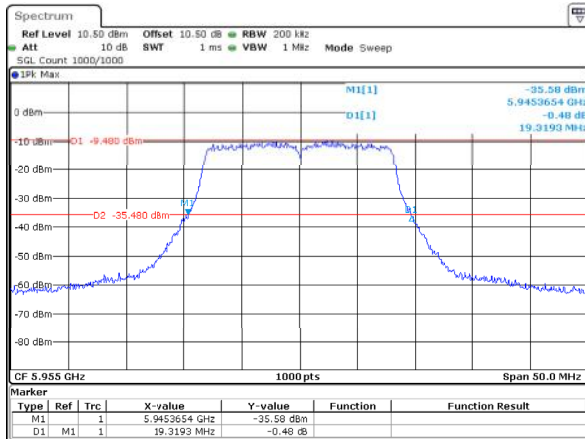
802.11a_5955MHz_ANT1 19.319MHz
