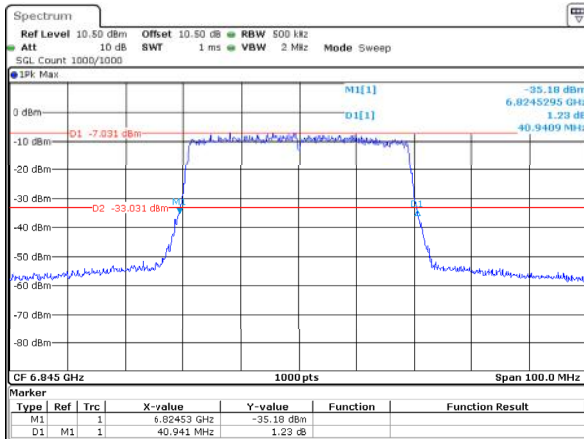
802.11ax40_6845MHz_RU_Full_ANT1 40.941MHz
