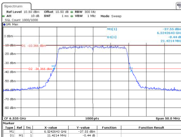
802.11ax20_6535MHz_RU_Full_ANT1 21.421MHz
