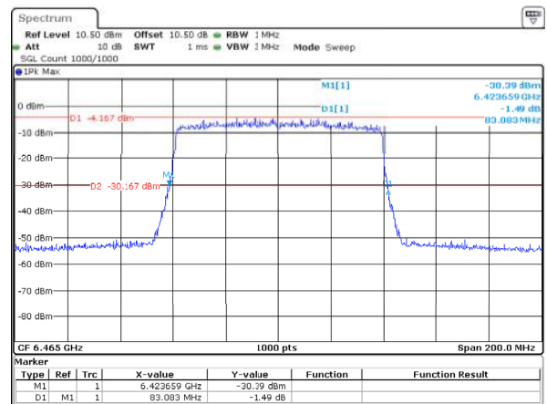
802.11ax80_6465MHz_RU_Full_ANT1 83.083MHz
