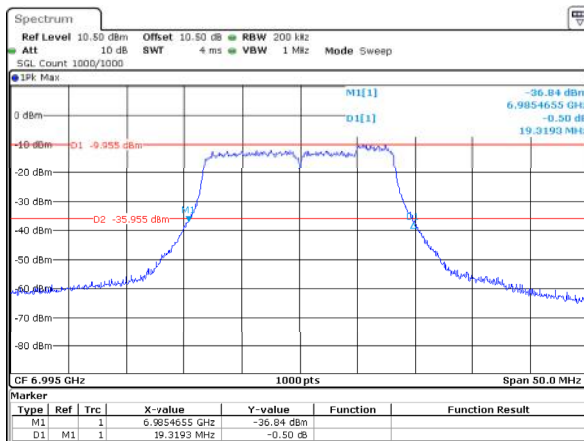
802.11a_6995MHz_ANT2 19.319MHz
