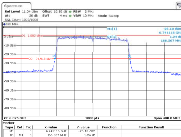
802.11ax160_6825MHz_RU_Full_ANT1 166.567MHz
