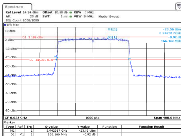
802.11ax160_6025MHz_RU_Full_ANT2 166.166MHz
