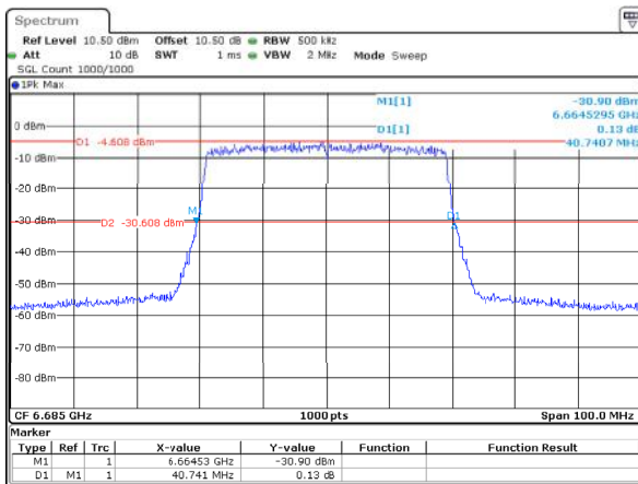
802.11ax40_6685MHz_RU_Full_ANT2 40.741MHz
