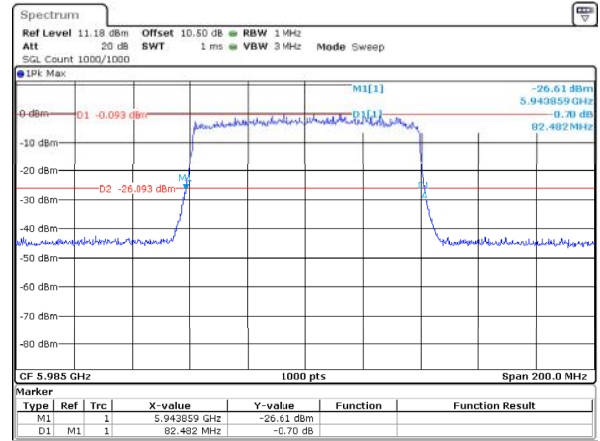
802.11ax80_5985MHz_RU_Full_ANT2 82.482MHz
