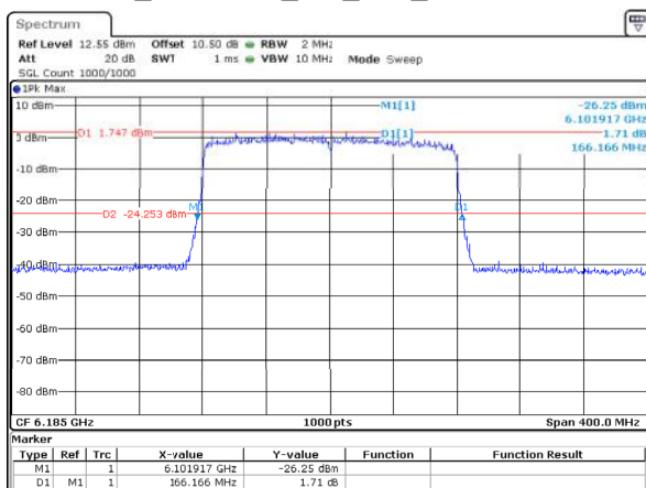
802.11ax160_6185MHz_RU_Full_ANT2 166.166MHz
