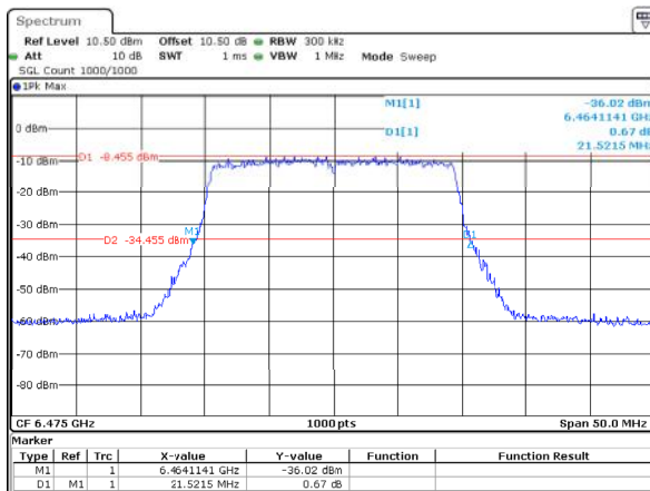
802.11ax20_6475MHz_RU_Full_ANT2 21.522MHz
