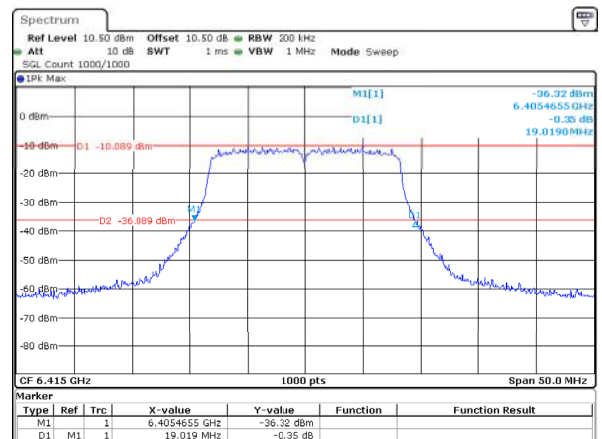
802.11a_6415MHz_ANT2 19.019MHz
