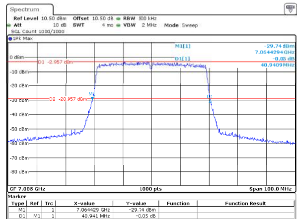
802.11ax40_7085MHz_RU_Full_ANT2 40.941MHz
