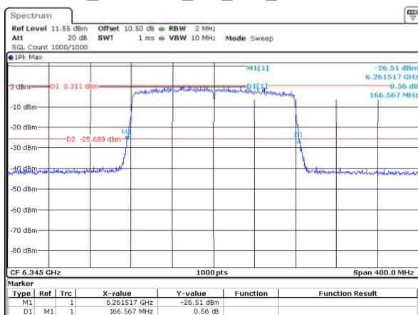
802.11ax160_6345MHz_RU_Full_ANT1 166.567MHz
