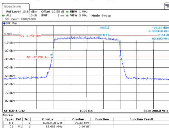
802.11ax80_6545MHz_RU_Full_ANT2 82.683MHz
