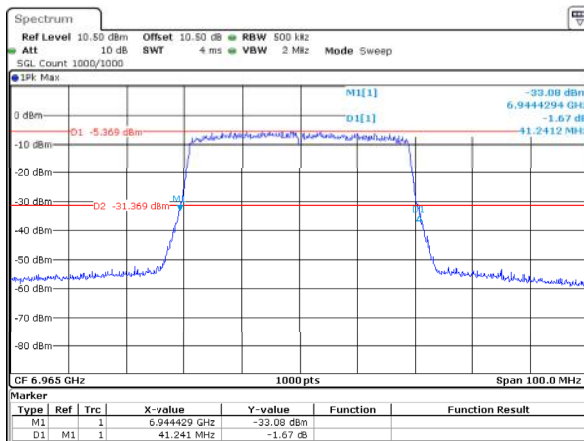
802.11ax40_6965MHz_RU_Full_ANT2 41.241MHz
