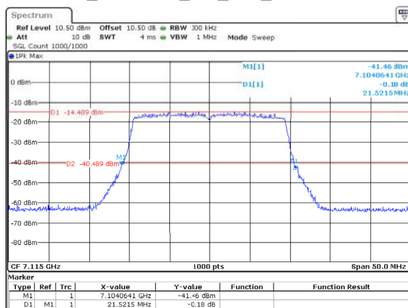
802.11ax20_7115MHz_RU_Full_ANT2 21.522MHz
