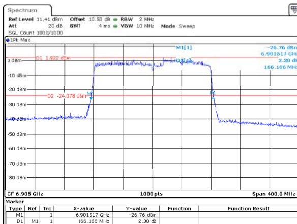
802.11ax160_6985MHz_RU_Full_ANT1 166.166MHz
