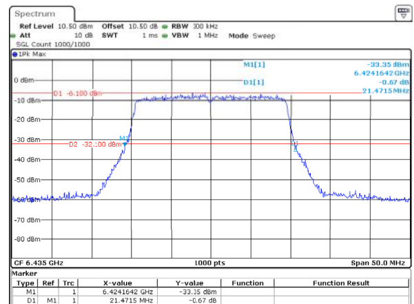
802.11ax20_6435MHz_RU_Full_ANT2 21.471MHz
