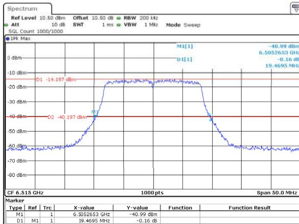
802.11a_6515MHz_ANT1 19.469MHz
