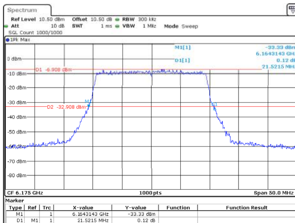
802.11ax20_6175MHz_RU_Full_ANT2 21.522MHz
