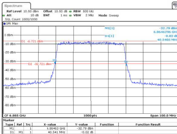
802.11ax40_6885MHz_RU_Full_ANT1 40.541MHz
