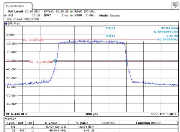
802.11ax40_6445MHz_RU_Full_ANT1 40.941MHz
