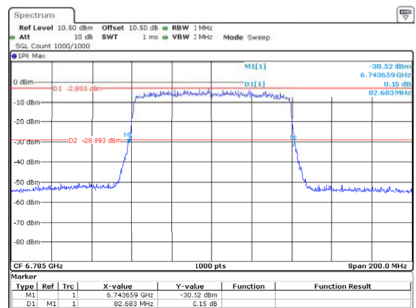
802.11ax80_6785MHz_RU_Full_ANT2 82.683MHz
