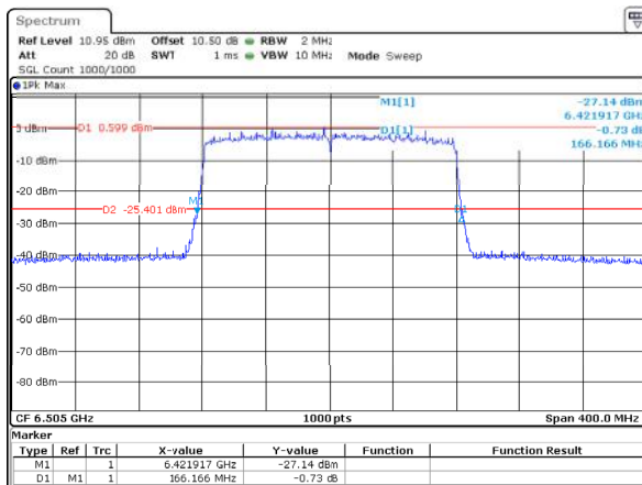
802.11ax160_6505MHz_RU_Full_ANT1 166.166MHz
