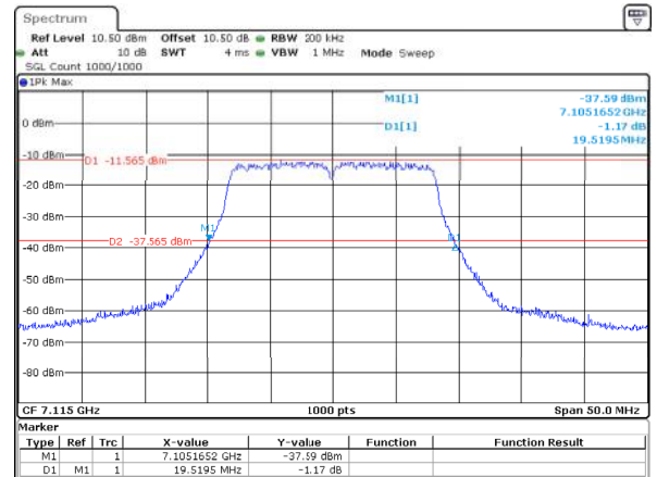
802.11a_7115MHz_ANT1 19.520MHz
