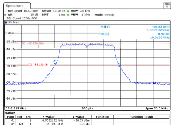
802.11a_6515MHz_ANT2 19.319MHz
