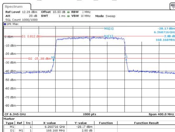
802.11ax160_6345MHz_RU_Full_ANT2 168.168MHz
