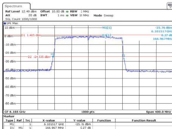
802.11ax160_6185MHz_RU_Full_ANT1 166.967MHz
