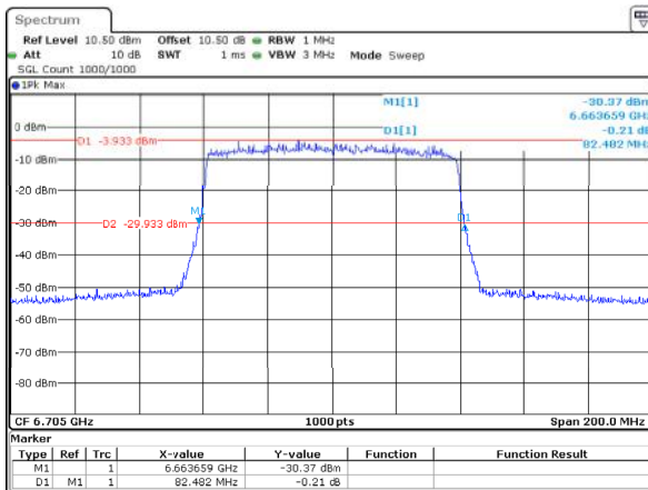
802.11ax80_6705MHz_RU_Full_ANT1 82.482MHz
