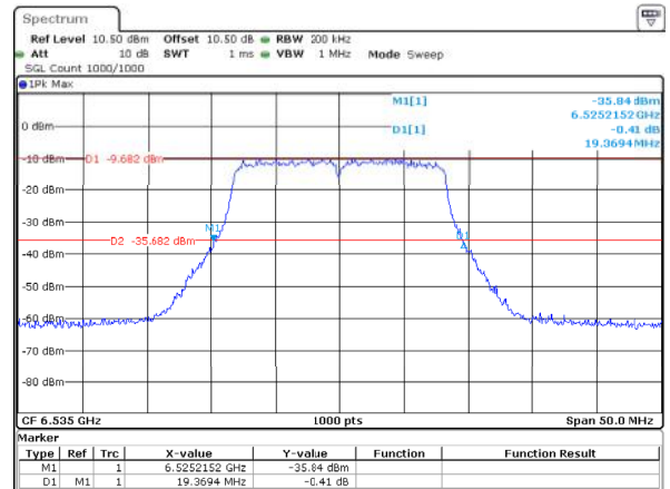
802.11a_6535MHz_ANT2 19.369MHz
