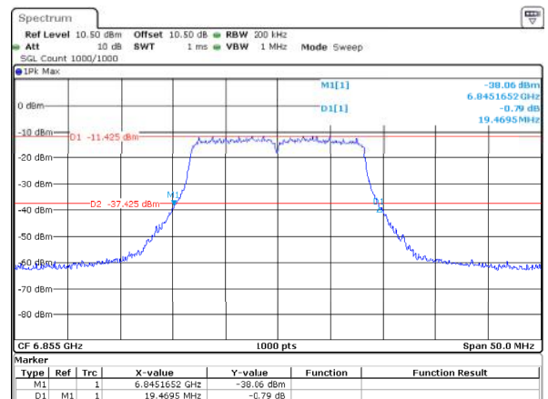
802.11a_6855MHz_ANT2 19.469MHz
