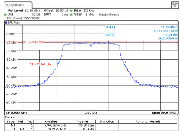
802.11a_5955MHz_ANT2 19.219MHz
