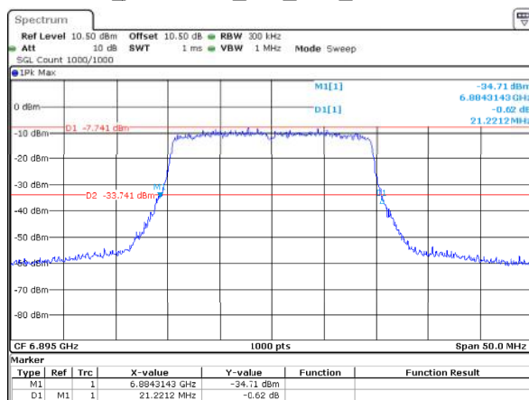
802.11ax20_6895MHz_RU_Full_ANT2 21.221MHz
