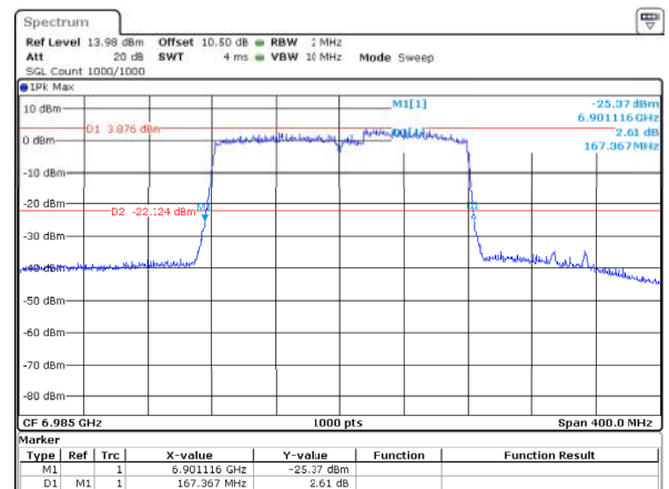
802.11ax160_6985MHz_RU_Full_ANT2 167.367MHz
