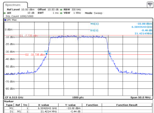
802.11ax20_6515MHz_RU_Full_ANT2 21.421MHz
