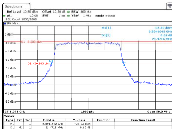
802.11ax20_6875MHz_RU_Full_ANT2 21.471MHz
