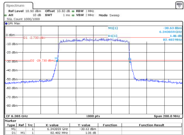
802.11ax80_6385MHz_RU_Full_ANT2 82.482MHz
