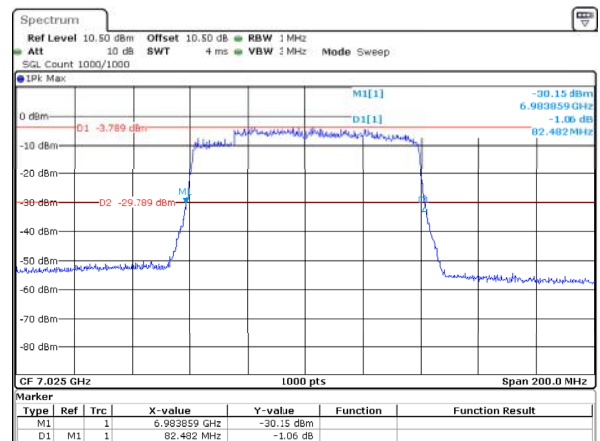
802.11ax80_7025MHz_RU_Full_ANT1 82.482MHz
