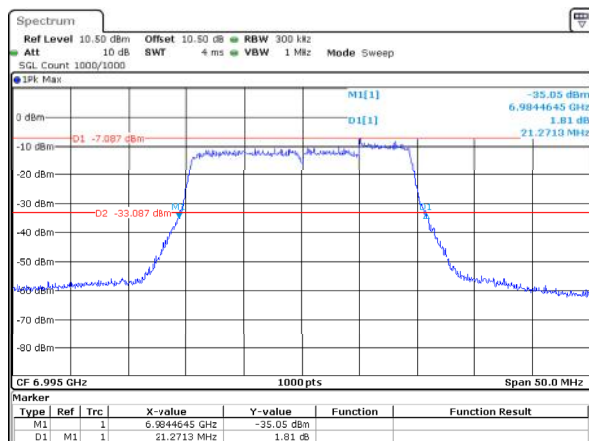
802.11ax20_6995MHz_RU_Full_ANT1 21.271MHz
