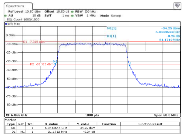
802.11ax20_6855MHz_RU_Full_ANT2 21.171MHz
