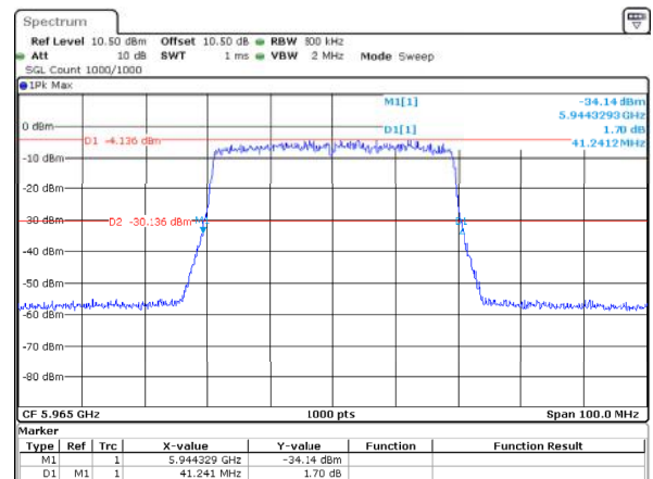
802.11ax40_5965MHz_RU_Full_ANT2 41.241MHz
