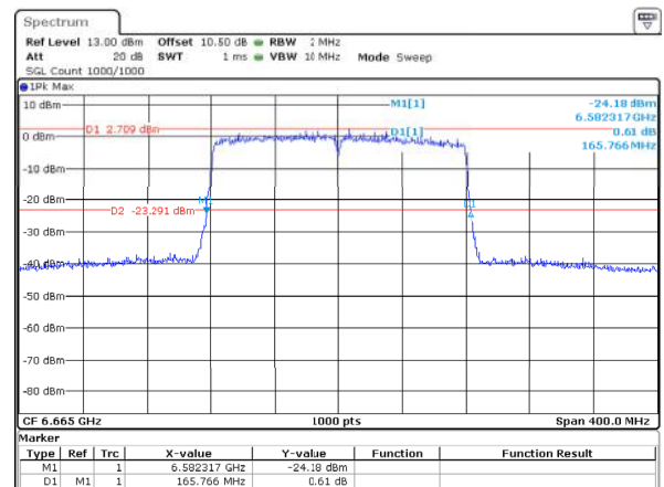
802.11ax160_6665MHz_RU_Full_ANT2 165.766MHz
