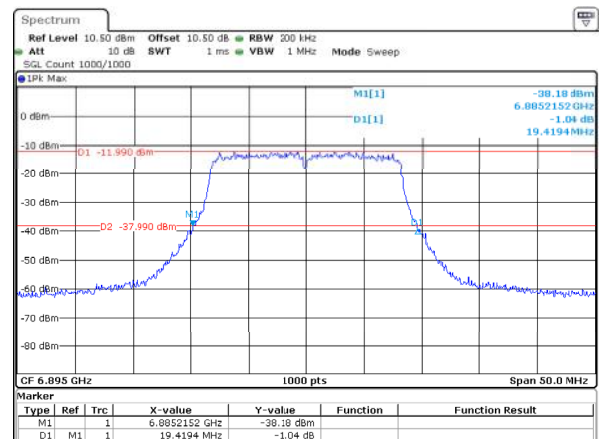
802.11a_6895MHz_ANT2 19.419MHz
