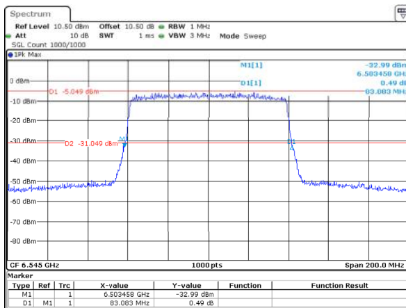
802.11ax80_6545MHz_RU_Full_ANT1 83.083MHz
