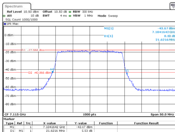
802.11ax20_7115MHz_RU_Full_ANT1 21.622MHz
