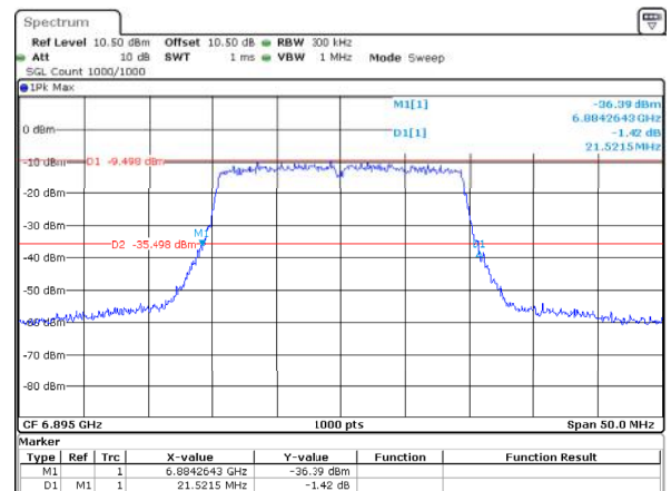
802.11ax20_6895MHz_RU_Full_ANT1 21.522MHz
