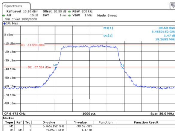
802.11a_6475MHz_ANT2 19.269MHz
