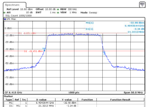
802.11ax20_6415MHz_RU_Full_ANT2 21.321MHz
