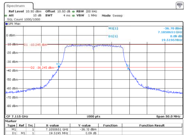
802.11a_7115MHz_ANT2 19.520MHz
