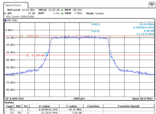
802.11ax20_6695MHz_RU_Full_ANT1 21.522MHz
