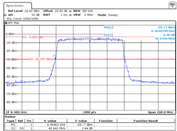
802.11ax40_6485MHz_RU_Full_ANT2 40.641MHz
