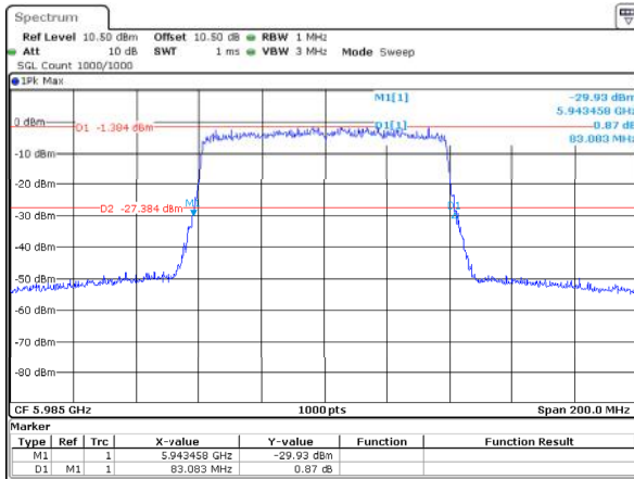
802.11ax80_5985MHz_RU_Full_ANT1 83.083MHz
