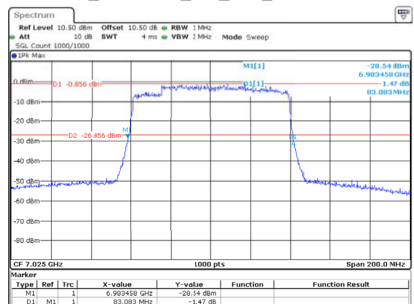
802.11ax80_7025MHz_RU_Full_ANT2 83.083MHz
