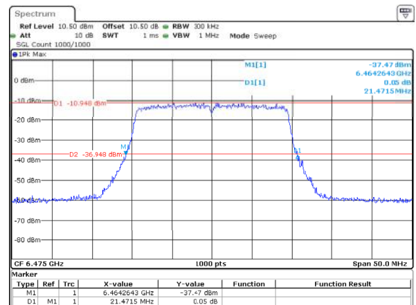
802.11ax20_6475MHz_RU_Full_ANT1 21.471MHz
