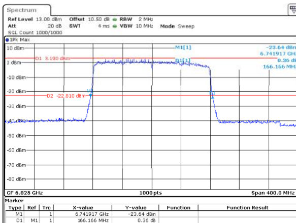
802.11ax160_6825MHz_RU_Full_ANT2 166.166MHz
