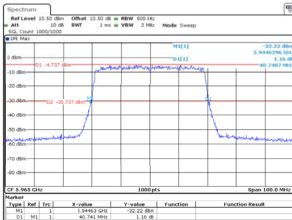
802.11ax40_5965MHz_RU_Full_ANT1 40.741MHz
