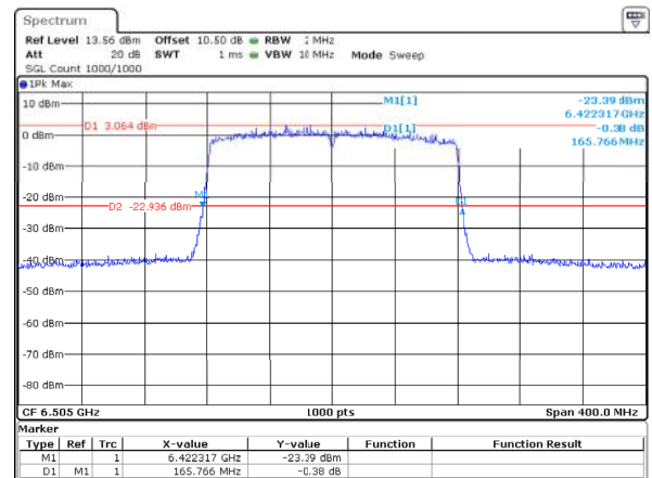
802.11ax160_6505MHz_RU_Full_ANT2 165.766MHz
