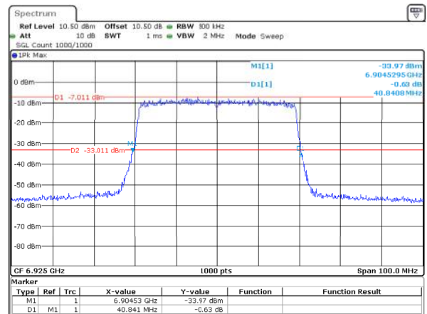
802.11ax40_6925MHz_RU_Full_ANT1 40.841MHz
