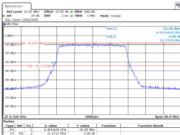
802.11ax20_6435MHz_RU_Full_ANT1 21.271MHz
