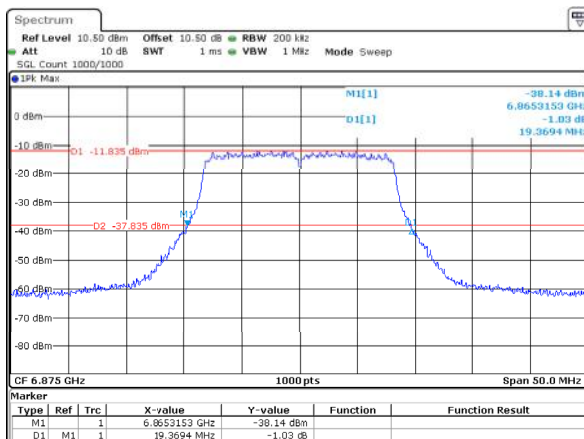
802.11a_6875MHz_ANT2 19.369MHz
