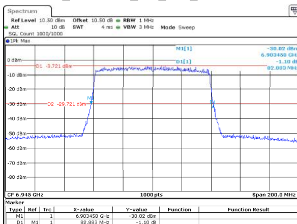
802.11ax80_6945MHz_RU_Full_ANT2 82.883MHz
