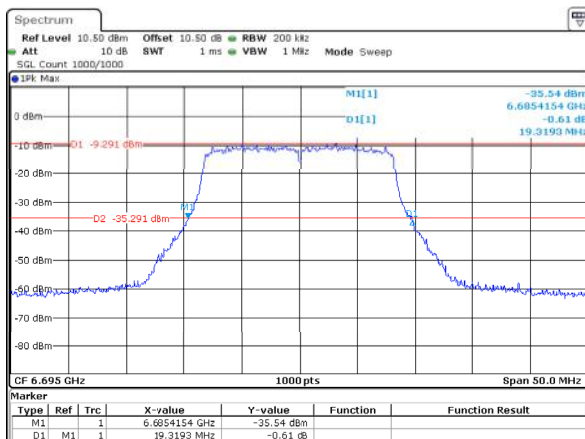
802.11a_6695MHz_ANT2 19.319MHz
