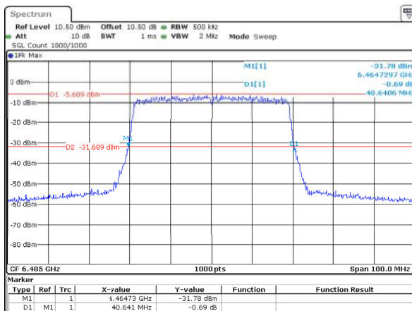
802.11ax40_6485MHz_RU_Full_ANT1 40.641MHz
