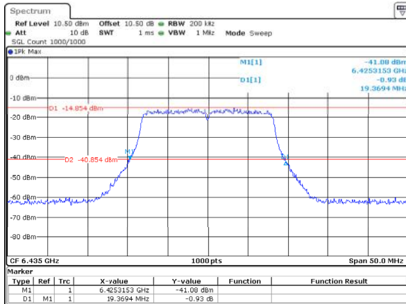
802.11a_6435MHz_ANT1 19.369MHz
