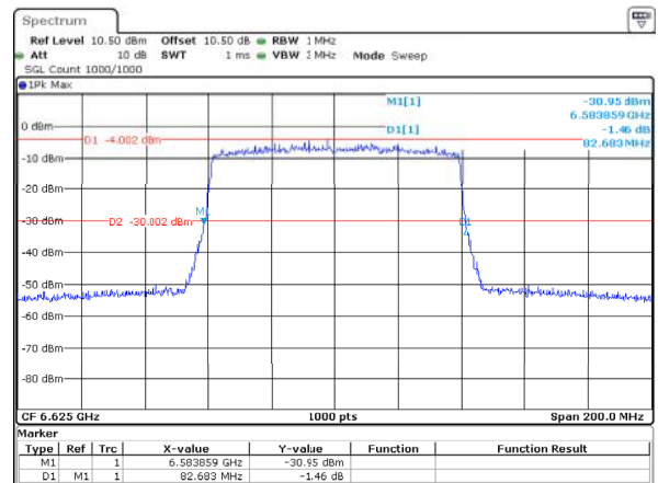
802.11ax80_6625MHz_RU_Full_ANT1 82.683MHz
