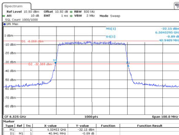
802.11ax40_6525MHz_RU_Full_ANT1 40.941MHz
