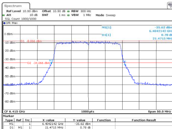
802.11ax20_6415MHz_RU_Full_ANT1 21.471MHz
