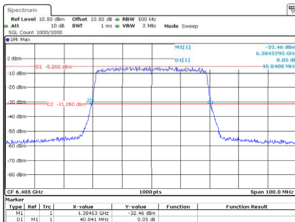
802.11ax40_6405MHz_RU_Full_ANT1 40.841MHz
