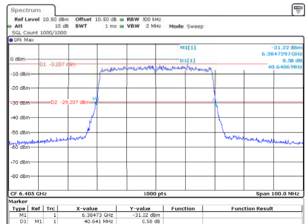
802.11ax40_6405MHz_RU_Full_ANT2 40.641MHz
