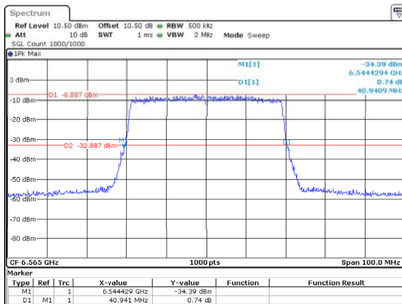
802.11ax40_6565MHz_RU_Full_ANT1 40.941MHz
