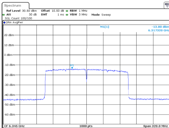
802.11ax160_6345MHz_RU_Full_ANT1 -13.80dBm/MHz
