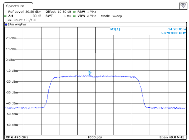
802.11ax20_6475MHz_RU_Full_ANT1 -14.28dBm/MHz
