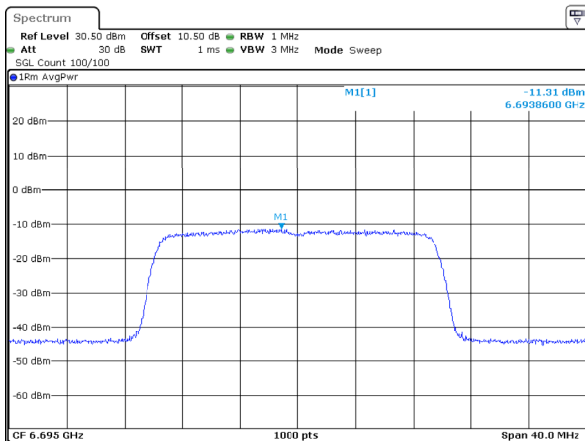
802.11ax20_6695MHz_RU_Full_ANT2 -11.31dBm/MHz
