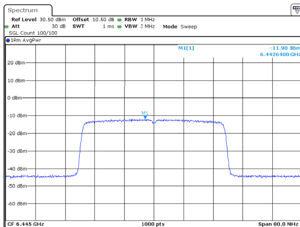
802.11ax40_6445MHz_RU_Full_ANT1 -11.90dBm/MHz
