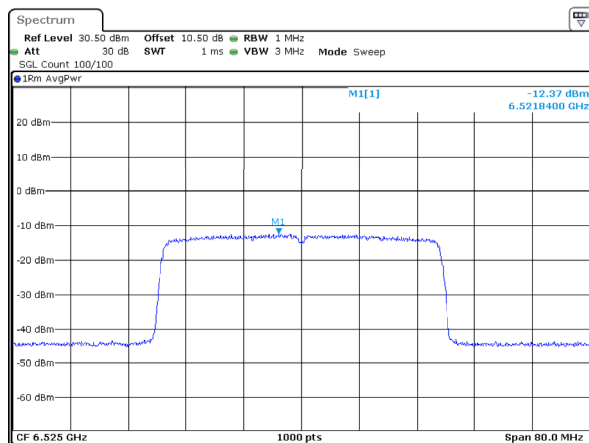
802.11ax40_6525MHz_RU_Full_ANT1 -12.37dBm/MHz
