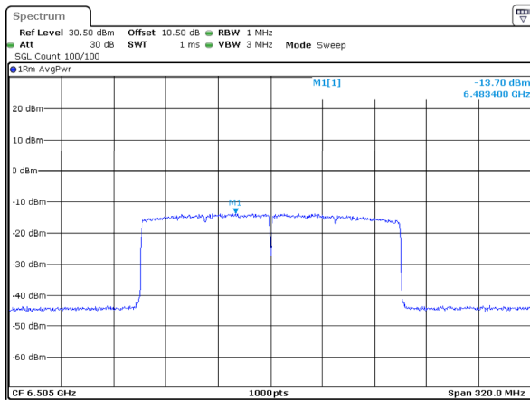
802.11ax160_6505MHz_RU_Full_ANT1 -13.70dBm/MHz
