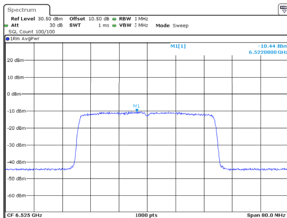
802.11ax40_6525MHz_RU_Full_ANT2 -10.44dBm/MHz
