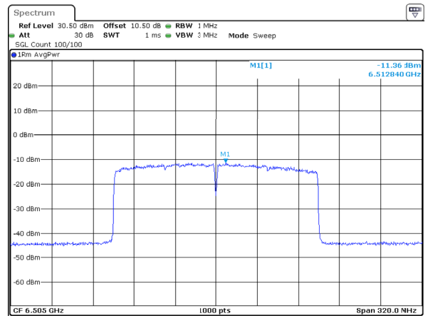
802.11ax160_6505MHz_RU_Full_ANT2 -11.36dBm/MHz
