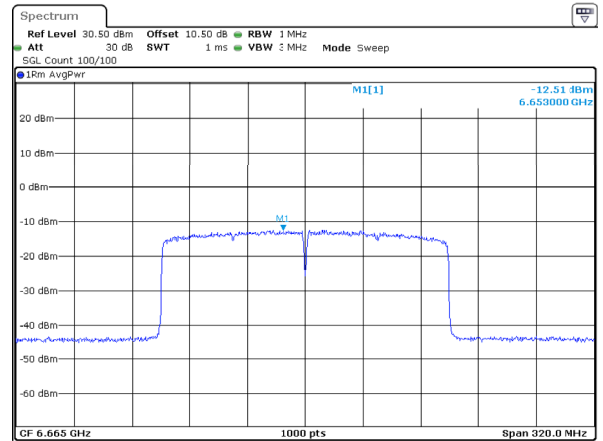
802.11ax160_6665MHz_RU_Full_ANT1 -12.51dBm/MHz
