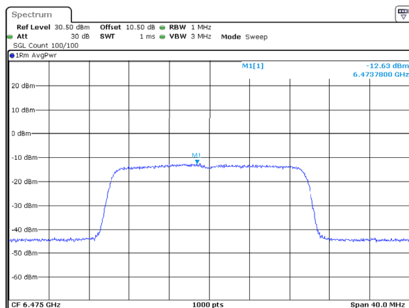
802.11ax20_6475MHz_RU_Full_ANT2 -12.63dBm/MHz
