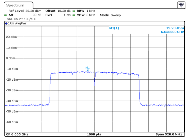
802.11ax160_6665MHz_RU_Full_ANT2 -12.28dBm/MHz
