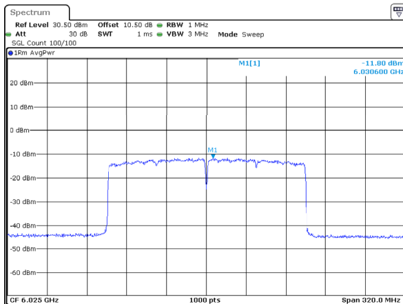
802.11ax160_6025MHz_RU_Full_ANT1 -11.80dBm/MHz
