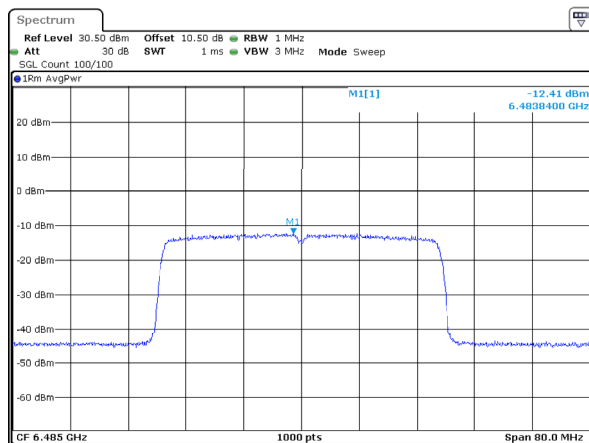
802.11ax40_6485MHz_RU_Full_ANT1 -12.41dBm/MHz
