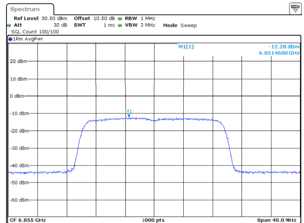
802.11ax20_6855MHz_RU_Full_ANT2 -12.28dBm/MHz
