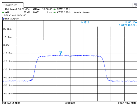
802.11ax20_6515MHz_RU_Full_ANT2 -11.83dBm/MHz
