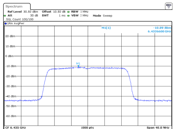
802.11ax20_6435MHz_RU_Full_ANT2 -10.89dBm/MHz
