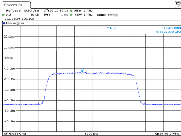
802.11ax20_6855MHz_RU_Full_ANT1 -13.54dBm/MHz
