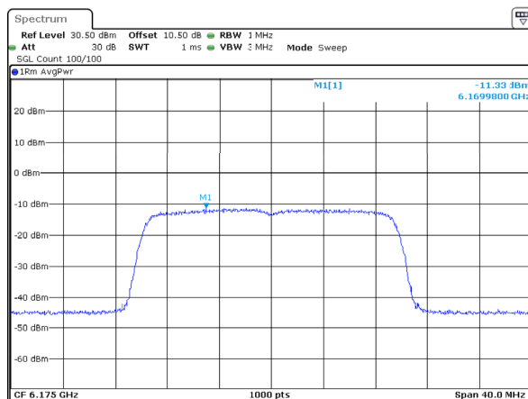
802.11ax20_6175MHz_RU_Full_ANT1 -11.33dBm/MHz
