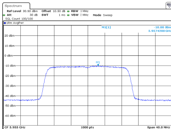
802.11ax20_5955MHz_RU_Full_ANT2 -10.00dBm/MHz
