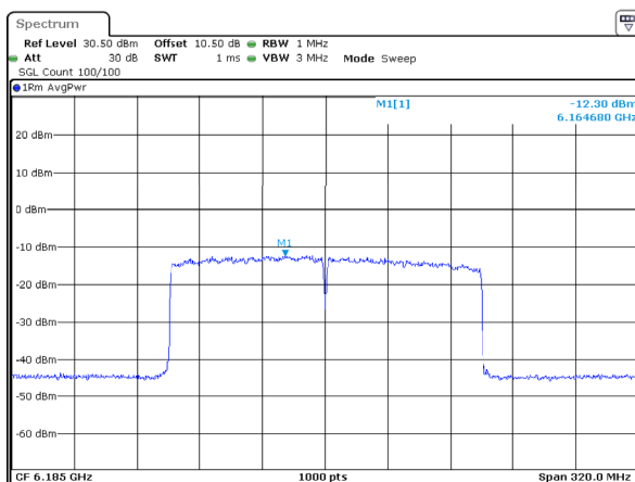
802.11ax160_6185MHz_RU_Full_ANT2 -12.30dBm/MHz
