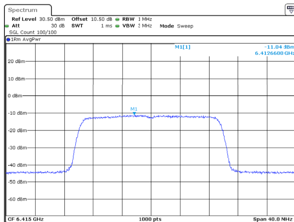
802.11ax20_6415MHz_RU_Full_ANT2 -11.04dBm/MHz
