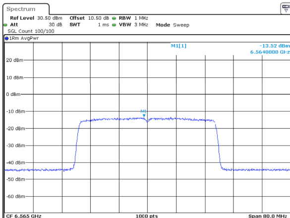
802.11ax40_6565MHz_RU_Full_ANT1 -13.52dBm/MHz
