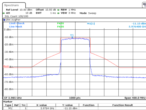
802.11ax80_5985MHz_RU_Full_ANT 2
