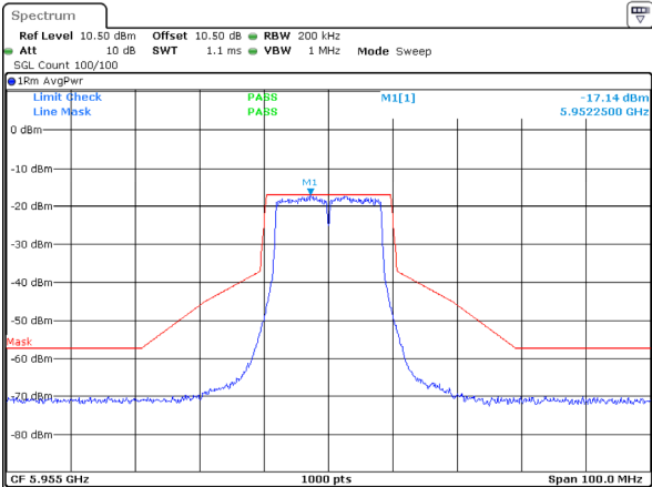
802.11a_5955MHz_ANT 1
