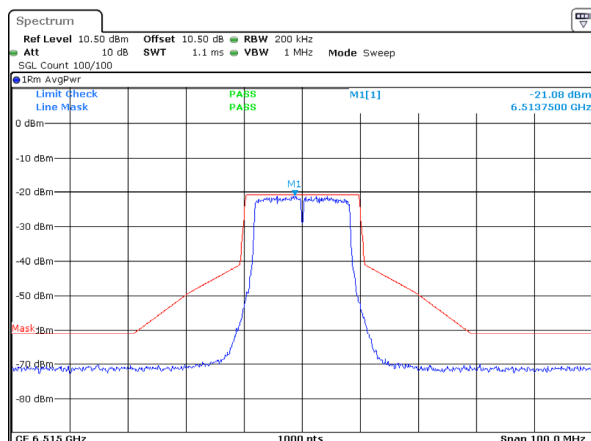
802.11a_6515MHz_ANT 1
