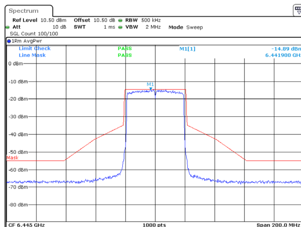
802.11ax40_6445MHz_RU_Full_ANT 1
