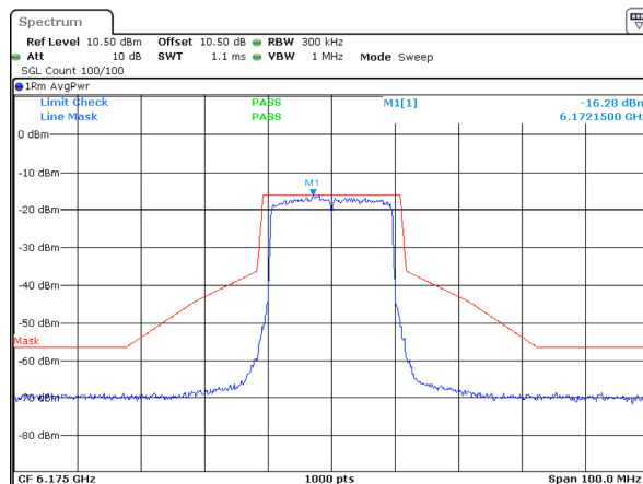
802.11ax20_6175MHz_RU_Full_ANT 1
