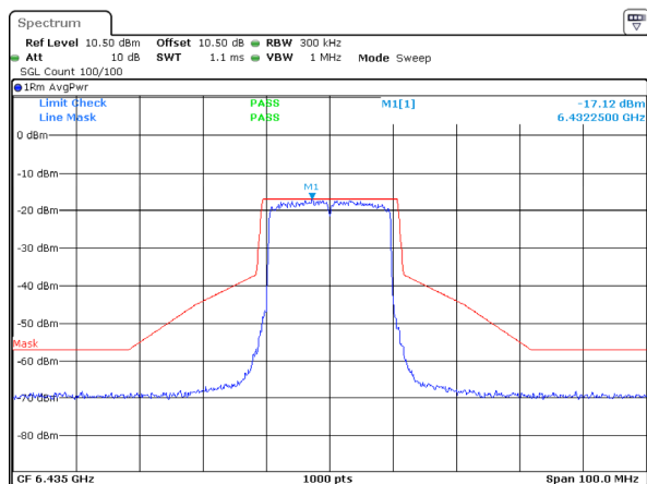
802.11ax20_6435MHz_RU_Full_ANT 1
