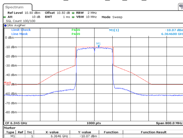
802.11ax160_6345MHz_RU_Full_ANT 2
