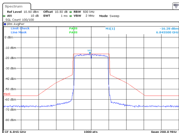
802.11ax40_6845MHz_RU_Full_ANT 1
