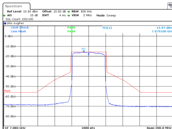
802.11ax40_7085MHz_RU_Full_ANT 1
