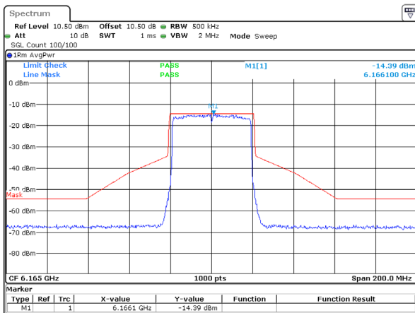
802.11ax40_6165MHz_RU_Full_ANT 2
