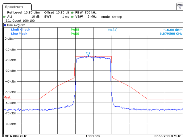
802.11ax40_6885MHz_RU_Full_ANT 1
