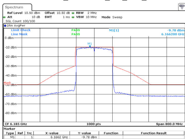
802.11ax160_6185MHz_RU_Full_ANT 2
