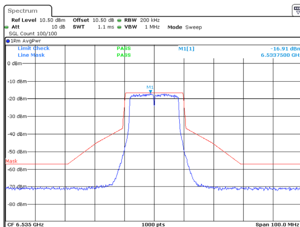
802.11a_6535MHz_ANT 2
