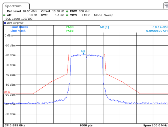
802.11ax20_6895MHz_RU_Full_ANT 1
