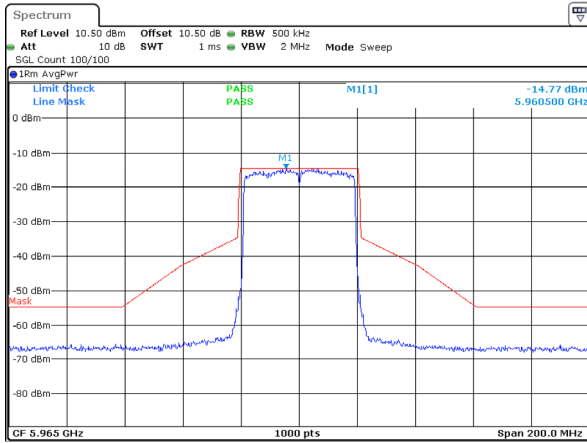
802.11ax40_5965MHz_RU_Full_ANT 1
