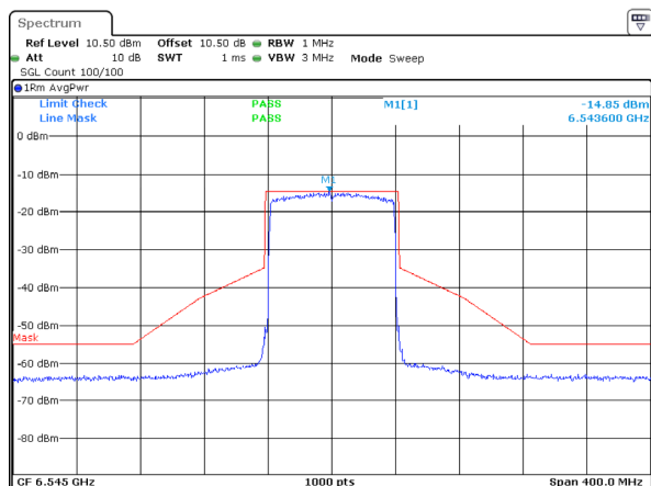
802.11ax80_6545MHz_RU_Full_ANT 1
