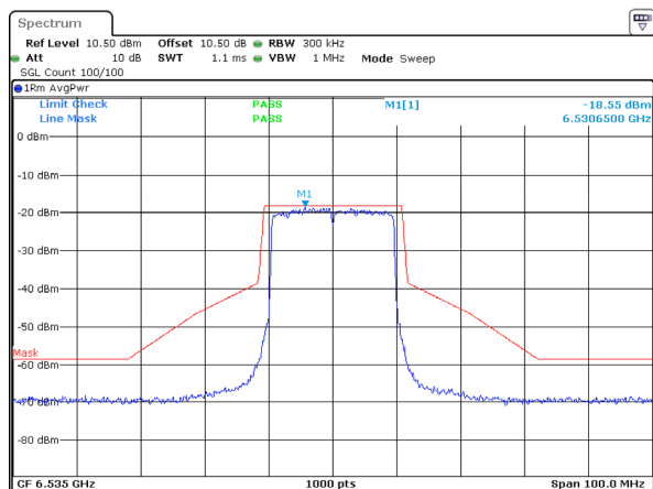
802.11ax20_6535MHz_RU_Full_ANT 1
