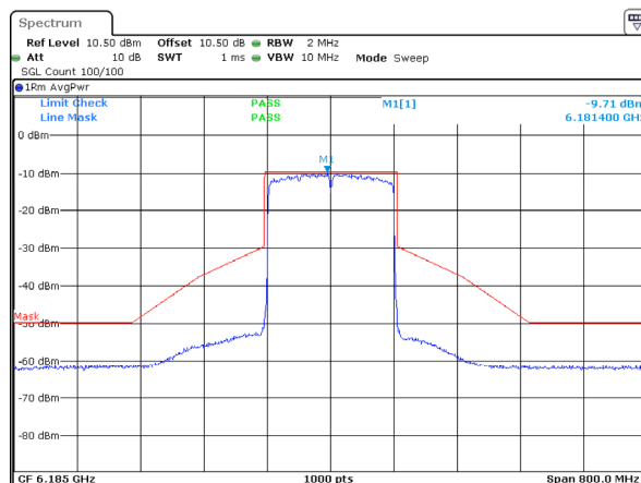
802.11ax160_6185MHz_RU_Full_ANT 1
