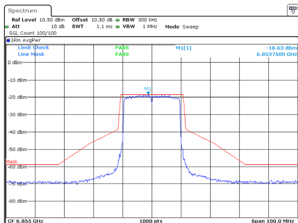
802.11ax20_6855MHz_RU_Full_ANT 1
