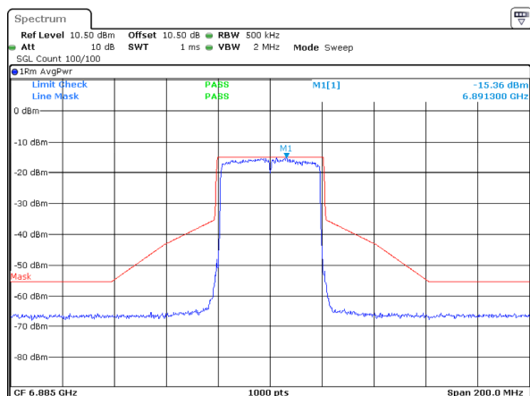
802.11ax40_6885MHz_RU_Full_ANT 2
