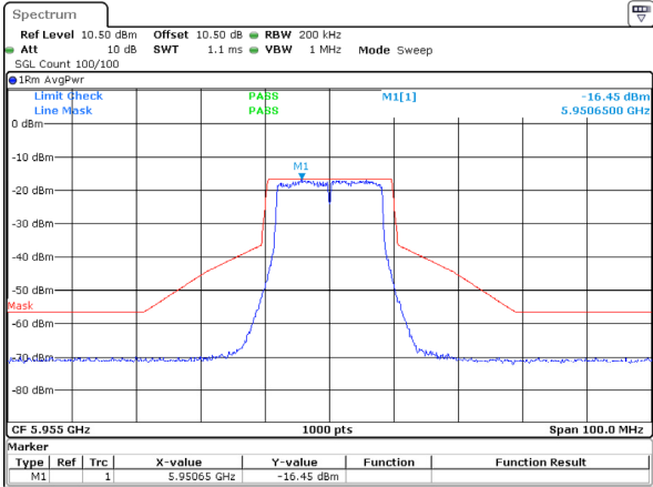
802.11a_5955MHz_ANT 2
