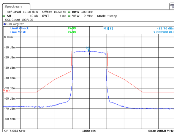
802.11ax40_7085MHz_RU_Full_ANT 2
