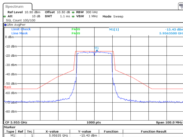
802.11ax20_5955MHz_RU_Full_ANT 2
