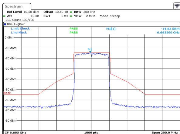
802.11ax40_6685MHz_RU_Full_ANT 2
