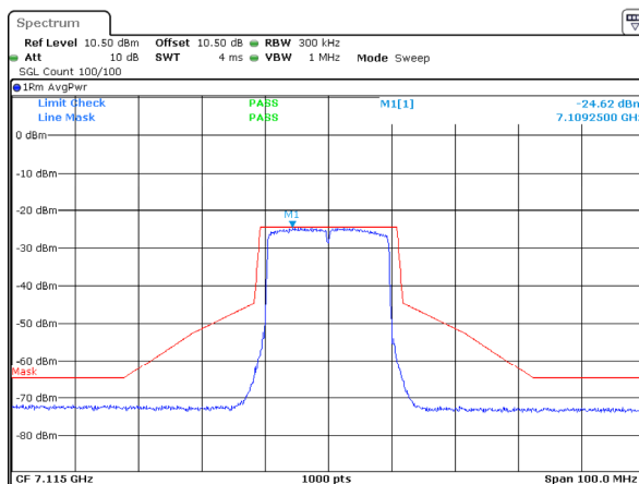
802.11ax20_7115MHz_RU_Full_ANT 2
