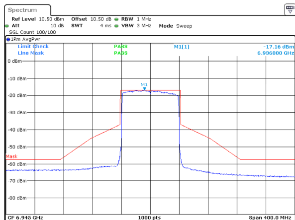
802.11ax80_6945MHz_RU_Full_ANT 1
