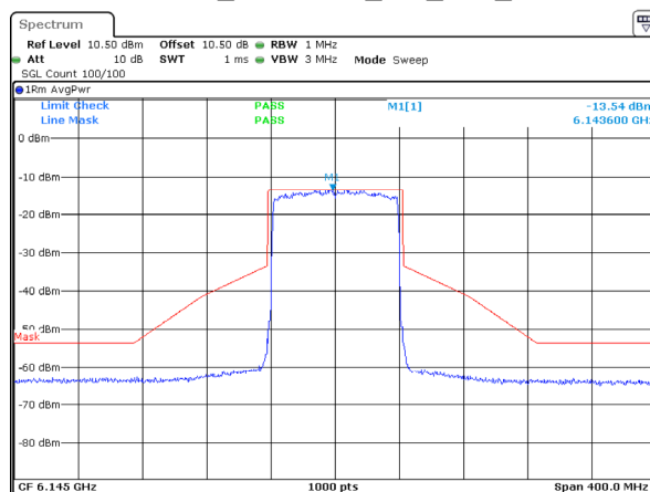
802.11ax80_6145MHz_RU_Full_ANT 1
