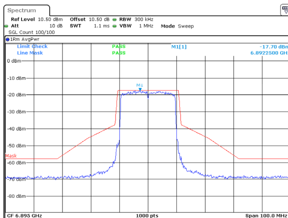
802.11ax20_6895MHz_RU_Full_ANT 2
