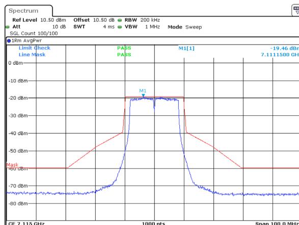
802.11a_7115MHz_ANT 1
