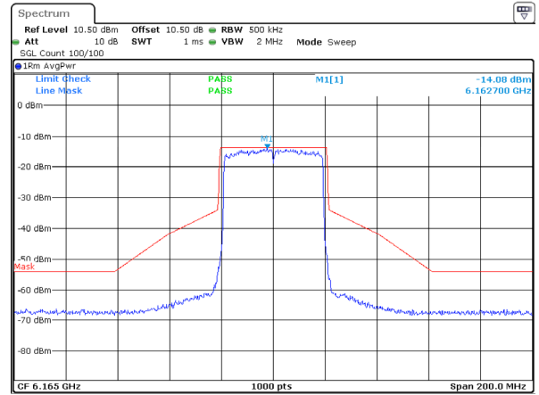
802.11ax40_6165MHz_RU_Full_ANT 1
