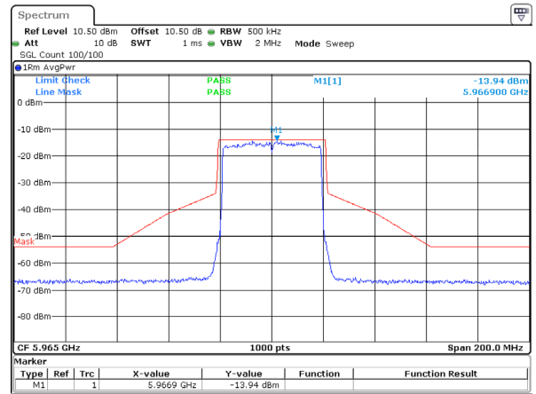
802.11ax40_5965MHz_RU_Full_ANT 2
