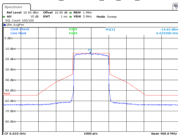
802.11ax80_6625MHz_RU_Full_ANT 2
