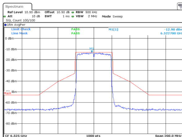
802.11ax40_6525MHz_RU_Full_ANT 2
