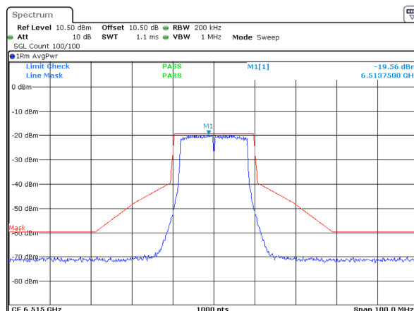
802.11a_6515MHz_ANT 2
