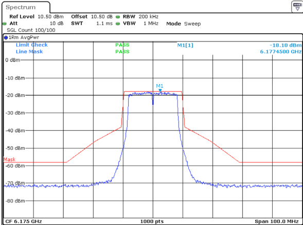
802.11a_6175MHz_ANT 1
