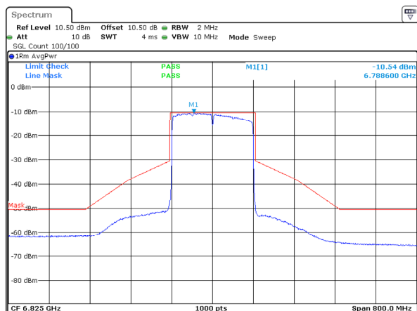
802.11ax160_6825MHz_RU_Full_ANT 1
