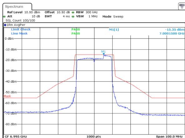
802.11ax20_6995MHz_RU_Full_ANT 2
