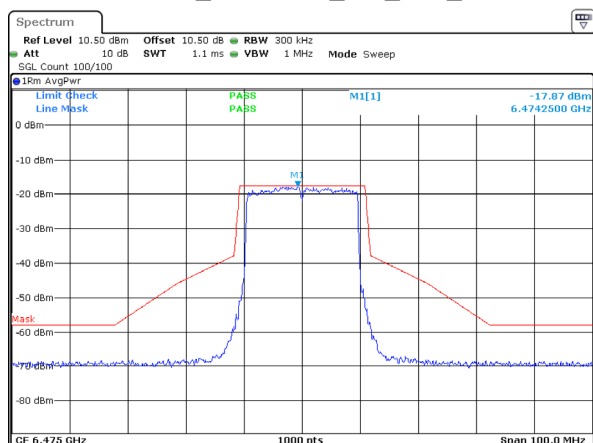
802.11ax20_6475MHz_RU_Full_ANT 2
