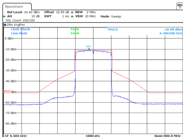
802.11ax160_6505MHz_RU_Full_ANT 1
