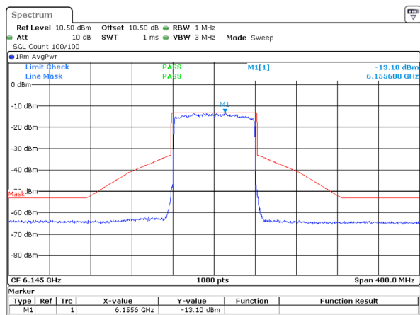
802.11ax80_6145MHz_RU_Full_ANT 2
