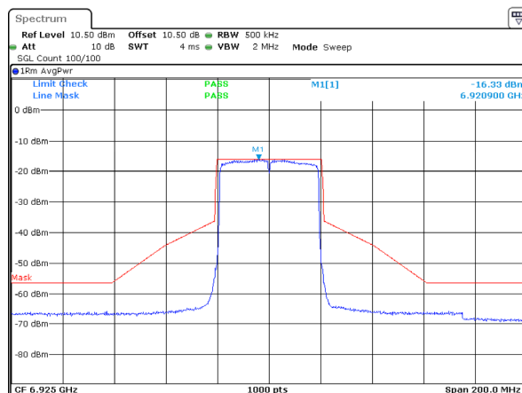
802.11ax40_6925MHz_RU_Full_ANT 2
