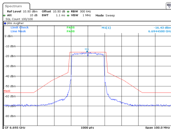
802.11ax20_6695MHz_RU_Full_ANT 1
