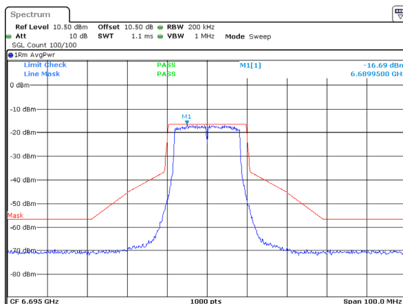
802.11a_6695MHz_ANT 1
