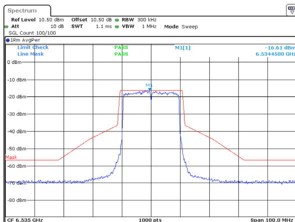
802.11ax20_6535MHz_RU_Full_ANT 2
