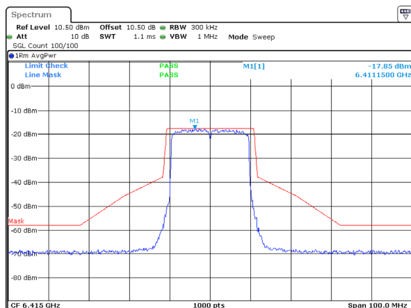
802.11ax20_6415MHz_RU_Full_ANT 1
