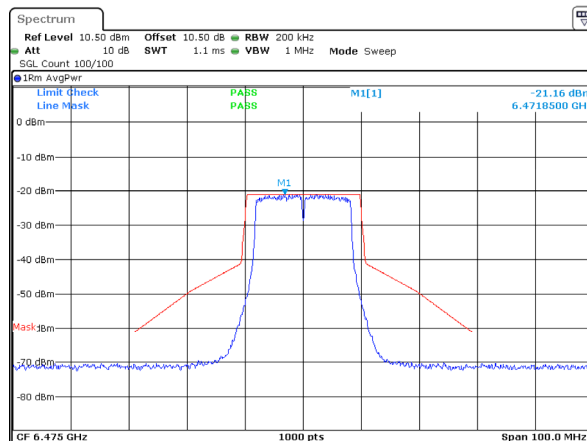
802.11a_6475MHz_ANT 1
