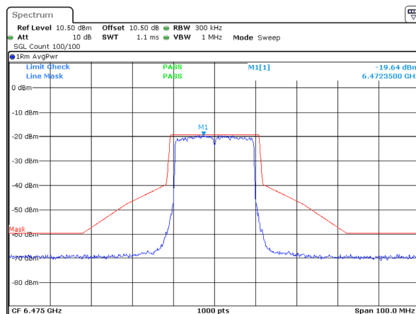
802.11ax20_6475MHz_RU_Full_ANT 1
