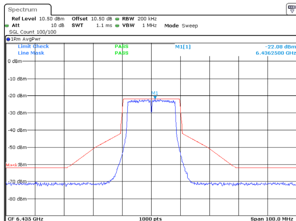
802.11a_6435MHz_ANT 1
