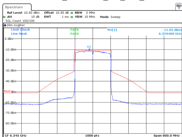
802.11ax160_6345MHz_RU_Full_ANT 1
