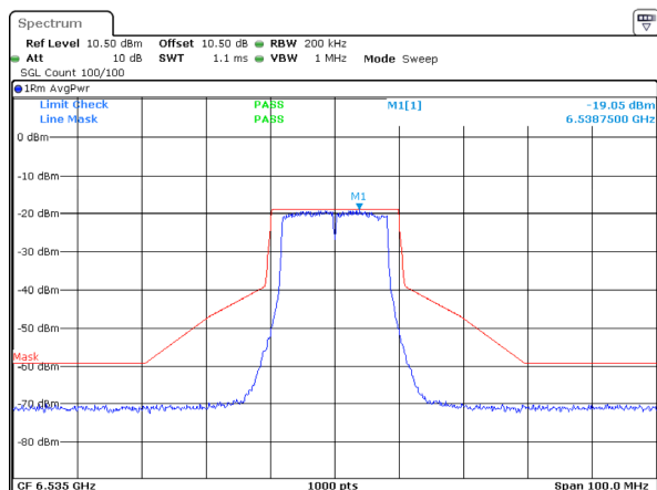
802.11a_6535MHz_ANT 1
