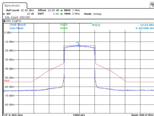
802.11ax80_6465MHz_RU_Full_ANT 1
