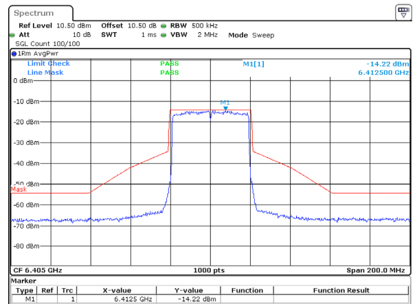
802.11ax40_6405MHz_RU_Full_ANT 2
