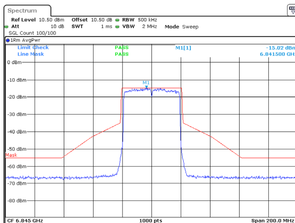
802.11ax40_6845MHz_RU_Full_ANT 2
