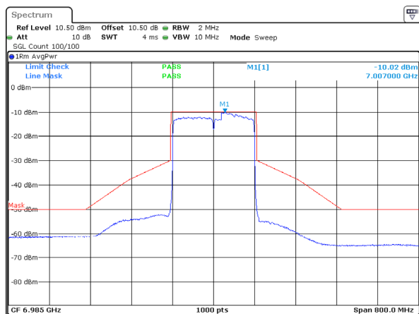
802.11ax160_6985MHz_RU_Full_ANT 1
