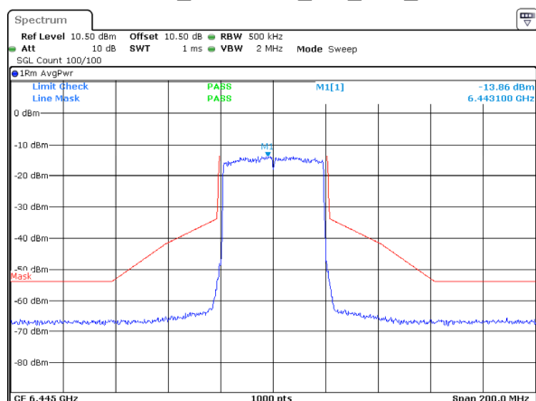
802.11ax40_6445MHz_RU_Full_ANT 2
