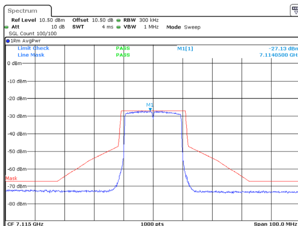
802.11ax20_7115MHz_RU_Full_ANT 1
