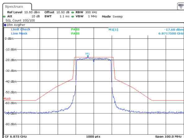
802.11ax20_6875MHz_RU_Full_ANT 2
