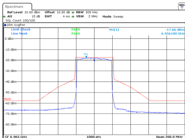
802.11ax40_6965MHz_RU_Full_ANT 1
