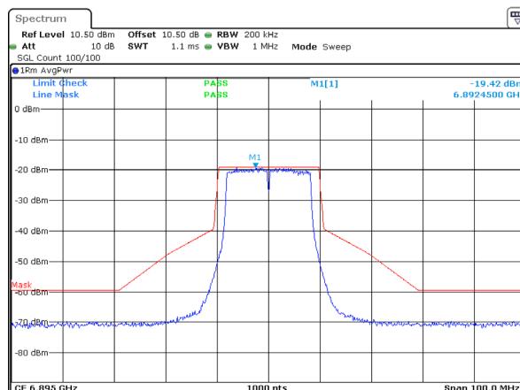
802.11a_6895MHz_ANT 2
