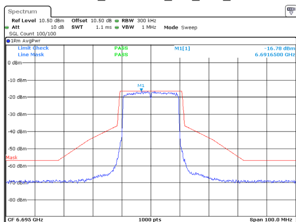
802.11ax20_6695MHz_RU_Full_ANT 2
