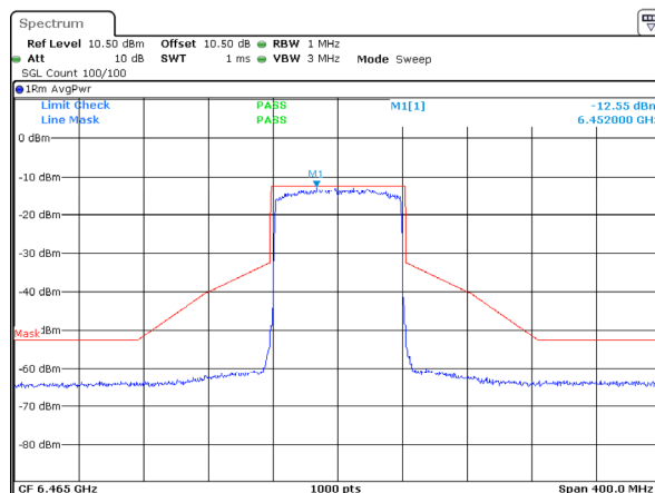
802.11ax80_6465MHz_RU_Full_ANT 2
