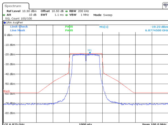
802.11a_6875MHz_ANT 2
