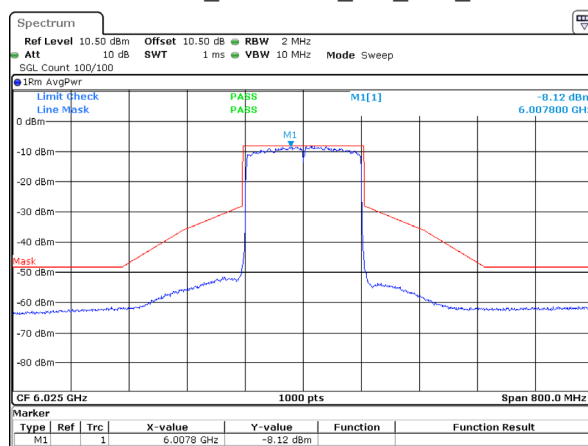
802.11ax160_6025MHz_RU_Full_ANT 2
