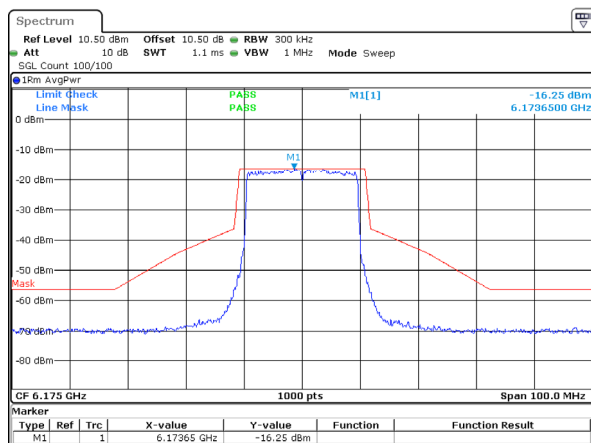
802.11ax20_6175MHz_RU_Full_ANT 2
