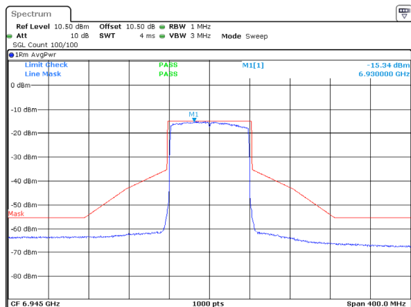
802.11ax80_6945MHz_RU_Full_ANT 2
