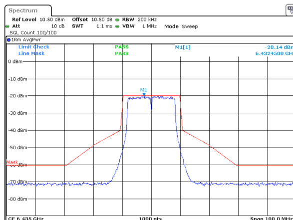
802.11a_6435MHz_ANT 2
