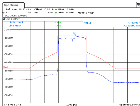
802.11ax160_6985MHz_RU_Full_ANT 2
