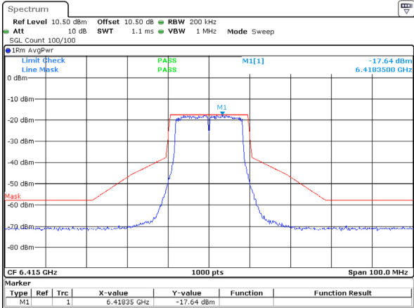
802.11a_6415MHz_ANT 2
