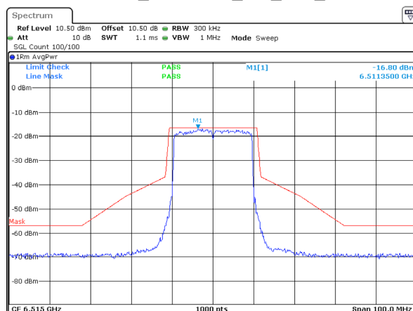
802.11ax20_6515MHz_RU_Full_ANT 2
