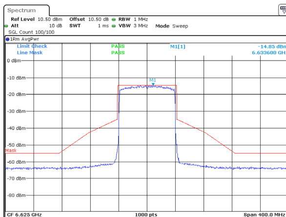
802.11ax80_6625MHz_RU_Full_ANT 1
