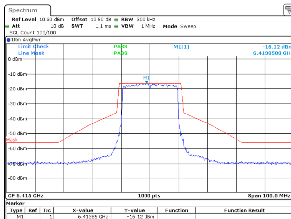
802.11ax20_6415MHz_RU_Full_ANT 2
