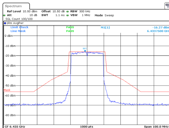
802.11ax20_6435MHz_RU_Full_ANT 2
