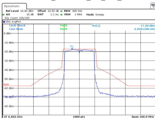
802.11ax20_6855MHz_RU_Full_ANT 2
