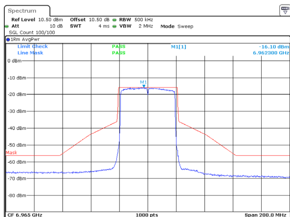
802.11ax40_6965MHz_RU_Full_ANT 2
