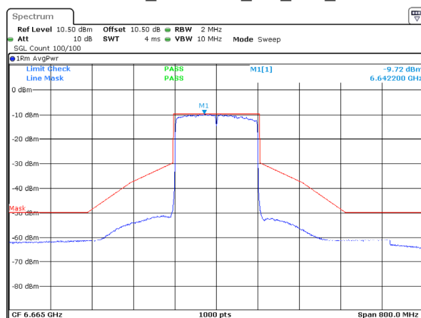
802.11ax160_6665MHz_RU_Full_ANT 2
