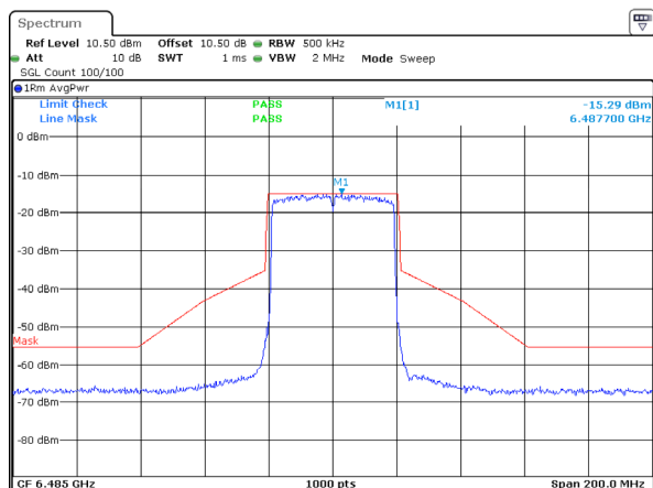
802.11ax40_6485MHz_RU_Full_ANT 1
