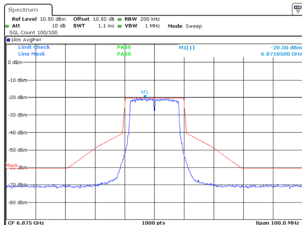
802.11a_6875MHz_ANT 1
