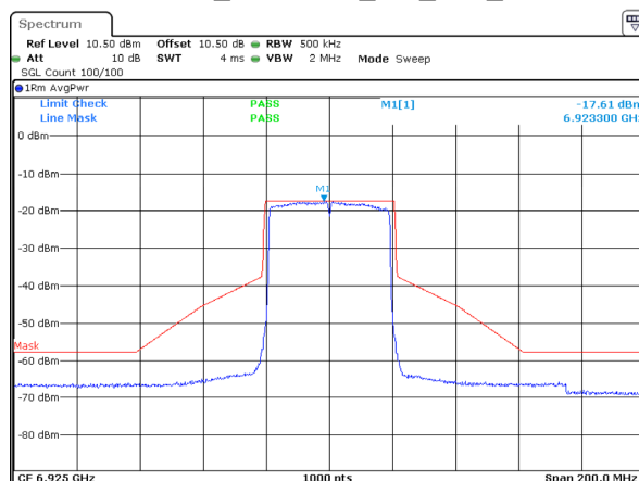
802.11ax40_6925MHz_RU_Full_ANT 1
