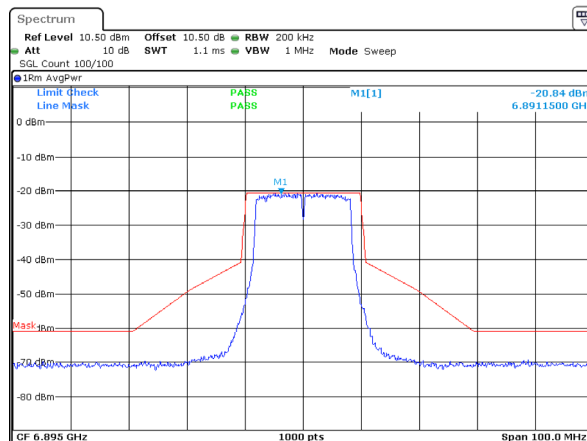
802.11a_6895MHz_ANT 1
