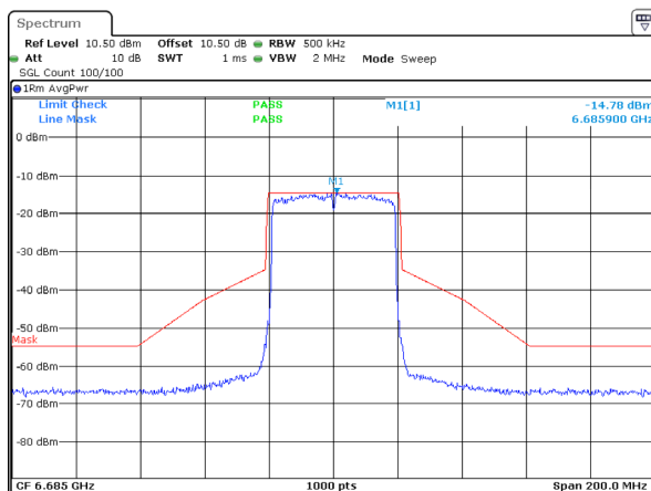
802.11ax40_6685MHz_RU_Full_ANT 1
