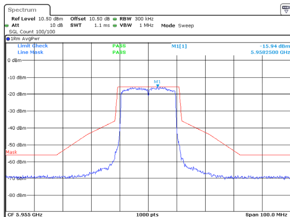
802.11ax20_5955MHz_RU_Full_ANT 1
