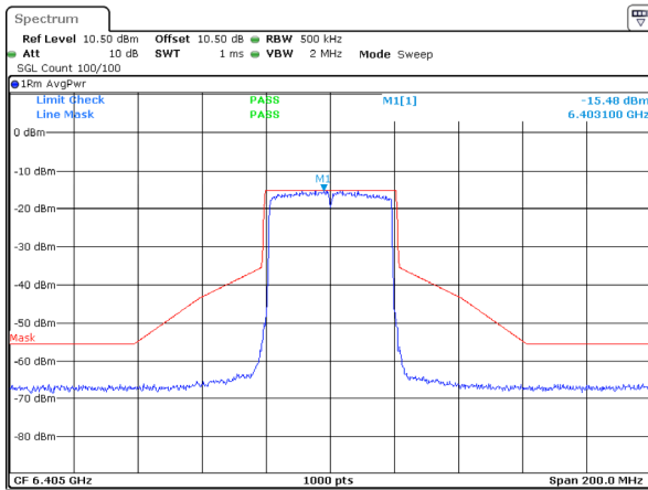
802.11ax40_6405MHz_RU_Full_ANT 1
