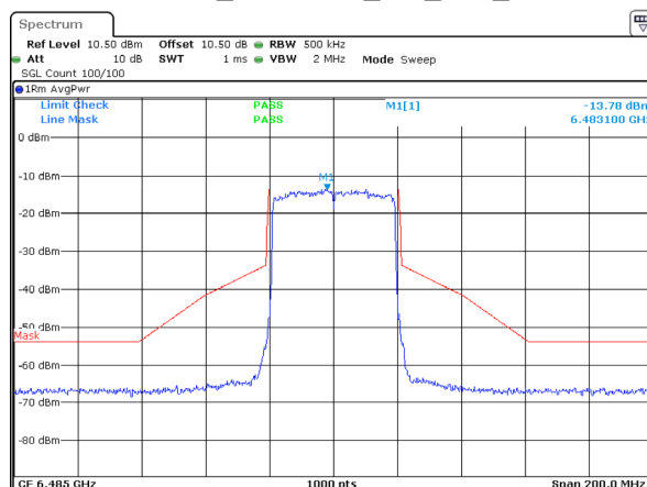
802.11ax40_6485MHz_RU_Full_ANT 2
