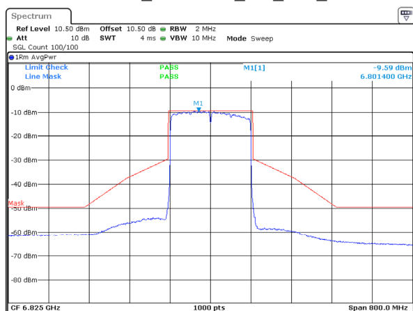
802.11ax160_6825MHz_RU_Full_ANT 2
