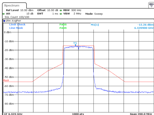
802.11ax40_6525MHz_RU_Full_ANT 1
