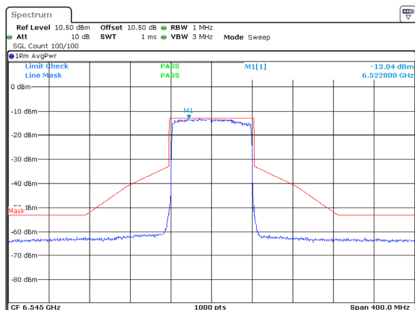
802.11ax80_6545MHz_RU_Full_ANT 2
