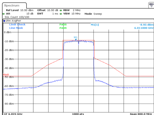
802.11ax160_6025MHz_RU_Full_ANT 1
