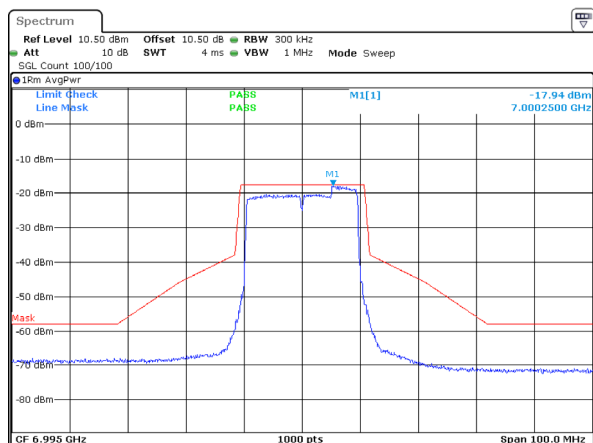
802.11ax20_6995MHz_RU_Full_ANT 1
