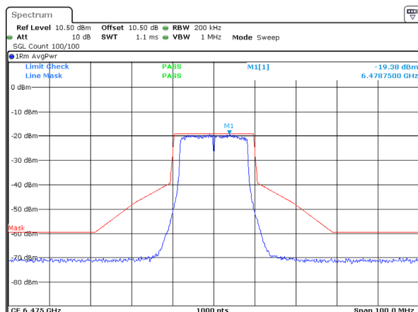
802.11a_6475MHz_ANT 2
