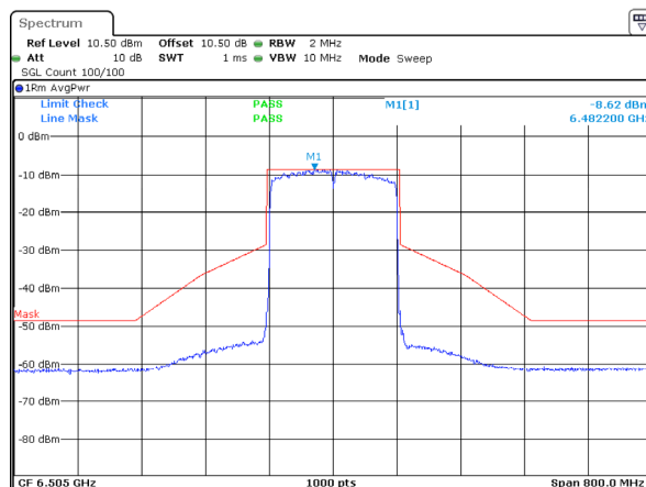
802.11ax160_6505MHz_RU_Full_ANT 2
