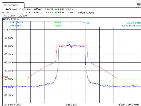
802.11ax20_6875MHz_RU_Full_ANT 1
