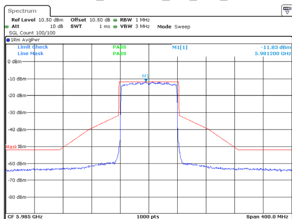
802.11ax80_5985MHz_RU_Full_ANT 1
