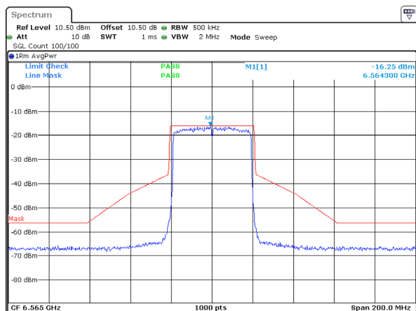
802.11ax40_6565MHz_RU_Full_ANT 1
