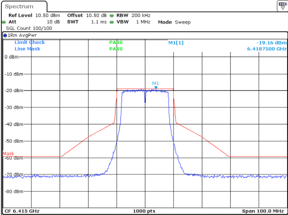
802.11a_6415MHz_ANT 1
