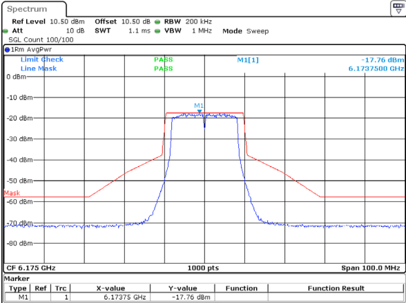
802.11a_6175MHz_ANT 2
