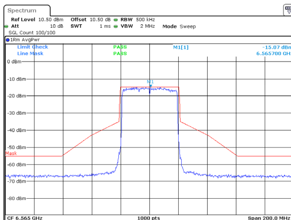
802.11ax40_6565MHz_RU_Full_ANT 2
