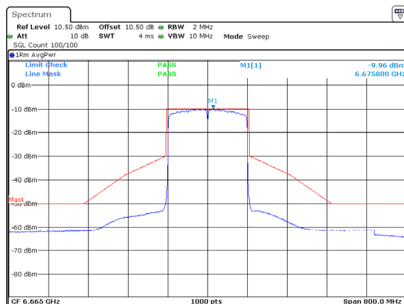
802.11ax160_6665MHz_RU_Full_ANT 1
