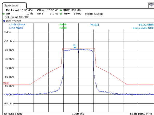
802.11ax20_6515MHz_RU_Full_ANT 1
