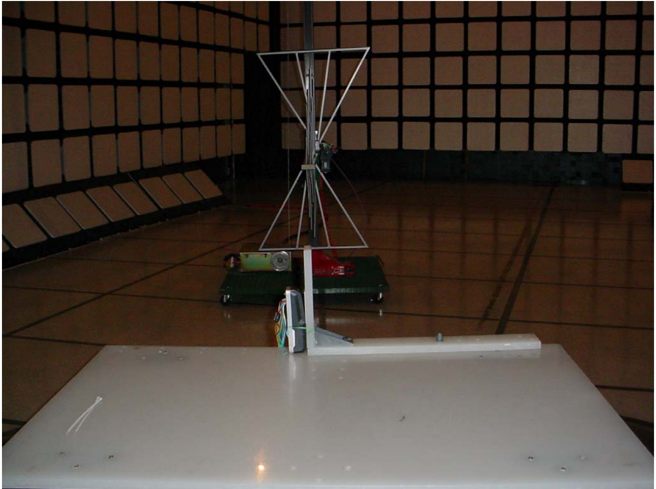
Radiated Emissions at 3 m Distance (30 MHz to 1000 MHz)
