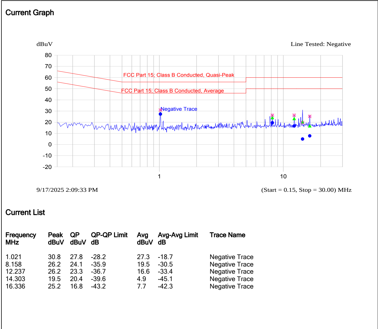
Plot 5.1.3.2. Power Line Conducted Emissions Line Voltage: 12 VDC; Line Tested: Negative
