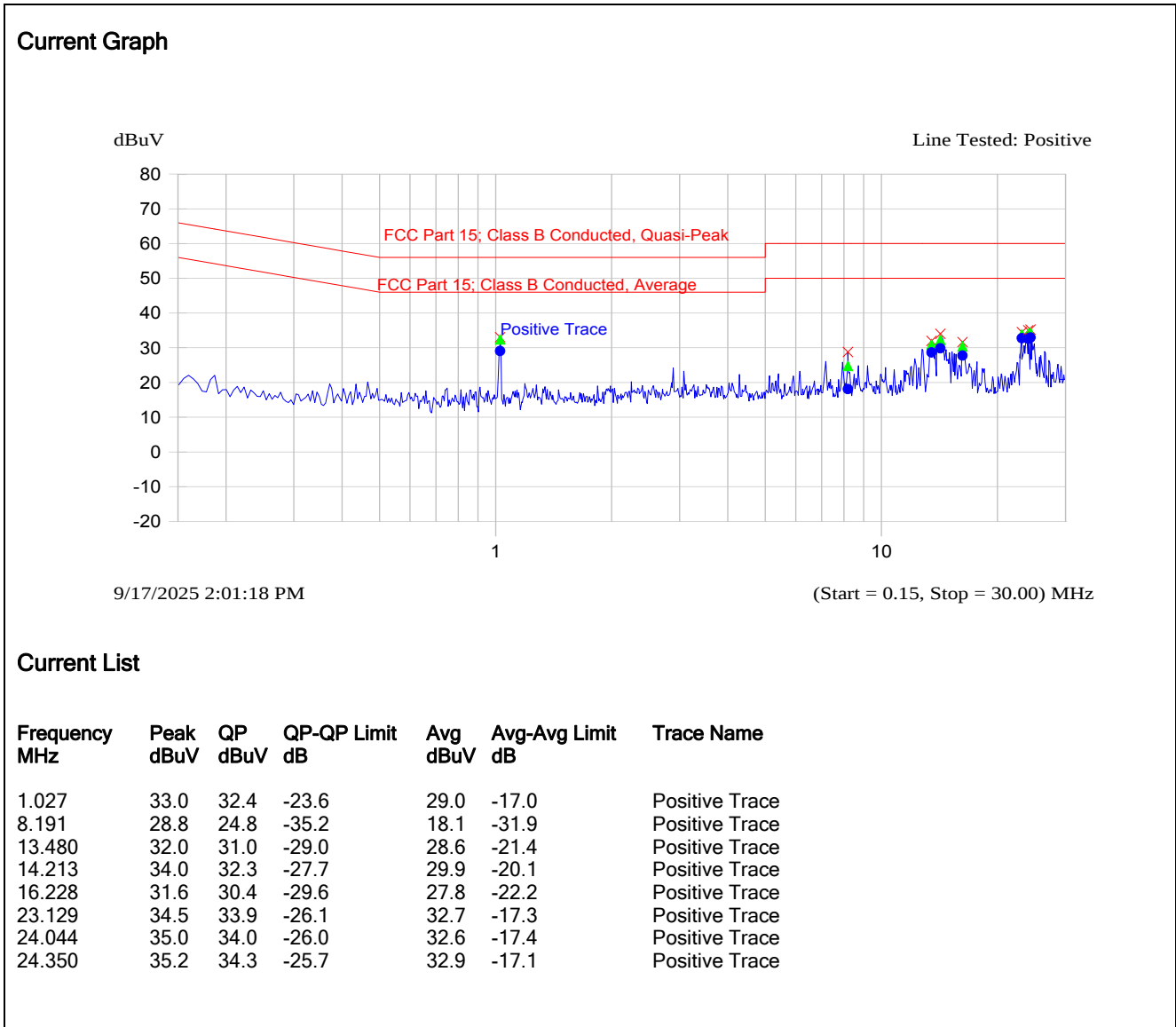
Plot 5.1.3.1. Power Line Conducted Emissions Line Voltage: 12 VDC; Line Tested: Positive
