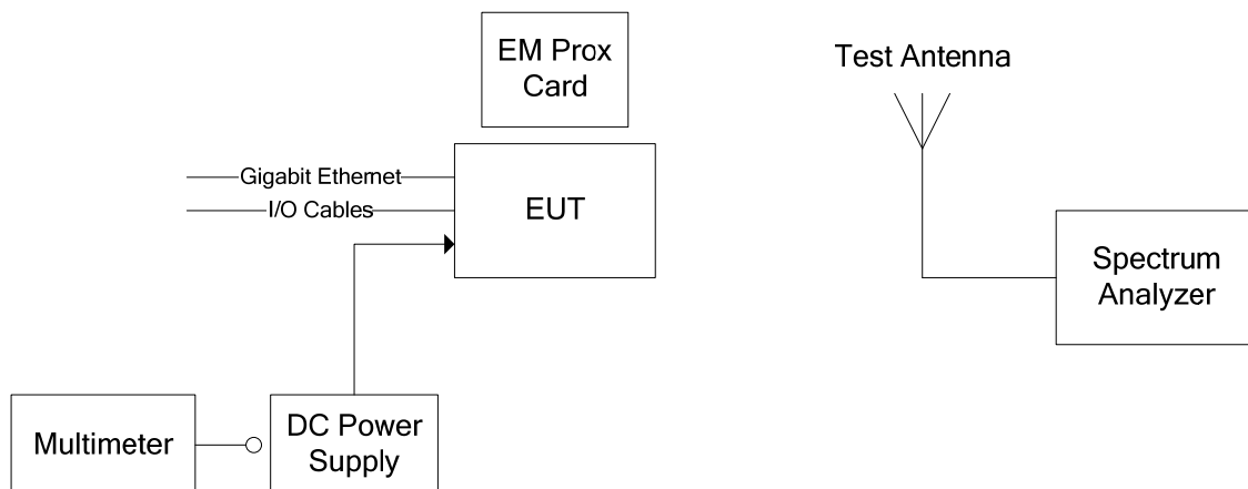
EUT Powered by External DC Power Supply
