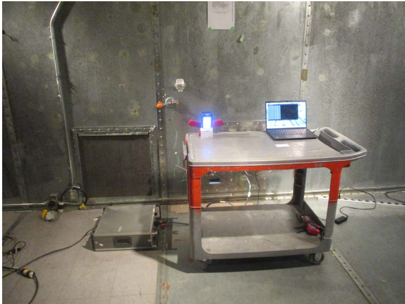
Power Line Conducted Emissions (without suppression)
