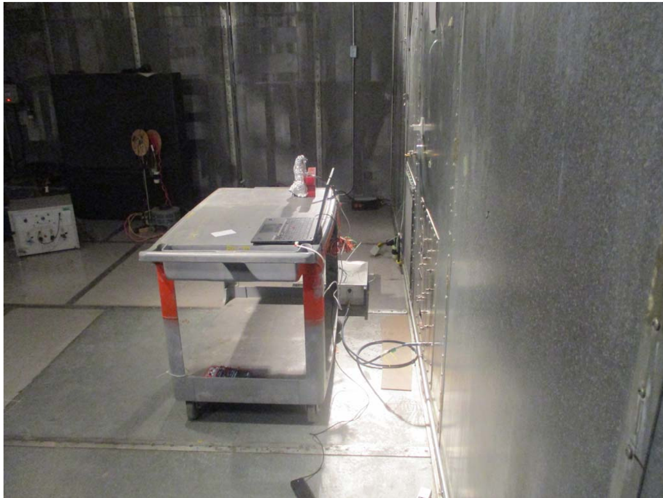
Power Line Conducted Emissions (with suppression)
