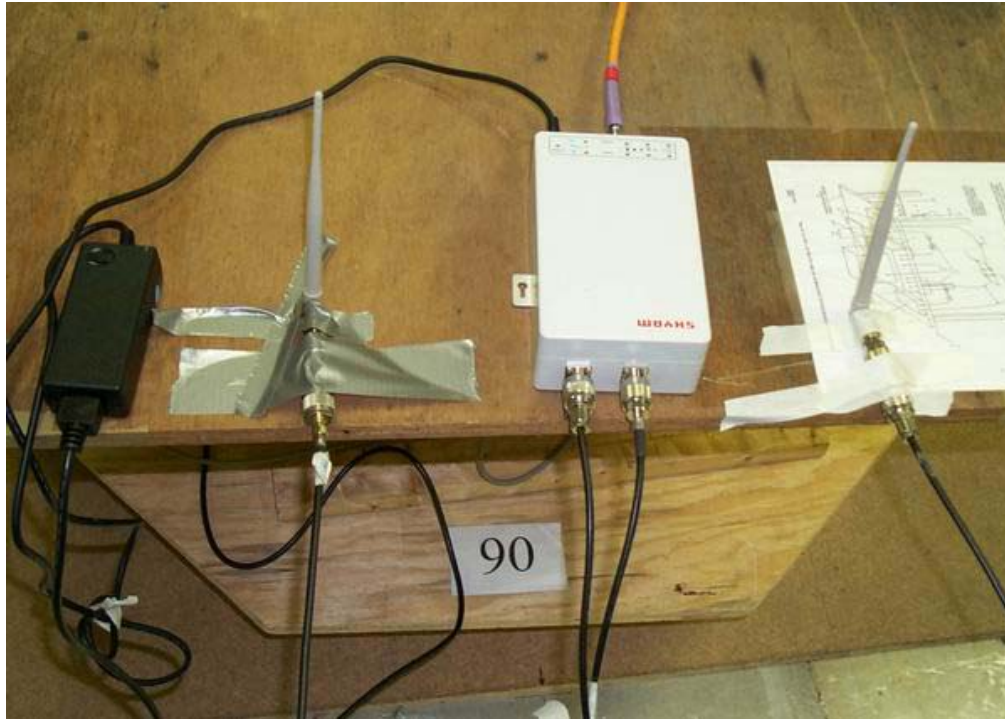
Configuration I: Top View
