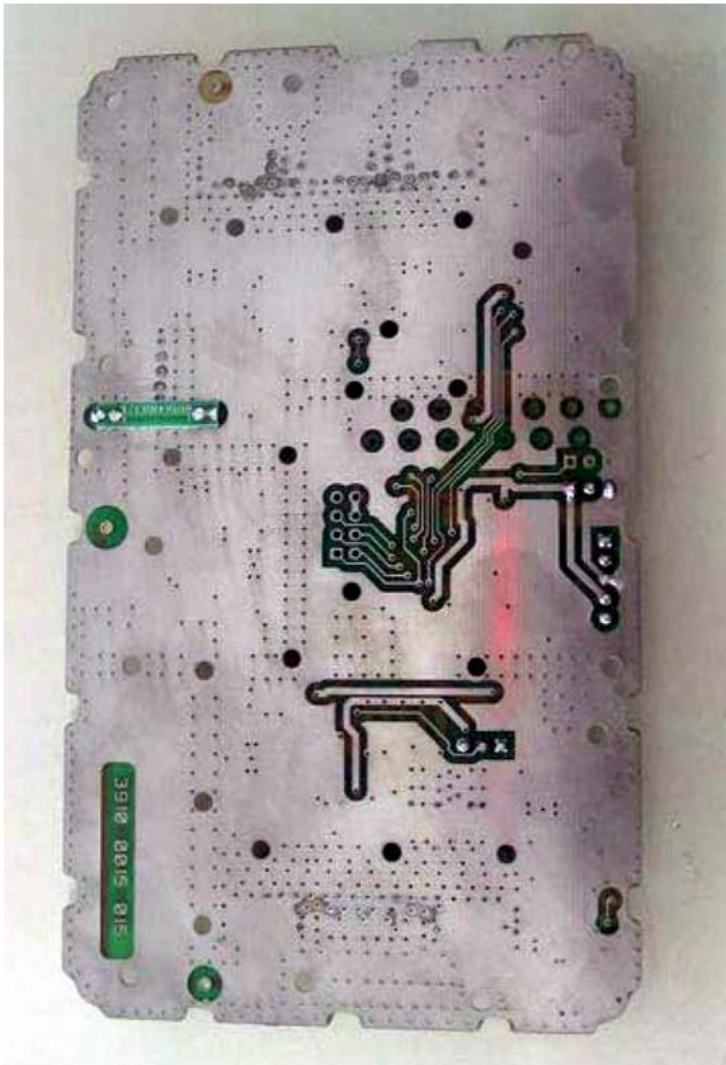
PCB2 Foil View
