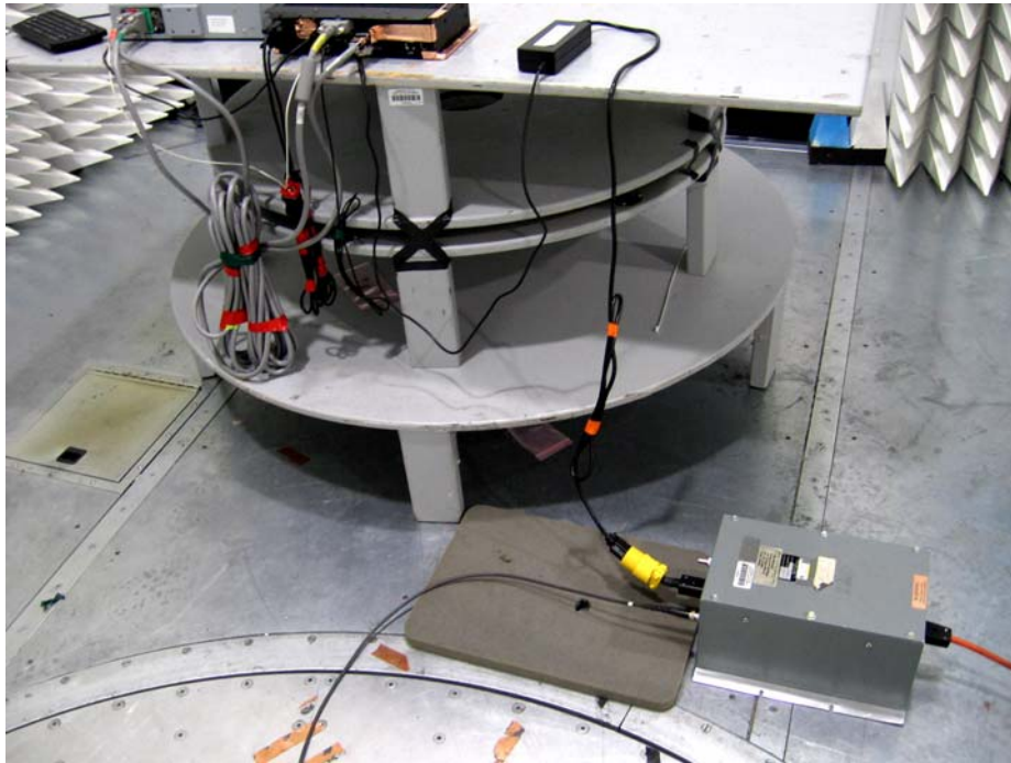
Power Line Conducted Emissions Test Configuration
