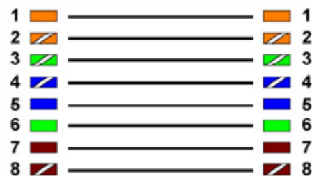
Example Straight Through Cable
