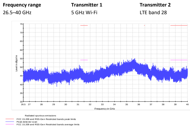
Figure 8.1-44: Radiated spurious emissions
