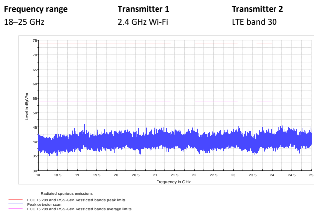
Figure 8.1-35: Radiated spurious emissions
