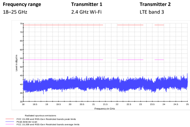
Figure 8.1-32: Radiated spurious emissions
