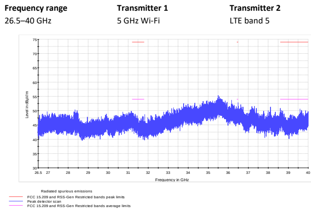
Figure 8.1-43: Radiated spurious emissions
