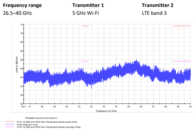
Figure 8.1-42: Radiated spurious emissions
