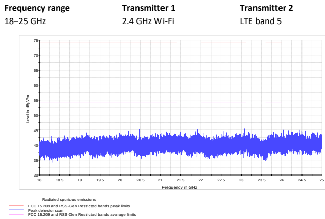
Figure 8.1-33: Radiated spurious emissions
