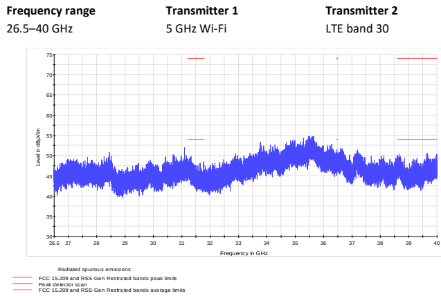
Figure 8.1-45: Radiated spurious emissions
