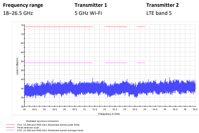
Figure 8.1-38: Radiated spurious emissions
