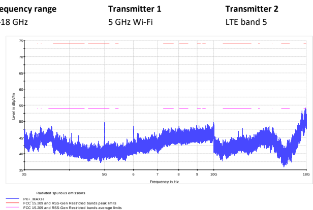
Figure 8.1-28: Radiated spurious emissions
