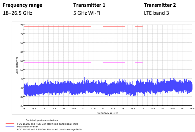
Figure 8.1-37: Radiated spurious emissions
