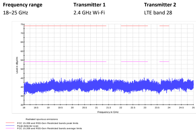
Figure 8.1-34: Radiated spurious emissions
