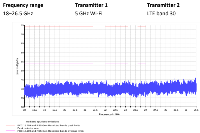
Figure 8.1-40: Radiated spurious emissions
