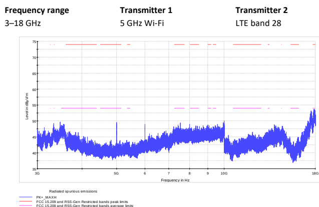
Figure 8.1-29: Radiated spurious emissions
