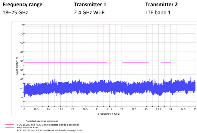
Figure 8.1-31: Radiated spurious emissions
