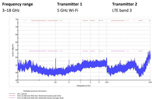
Figure 8.1-27: Radiated spurious emissions
