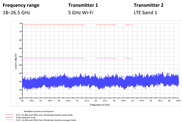
Figure 8.1-36: Radiated spurious emissions
