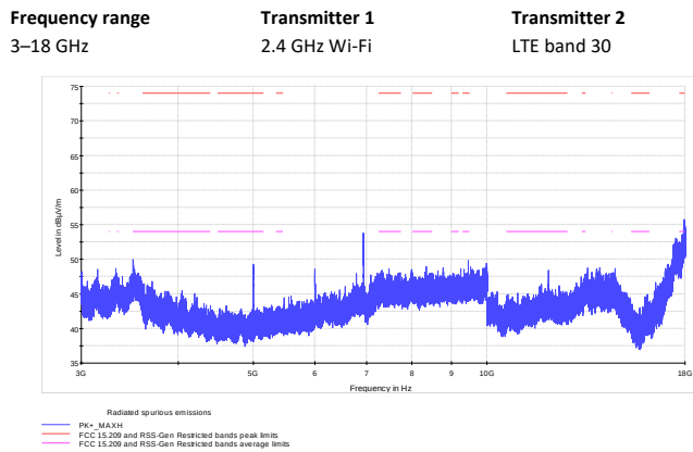
Figure 8.1-25: Radiated spurious emissions
