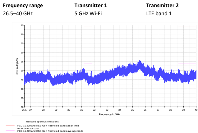
Figure 8.1-41: Radiated spurious emissions
