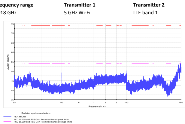
Figure 8.1-26: Radiated spurious emissions
