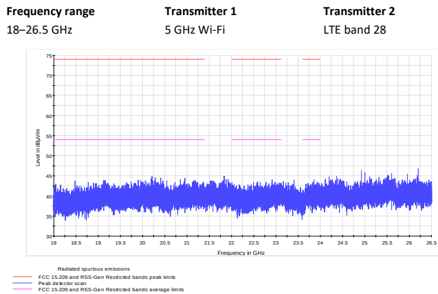
Figure 8.1-39: Radiated spurious emissions
