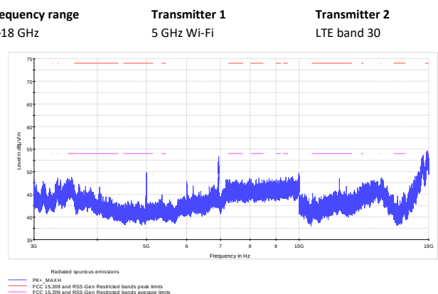
Figure 8.1-30: Radiated spurious emissions
