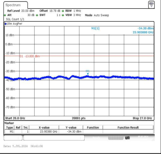
12-12-5MHz-5MHz-16QAM-16QAM-23071-23119- 1RB#0-1RB#24-20000~27000MHz-PASS
