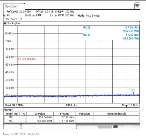
12-12-5MHz-5MHz-16QAM-16QAM-23071-23119- 1RB#0-1RB#24-30~1000MHz-PASS
