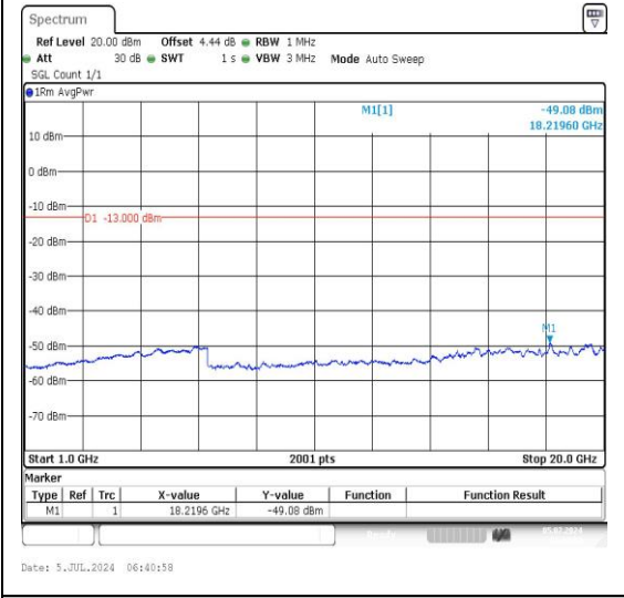
12-12-5MHz-5MHz-16QAM-16QAM-23071-23119 -1RB#0-1RB#24-1000~20000MHz-PASS
