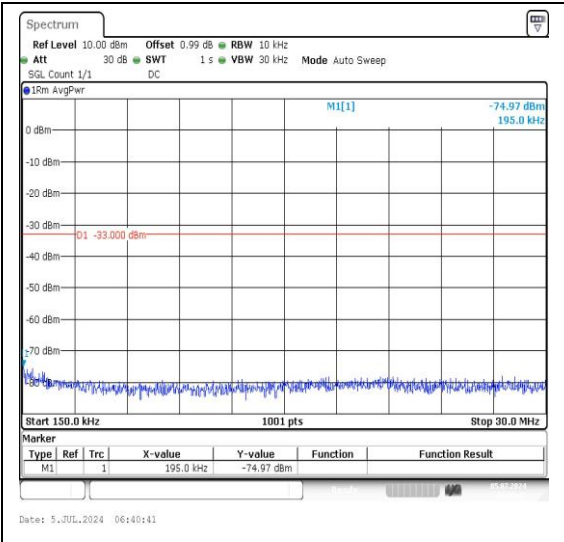
12-12-5MHz-5MHz-16QAM-16QAM-23071-23119 -1RB#0-1RB#24-0.15~30MHz-PASS
