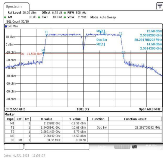
7-7-15MHz-15MHz-16QAM-16QAM-21225-21375- 75RB#0-75RB#0-PASS
