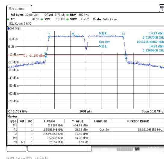
7-7-15MHz-15MHz-QPSK-QPSK-21025-21175-7 5RB#0-75RB#0-PASS
