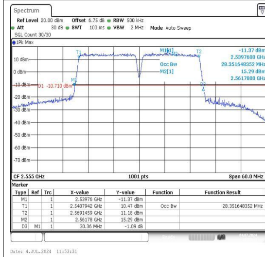
7-7-15MHz-15MHz-QPSK-QPSK-21225-21375-7 5RB#0-75RB#0-PASS
