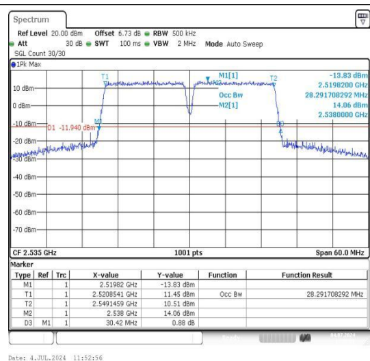
7-7-15MHz-15MHz-16QAM-16QAM-21025-21175- 75RB#0-75RB#0-PASS
