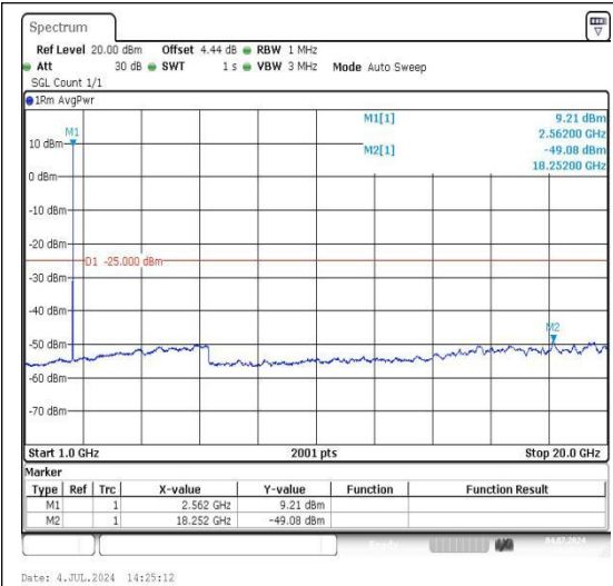
7-7-20MHz-10MHz-16QAM-16QAM-21251-21395-1RB#99-0RB#0-1000~20000MHz-PASS
