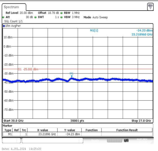
7-7-20MHz-10MHz-16QAM-16QAM-21251-21395-1RB#99-0RB#0-20000~27000MHz-PASS
