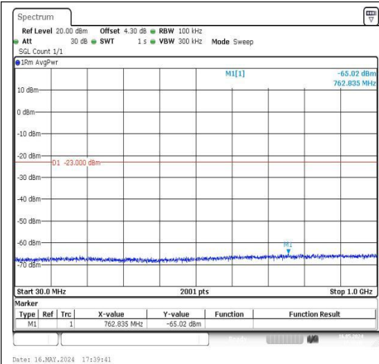
Band2_15MHz_QPSK_18900_1RB#0_30~1000_30~1000
