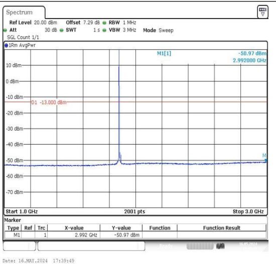
Band2_15MHz_QPSK_18900_1RB#0_1000~3000_1000~3000
