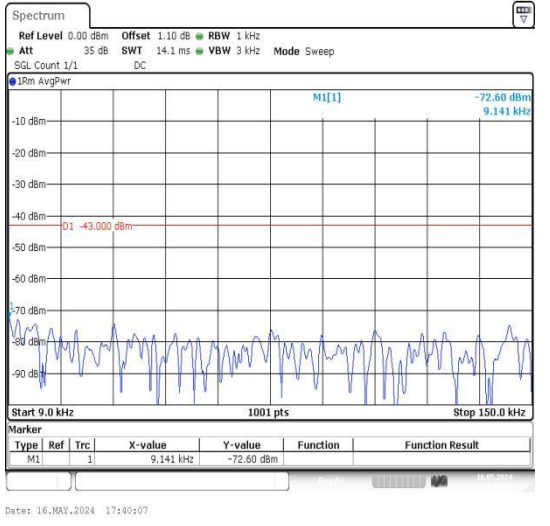
Band2_15MHz_16QAM_18900_1RB#0_0.009~0.15_0.009~0.15
