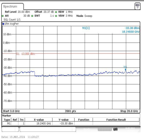
Band25_10MHz_16QAM_26090_1RB#0_3000~20000_3000~20000
