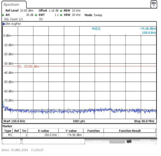
Band25_10MHz_QPSK_26365_1RB#0_0.15~30_0.15~30
