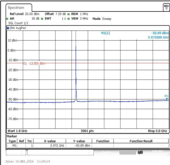
Band25_10MHz_16QAM_26090_1RB#0_1000~3000_1000~3000
