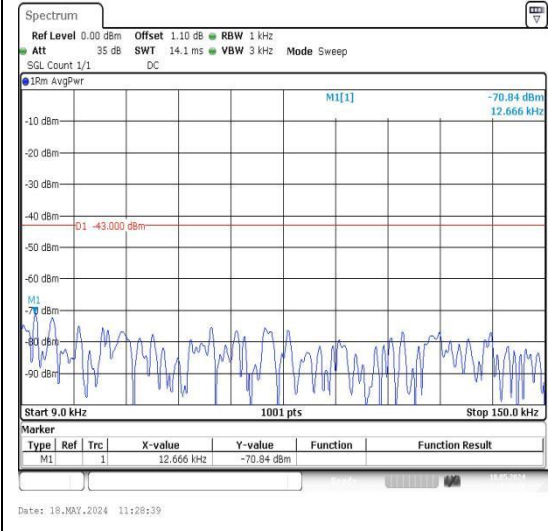
Band25_10MHz_QPSK_26365_1RB#0_0.009~0.15_0.009~0.15
