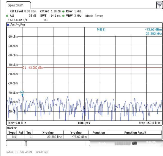
Band25_20MHz_QPSK_26365_1RB#0_0.009~0.15_0.009~0.15
