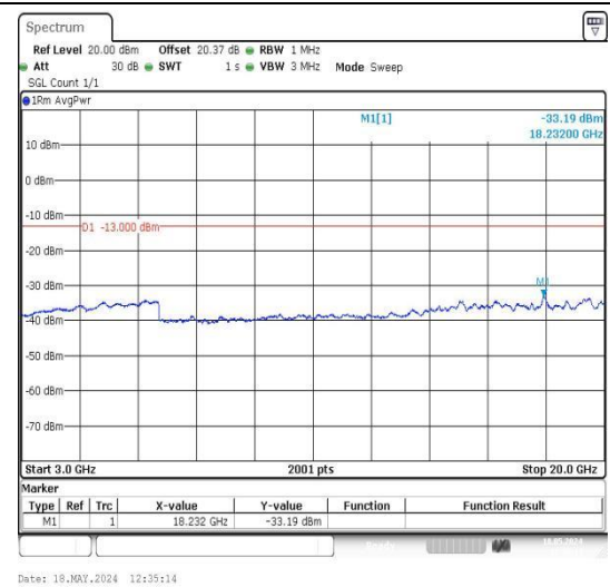
Band25_20MHz_16QAM_26140_1RB#0_3000~20000_3000~20000
