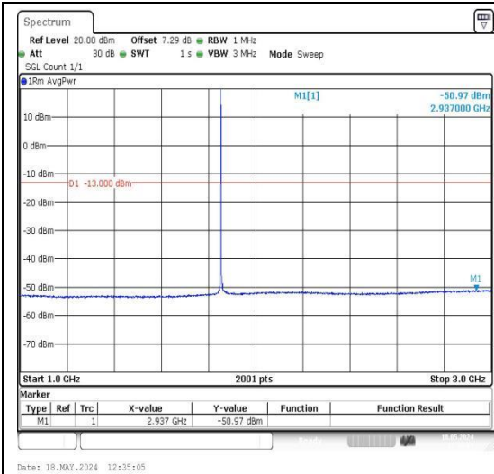
Band25_20MHz_16QAM_26140_1RB#0_1000~3000_1000~3000
