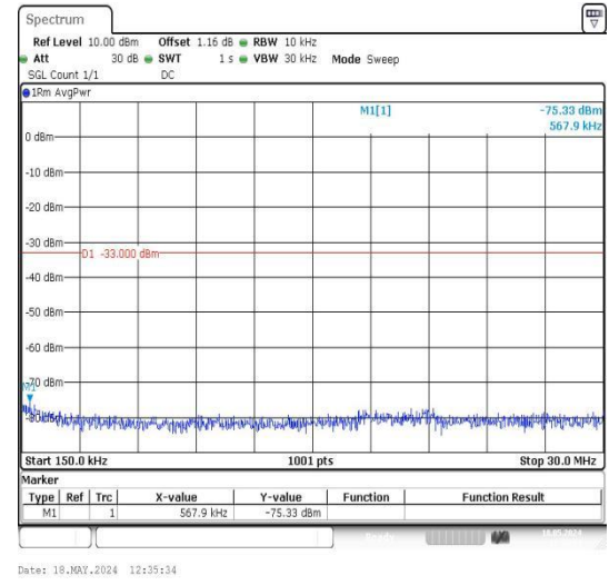
Band25_20MHz_QPSK_26365_1RB#0_0.15~30_0.15~30
