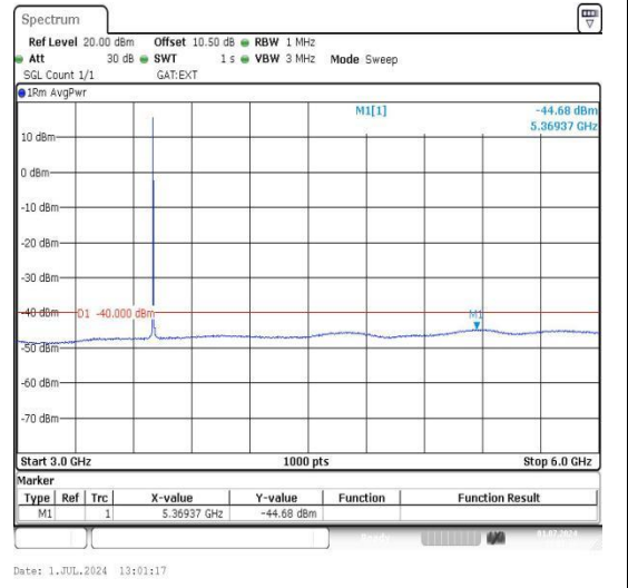
Band43_20MHz_16QAM_44690_1RB#0_3000~60 00_3000~6000
