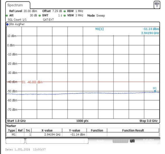
Band43_20MHz_16QAM_44690_1RB#0_1000~3 000_1000~3000
