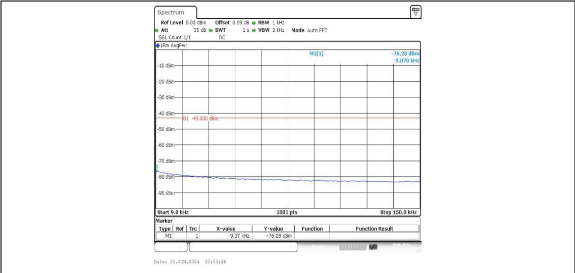
Band4-1312-1-0.009~0.15MHz-PASS
