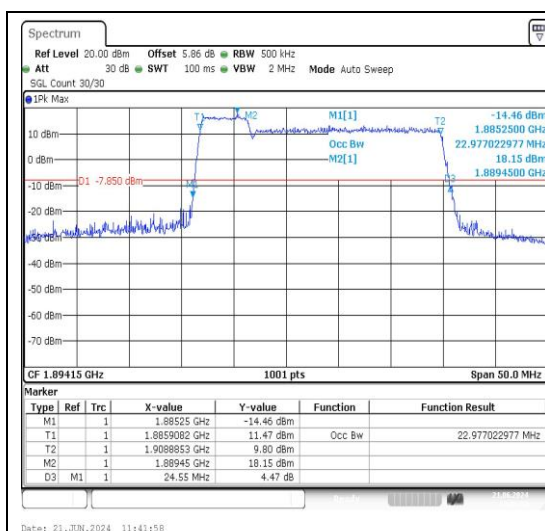
2-2-5MHz-20MHz-QPSK-QPSK-18983-19100-25 RB#0-100RB#0-PASS
