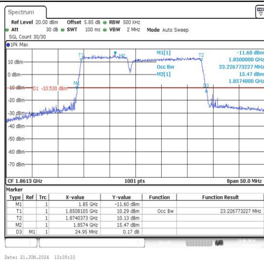
2-2-10MHz-15MHz-16QAM-16QAM-18653-18773-50RB#0-75RB#0-PASS
