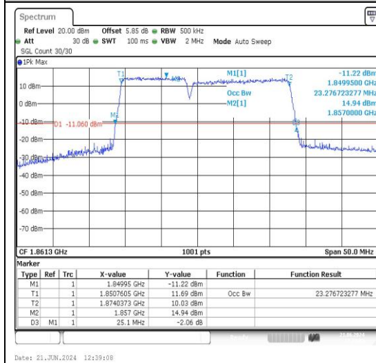
2-2-10MHz-15MHz-QPSK-QPSK-18653-18773-5 0RB#0-75RB#0-PASS
