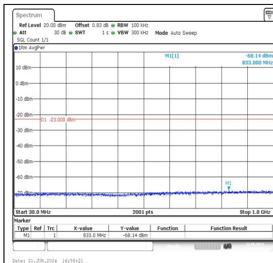
2-2-15MHz-15MHz-QPSK-QPSK-18825-18975-1 RB#74-0RB#0-30~1000MHz-PASS
