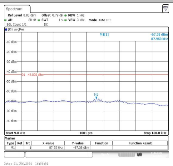
2-2-15MHz-15MHz-16QAM-16QAM-18825-18975- 1RB#74-0RB#0-0.009~0.15MHz-PASS
