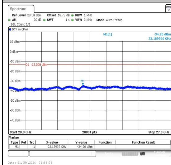
2-2-15MHz-15MHz-QPSK-QPSK-18825-18975-1 RB#74-0RB#0-20000~27000MHz-PASS
