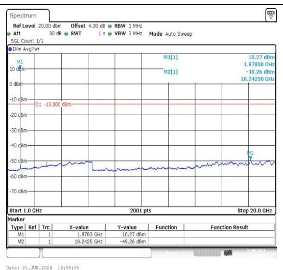
2-2-15MHz-15MHz-QPSK-QPSK-18825-18975-1R B#74-0RB#0-1000~20000MHz-PASS
