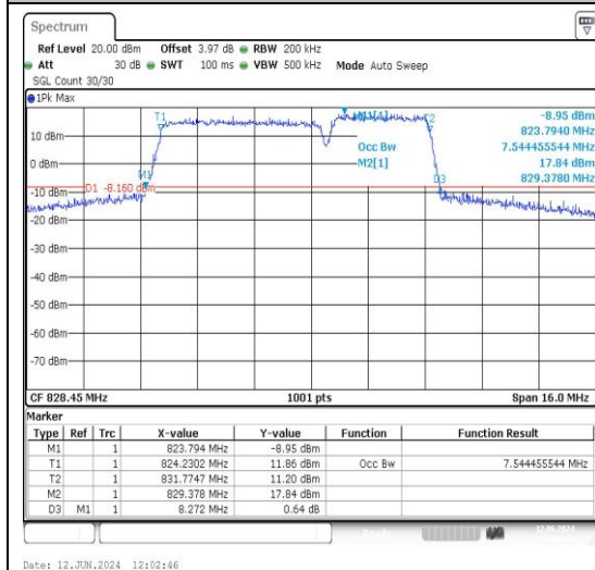
5-5-5MHz-3MHz-QPSK-QPSK-20425-20464-25R B#0-15RB#0-PASS
