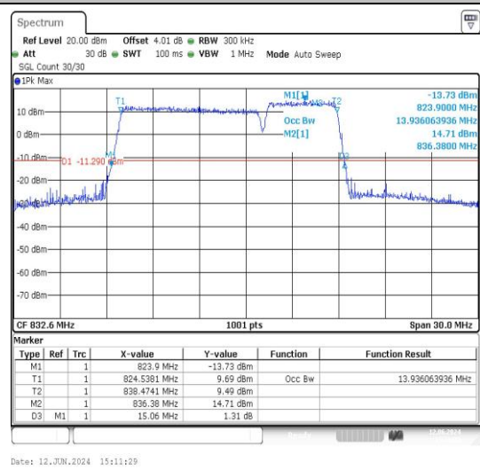
5-5-5MHz-10MHz-16QAM-16QAM-20528-20600-2 5RB#0-50RB#0-PASS
