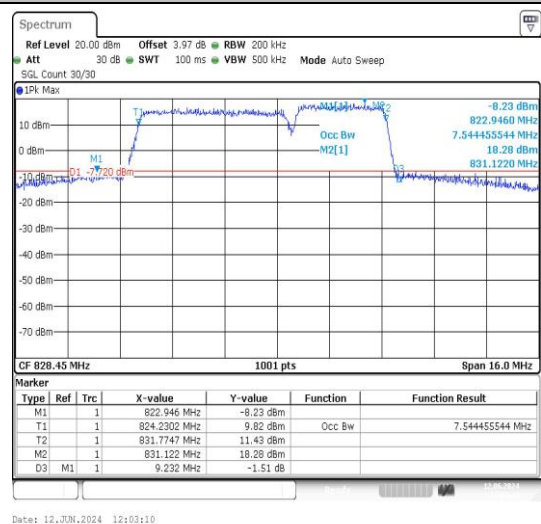
5-5-5MHz-3MHz-16QAM-16QAM-20425-20464-25 RB#0-15RB#0-PASS
