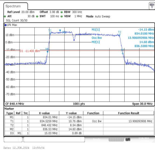
5-5-5MHz-10MHz-16QAM-16QAM-20528-20600-2 5RB#0-50RB#0-PASS
