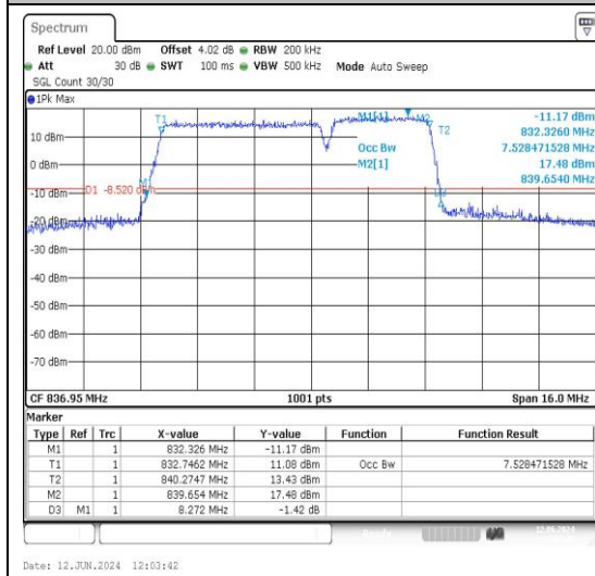
5-5-5MHz-3MHz-QPSK-QPSK-20425-20464-25R B#0-15RB#0-PASS
