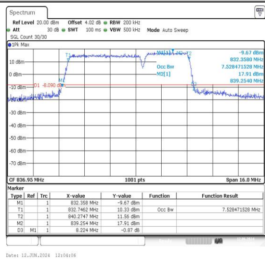
5-5-5MHz-3MHz-16QAM-16QAM-20425-20464-25 RB#0-15RB#0-PASS
