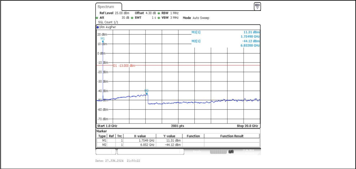
Band4-1513-1000~20000MHz-PASS
