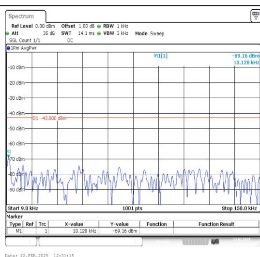
Band25_15MHz_16QAM_26615_1RB#0_0.009~0.15_0.009~0.15
