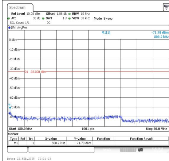
Band25_15MHz_16QAM_26615_1RB#0_0.15~30_0.15~30
