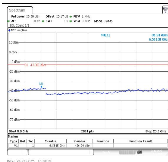
Band25_15MHz_QPSK_26615_1RB#0_3000~20000_3000~20000
