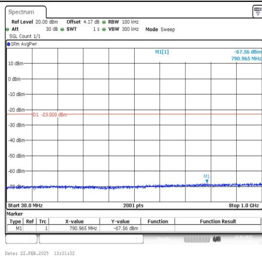
Band25_15MHz_16QAM_26615_1RB#0_30~1000_30~1000
