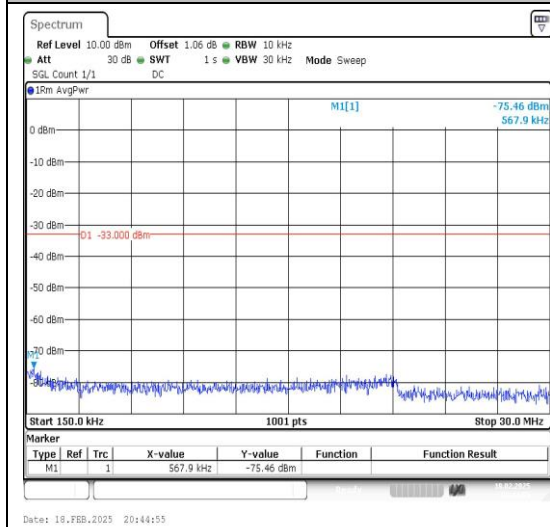
Band4_3MHz_16QAM_19965_1RB#0_0.15~30 0.15~30
