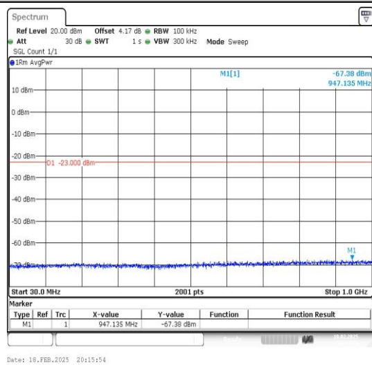
Band4_1.4MHz_16QAM_20393_1RB#0_30~1000_30~1000
