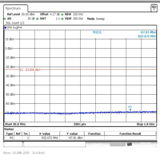
Band4_5MHz_16QAM_19975_1RB#0_30~1000_3 0~1000
