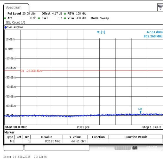
Band4_1.4MHz_16QAM_19957_1RB#0_30~1000_30~1000
