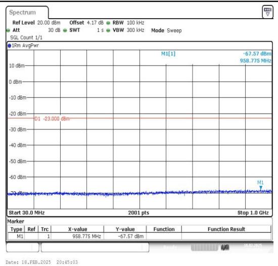
Band4_3MHz_16QAM_19965_1RB#0_30~1000_3 0~1000
