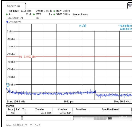
Band4_1.4MHz_16QAM_20393_1RB#0_0.15~30_0.15~30
