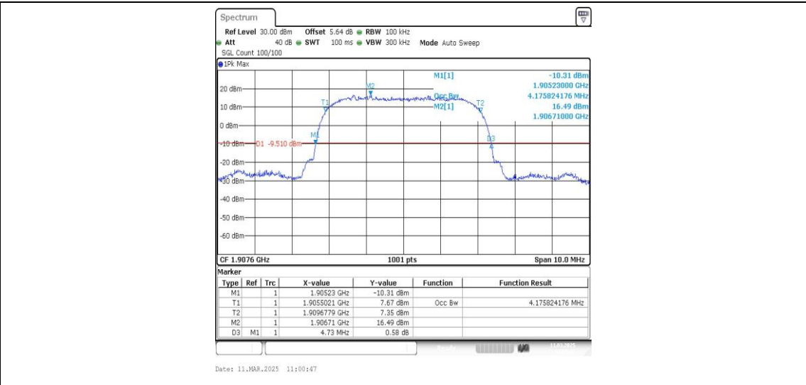
Band2-9538-1-PASS
