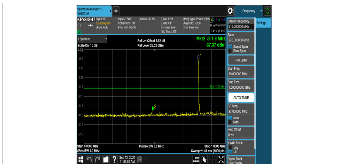
Band26-10MHz-QPSK-26740-1RB#0-Range3:30~1000MHz
