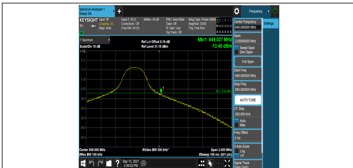
Band26-5MHz-QPSK-27015-1RB#24
