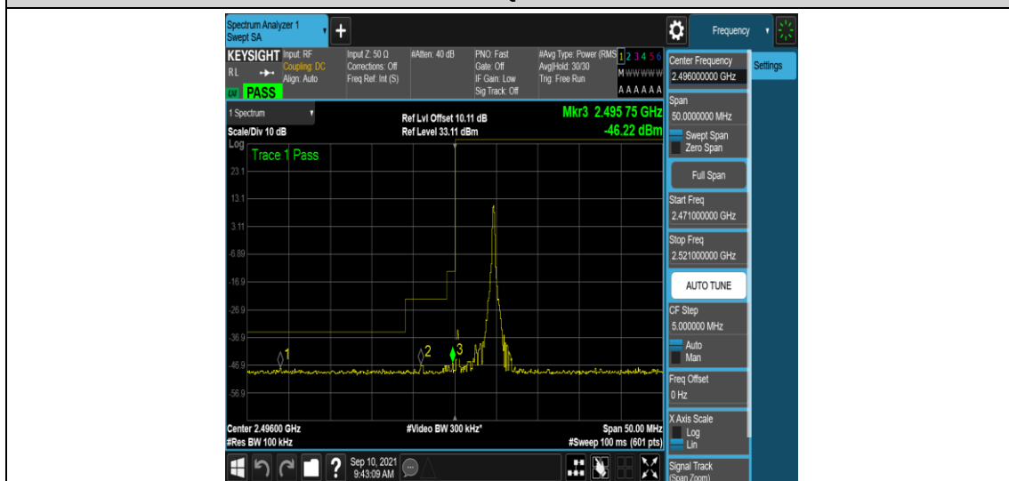
Band41-5MHz-16QAM-39675-1RB#24
