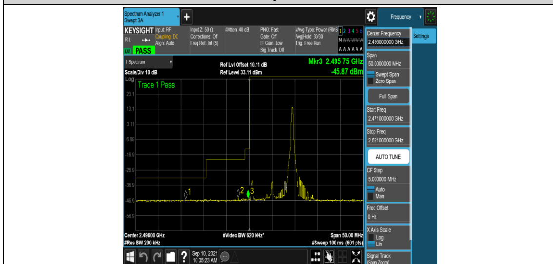
Band41-10MHz-QPSK-39700-1RB#49
