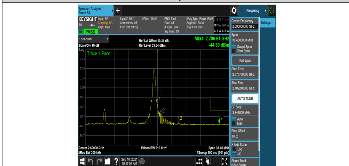
Band41-15MHz-16QAM-41515-1RB#74
