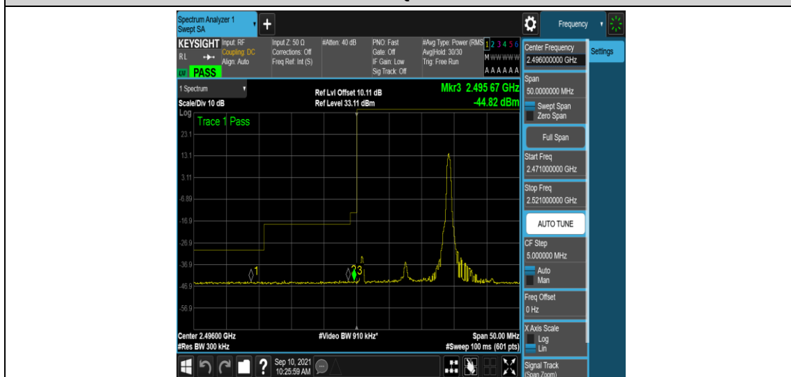
Band41-15MHz-16QAM-39725-1RB#74
