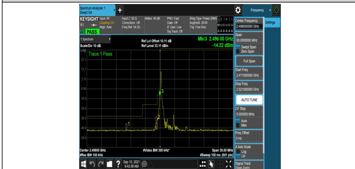
Band41-5MHz-16QAM-39675-1RB#0
