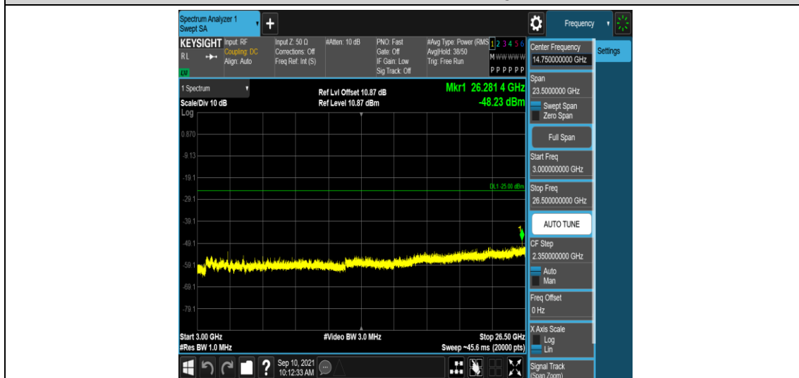
Band41-10MHz-16QAM-40620-1RB#0-Range5:3000~26500MHz
