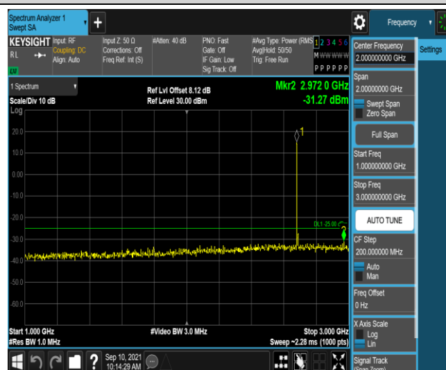
Band41-10MHz-16QAM-41540-1RB#0-Range4:1000~3000MHz
