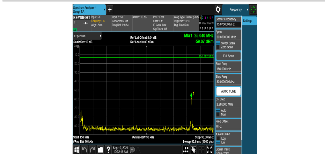
Band41-15MHz-16QAM-40620-1RB#0-Range2:0.15~30MHz
