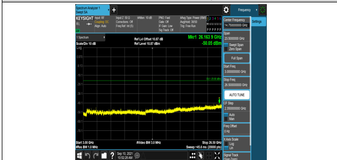
Band41-20MHz-QPSK-40620-1RB#0-Range5:3000~26500MHz
