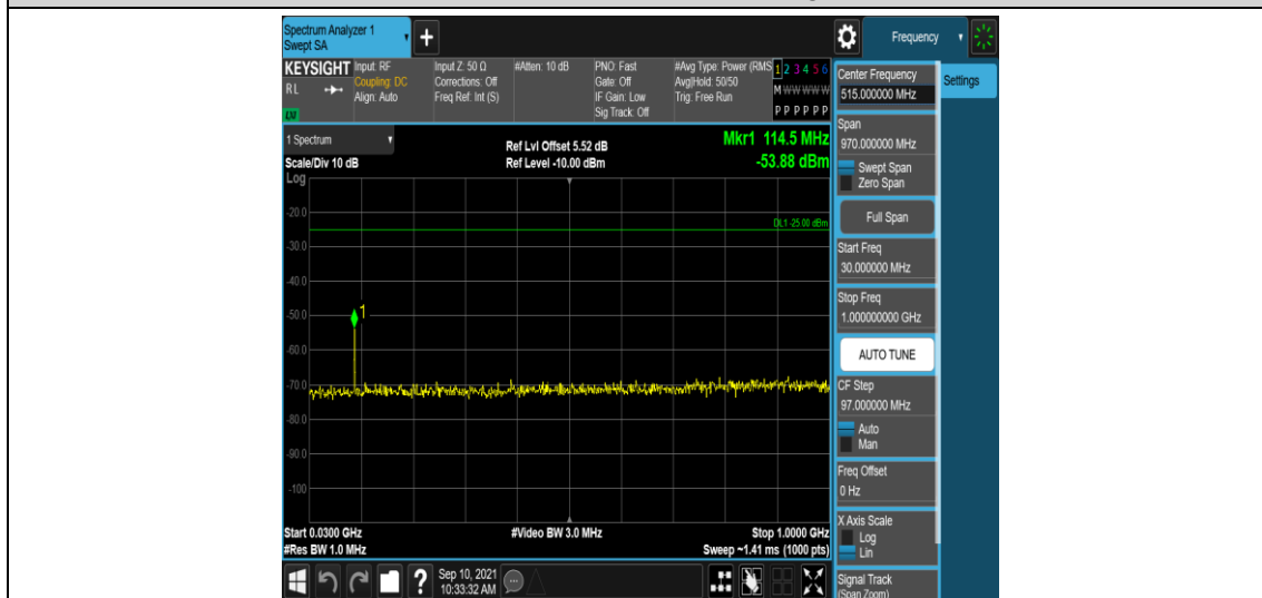
Band41-15MHz-QPSK-41515-1RB#0-Range3:30~1000MHz
