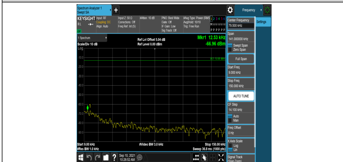
Band41-15MHz-QPSK-39725-1RB#0-Range1:0.009~0.15MHz
