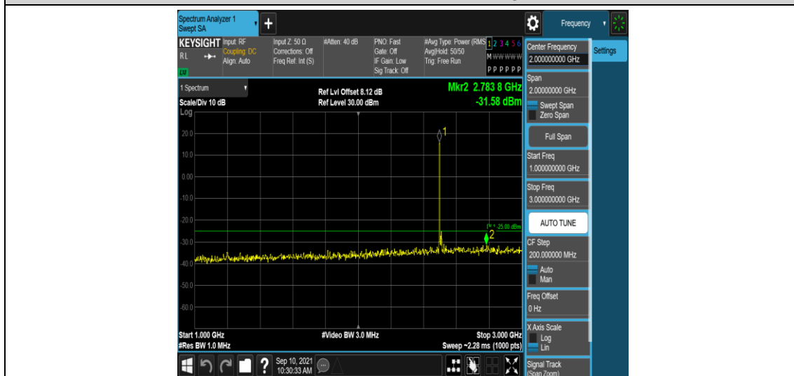
Band41-15MHz-16QAM-39725-1RB#0-Range4:1000~3000MHz
