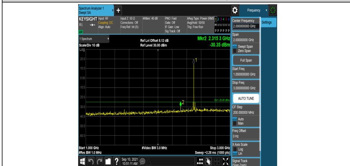
Band41-20MHz-16QAM-39750-1RB#0-Range4:1000~3000MHz
