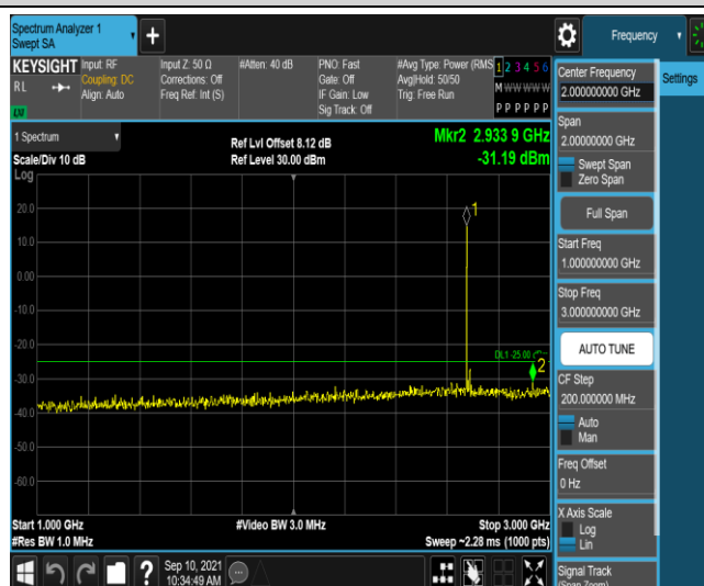
Band41-15MHz-16QAM-41515-1RB#0-Range4:1000~3000MHz
