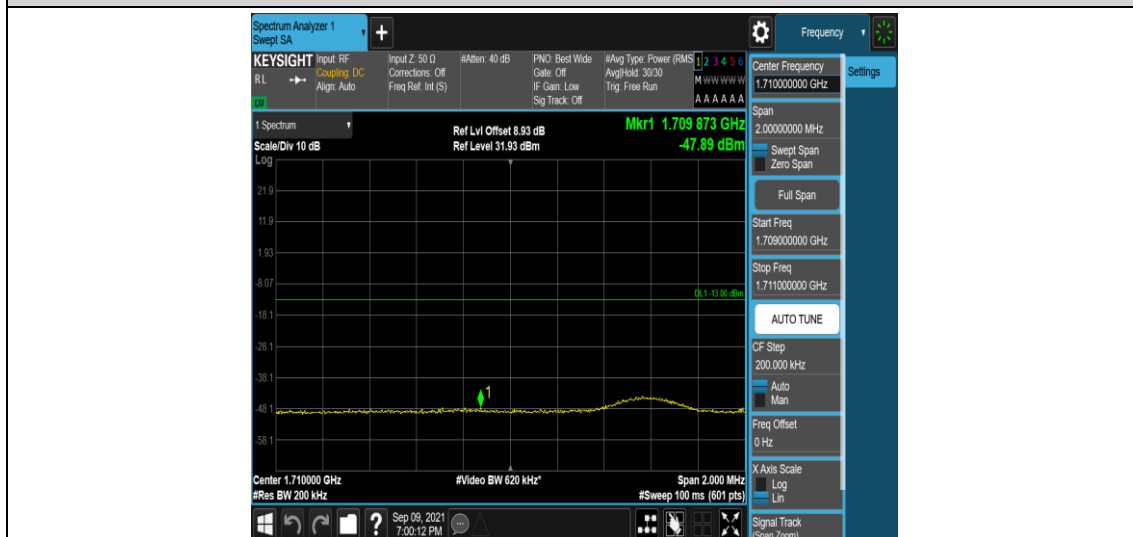
Band66-10MHz-QPSK-132022-1RB#49
