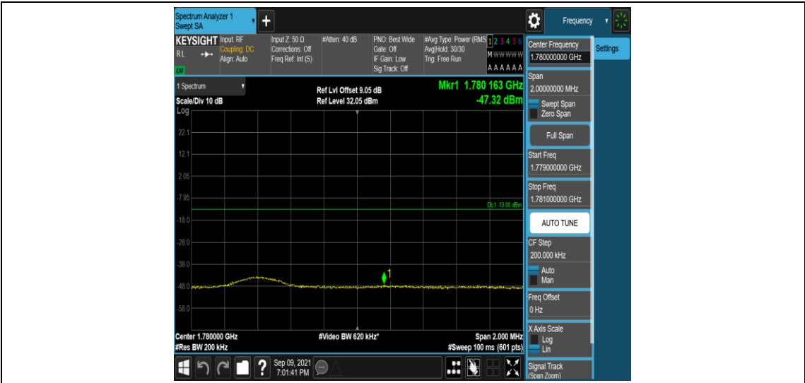
Band66-10MHz-16QAM-132622-1RB#0
