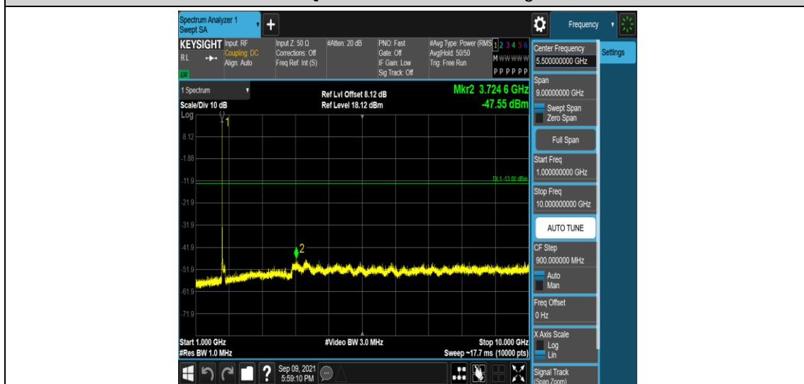
Band66-1.4MHz-16QAM-131979-1RB#0-Range4:1000~10000MHz
