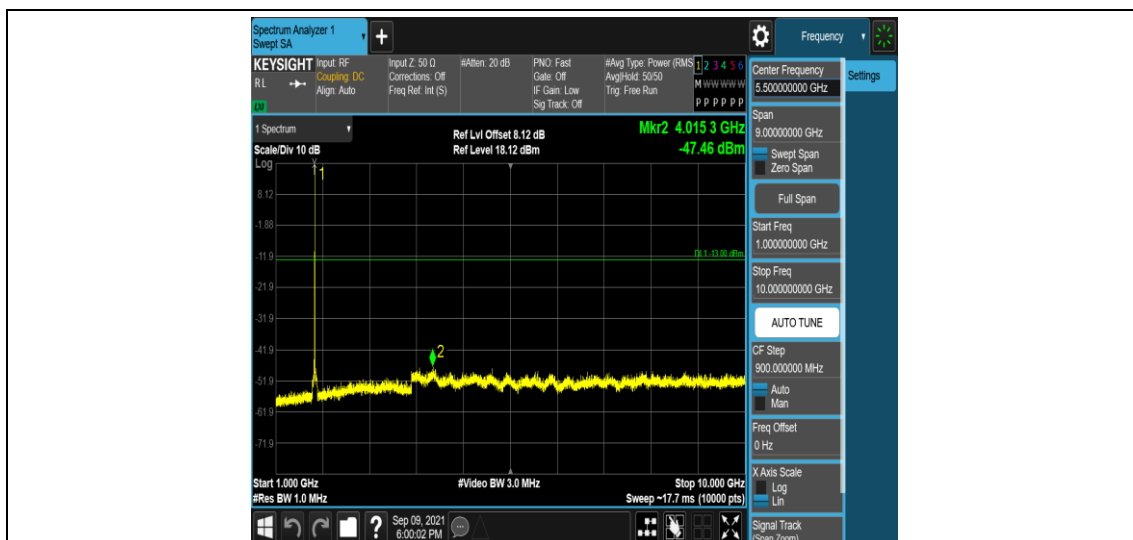
Band66-1.4MHz-QPSK-132322-1RB#0-Range4:1000~10000MHz
