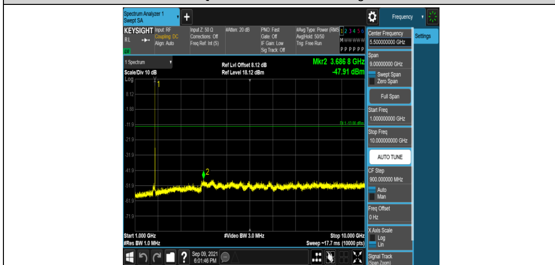
Band66-1.4MHz-QPSK-132665-1RB#0-Range4:1000~10000MHz
