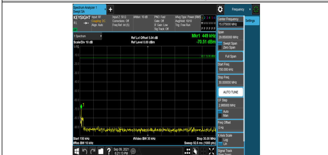
Band66-3MHz-QPSK-132322-1RB#0-Range2:0.15~30MHz
