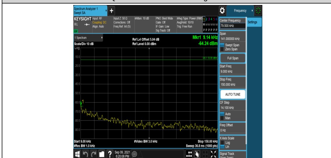
Band66-3MHz-16QAM-131987-1RB#0-Range1:0.009~0.15MHz
