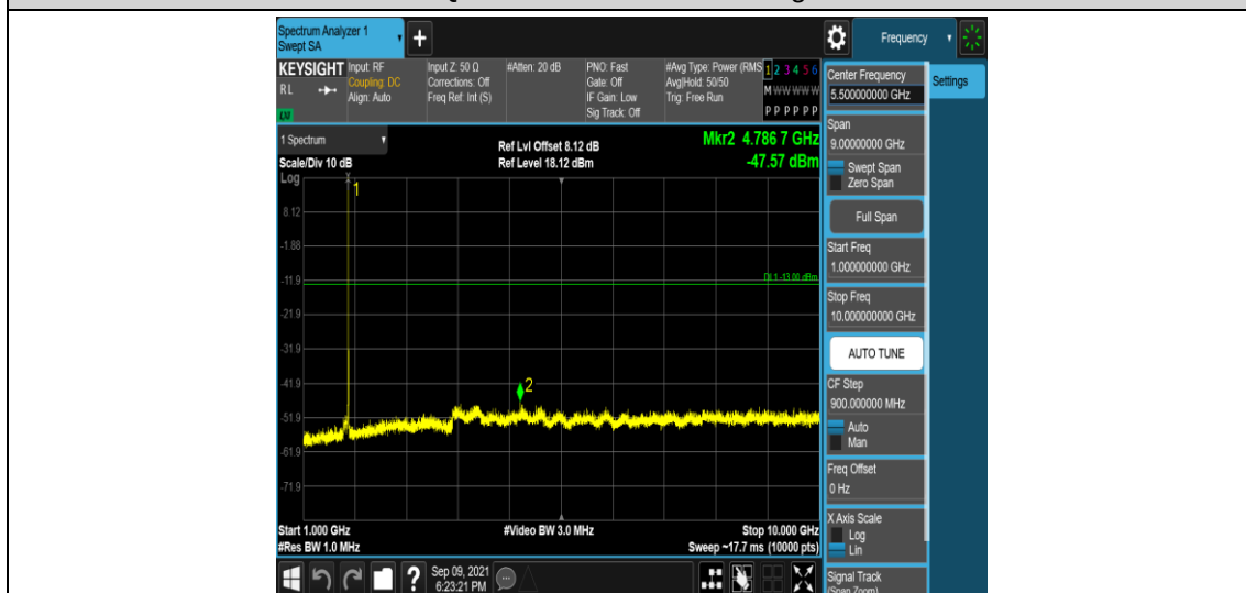
Band66-3MHz-QPSK-132657-1RB#0-Range4:1000~10000MHz
