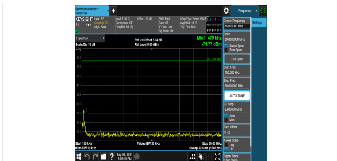
Band66-1.4MHz-16QAM-131979-1RB#0-Range2:0.15~30MHz
