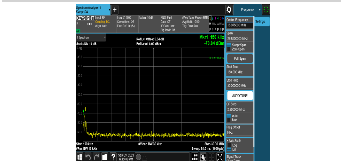
Band66-5MHz-QPSK-132322-1RB#0-Range2:0.15~30MHz
