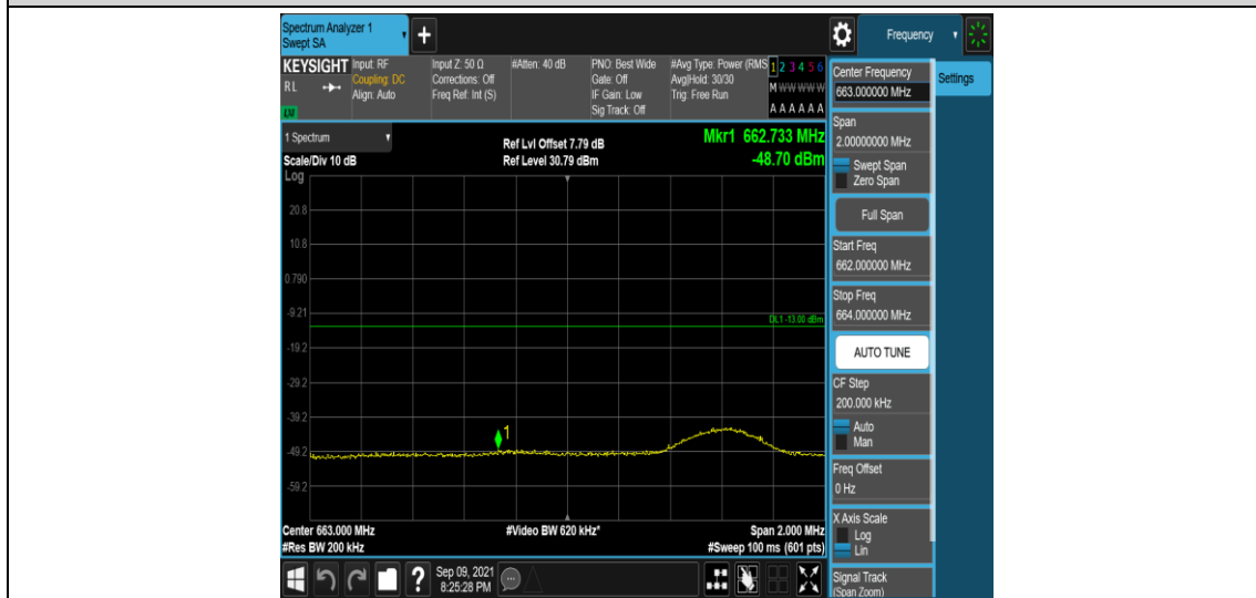
Band71-10MHz-16QAM-133172-1RB#49
