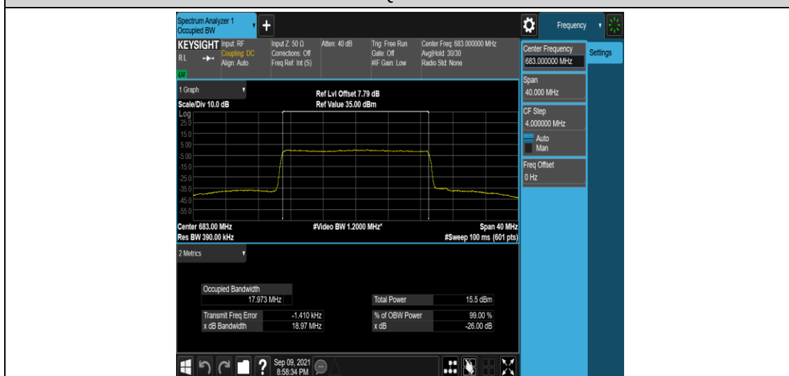
Band71-20MHz-16QAM-133322-100RB#0
